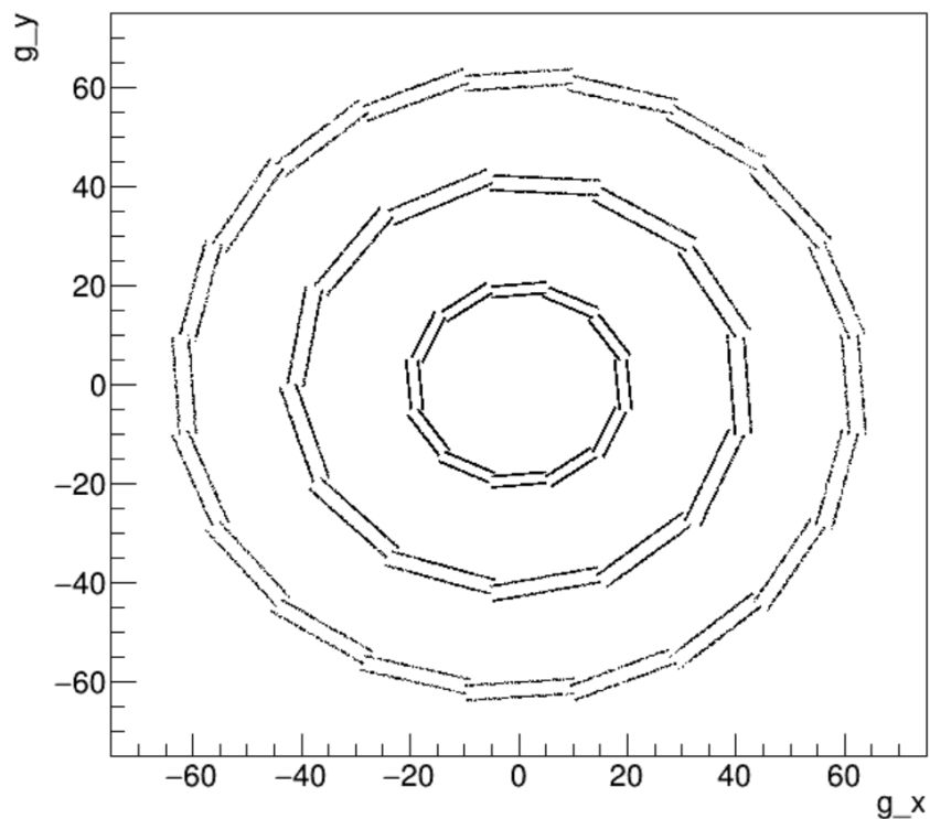
X-Y view : Vertex fatras-hit
