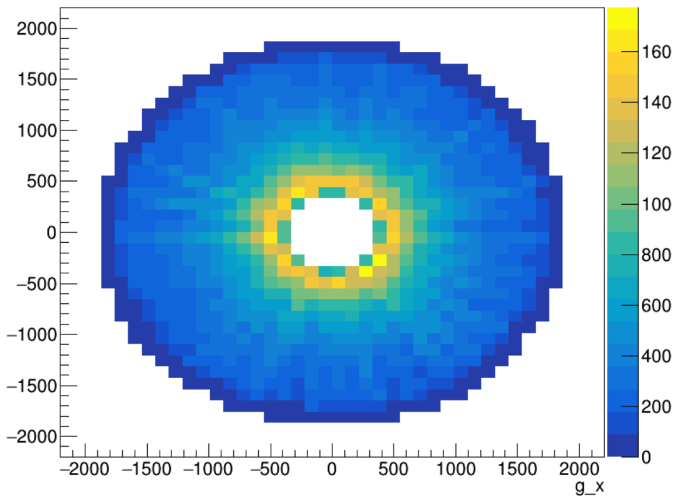
X-Y view : 100 layer TPC fatras-hit
