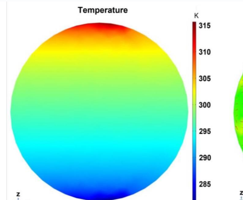
Fig. 3: Fluid temperature (left) and flow velocity (right) distribution in the spherical detector
