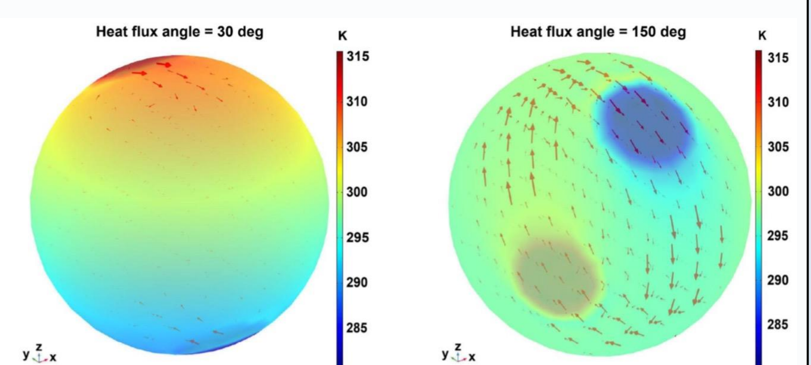
Fig.9 The distributions of temperature and liquid flow in the sphere when the CFD simulation reaches stable, for the two cases when the heat flux area deviates from the Z-axis by 30 degrees (left) and by 150 degrees (right), respectively
