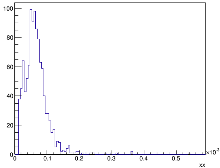
TrackerHitPlane
