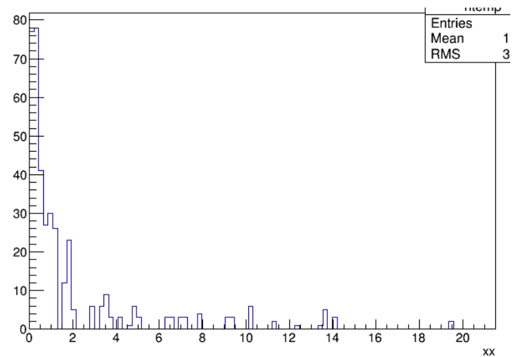
ReconstructedParticle
