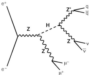
Fig. 1 Example Feynman diagram of the signal process which is characterized by the presence of a pair of muons, jets and neutrinos. In this example, the initial Z boson associated with the Higgs production is decaying into muons whereas cyclic permutation of the decay products from 3 Z bosons is considered in the analysis.
