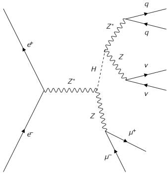
Fig. 1 Example feyman diagram of the signal process which is characterized by the presence of a pair of muons, jets and neutrinos. In this example, the initial Z boson associated with the Higgs production is decaying into muons whereas cyclic permutation of the decay products from 3 Z bosons is considered in the analysis.
