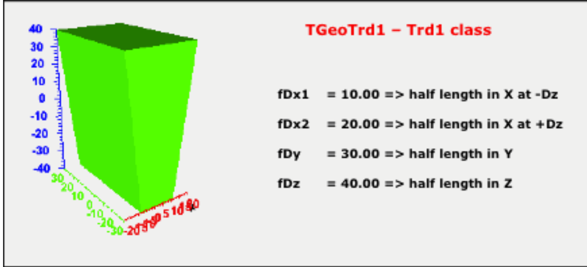
Figure 1.6: TGeoTrd1 class
