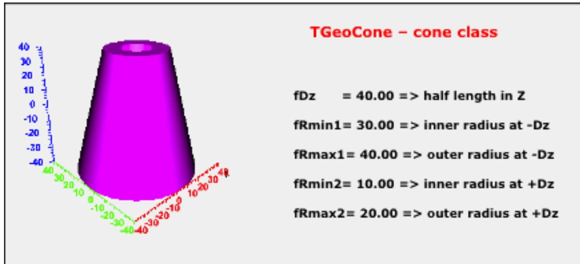
Figure 1.16: TGeoCone Class
