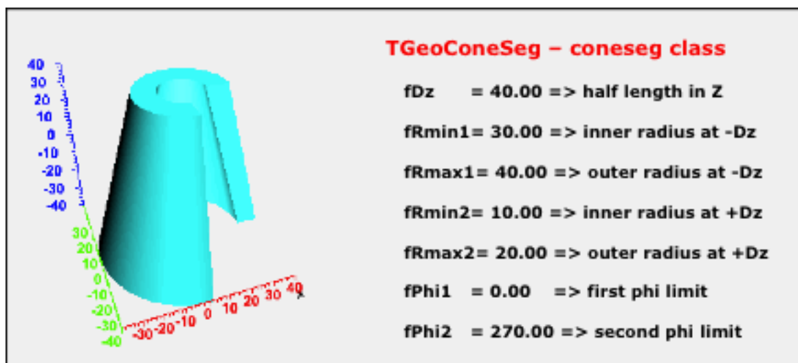
Figure 1.17: TGeoConeSeg Class
