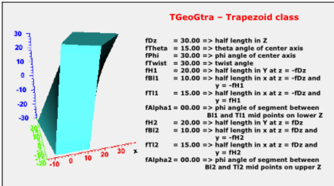
Figure 1.9: TGeoGtra class
