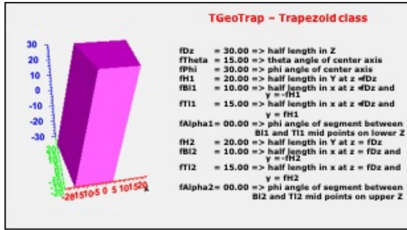
Figure 1.8: TGeoTrap Class
