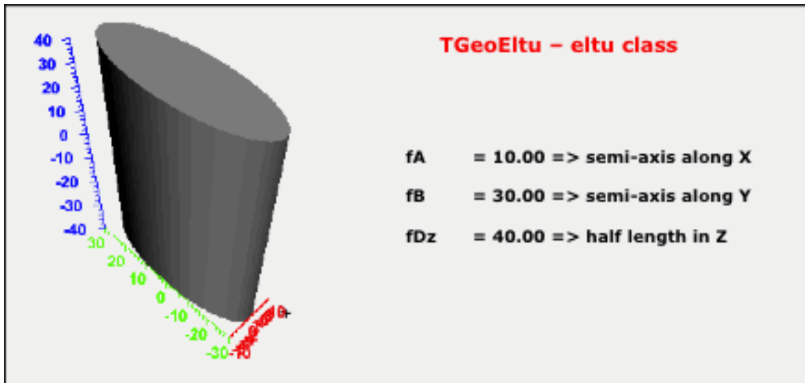
Figure 1.14: TGeoEltu Class
