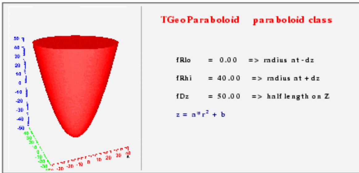
Figure 1.20: TGeoParaboloid Class
