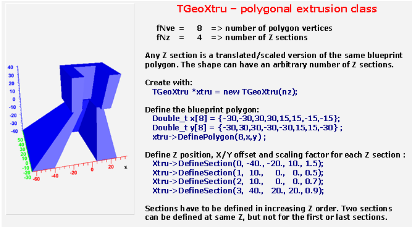
Figure 1.23: TGeoXtru Class
