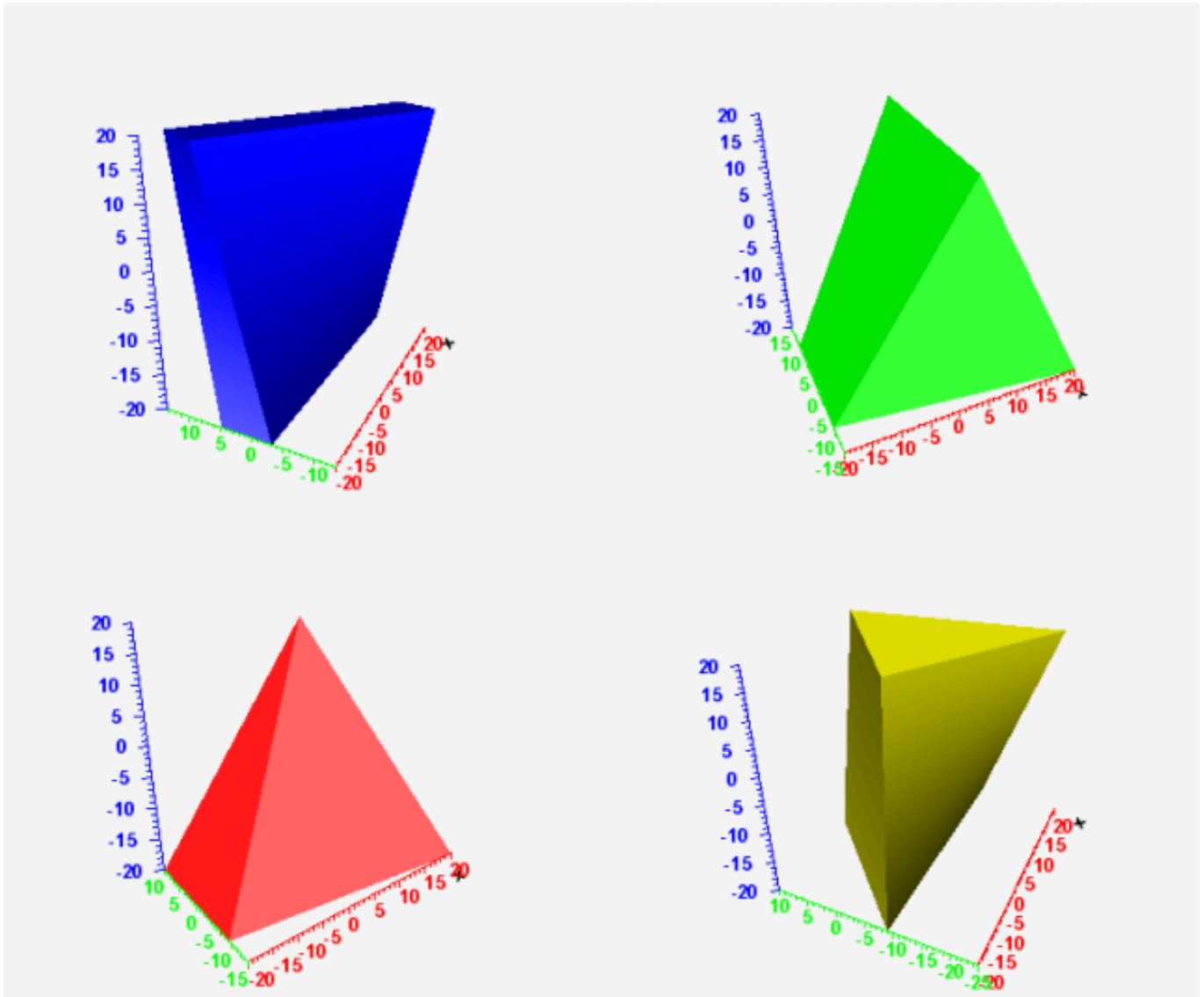
Figure 1.10: TGeoArb8 class
