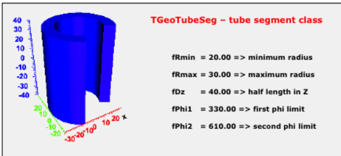
Figure 1.12: TGeoTubeSeg Class
