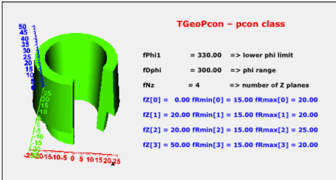
Figure 1.21: TGeoPcon Class
