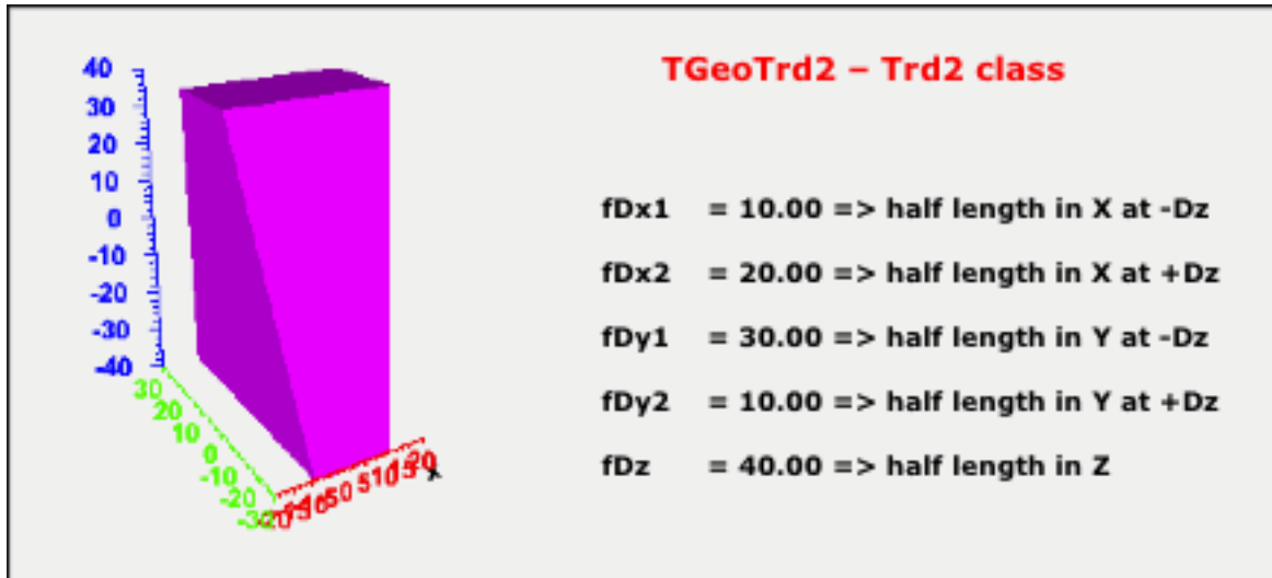
Figure 1.7: TGeoTrd2 class
