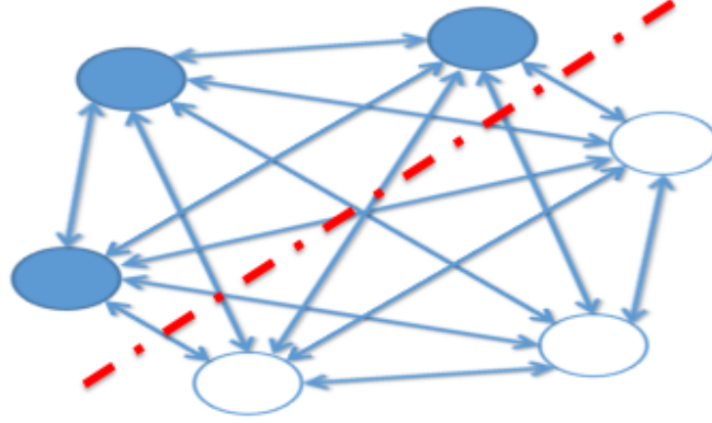
Figure 10: Illustration of Boltzmann Machine. With the introduction of hidden units (shaded nodes), the model conceptually splits into two parts: visible units and hidden units. The red dashed line is used to highlight the conceptual separation.
