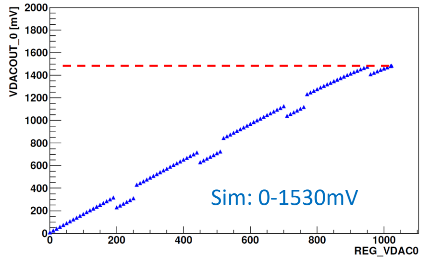
VDAC transfer curve
