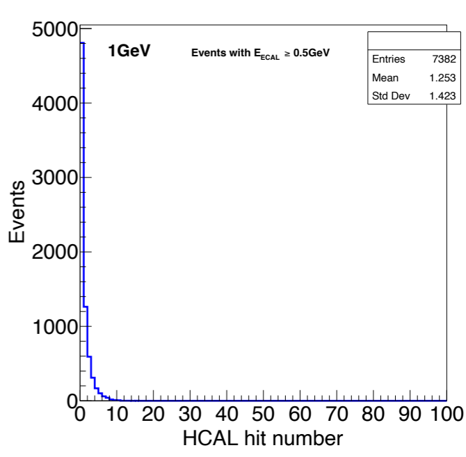
Events with E_{ECAL} > \text{threshold}
