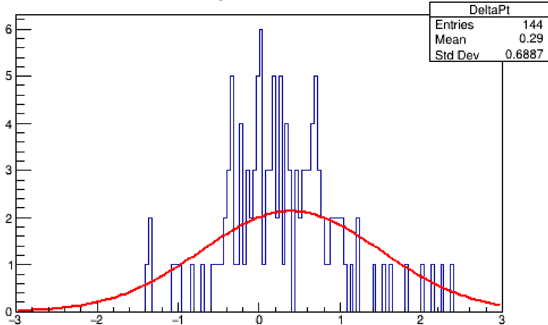
histogram of deltaPt
