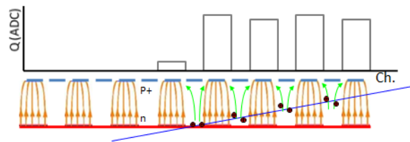
Figure 2: Beam test with silicon wafer is illustrated for the incident of a low angle charged particle. The impact position and angle is measured by the collected ionization charges by readout strips or pads on the edge where the particle enter and exit the wafer.
