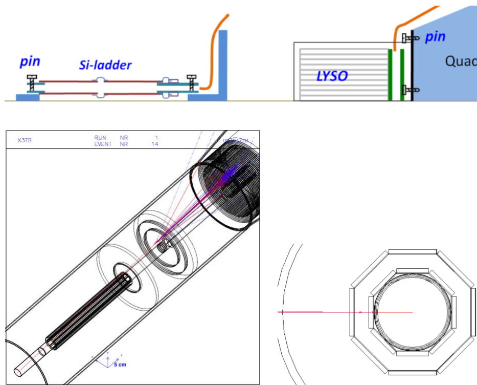
Figure 1: The top drawing illustrates the LumiCal detector design with silicon wafers and LYSO crystal calorimeter. The event display below is shown for a 50 GeV electron in GEANT simulation with the beam-pipe of 1 mm thick Al tube, flange layers at z=520 mm and z=700 mm. The LumiCal Si-wafers include two octagon rings at z=150-520 mm, disks of circular wafers on beam pipe flanges, and a Si-W calorimeter with front face at z=1000 mm.
