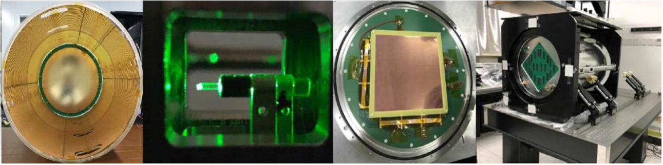
Fig. 2 TPC prototype integrated with 266nm UV calibration system
