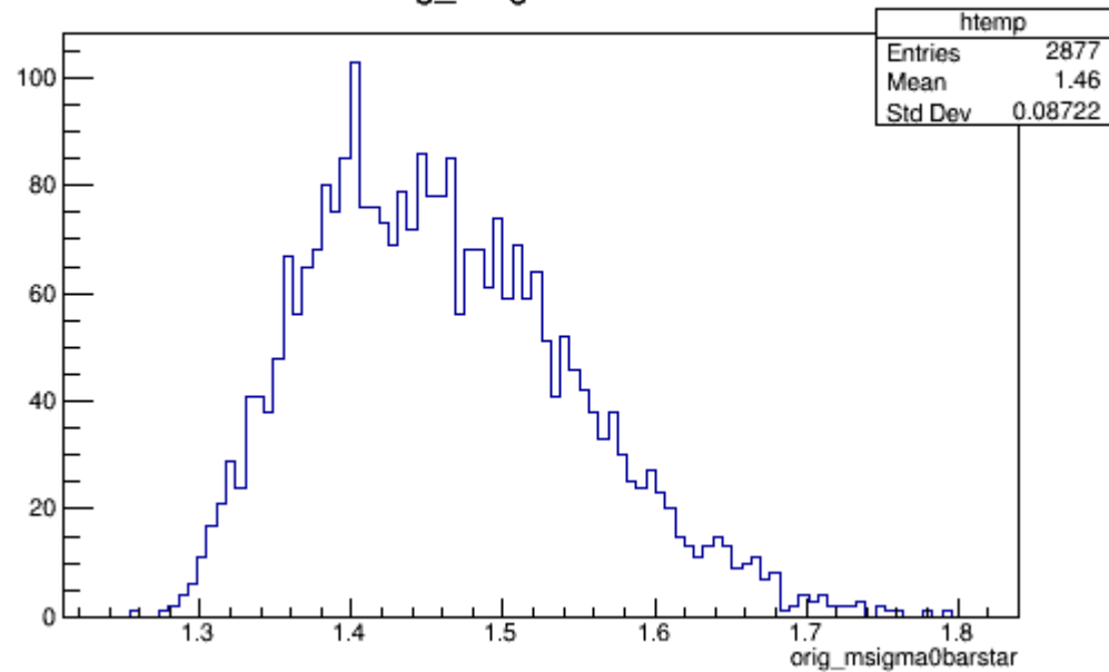
orig_msigma0barstar
