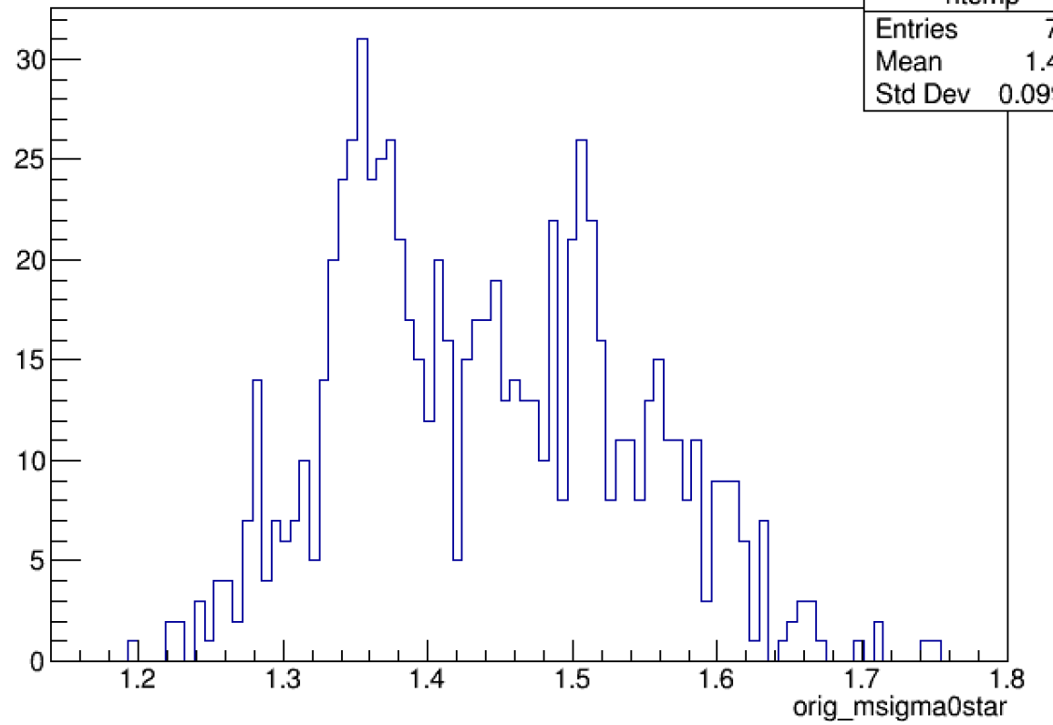
orig_msigma0star
