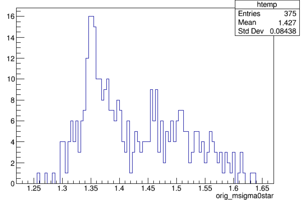
orig_msigma0star {iDcyTr == 0}
