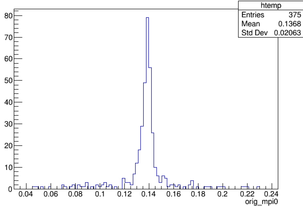
orig_mpi0 {iDcyTr == 0}
