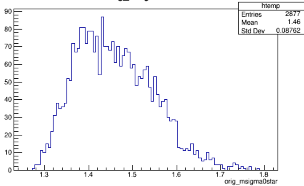
orig_msigma0star
