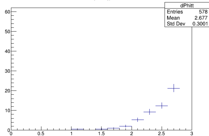
dPhitt_low
