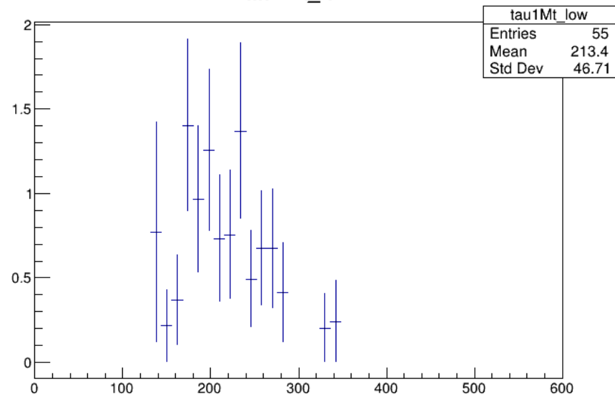
tau1Mt_low
