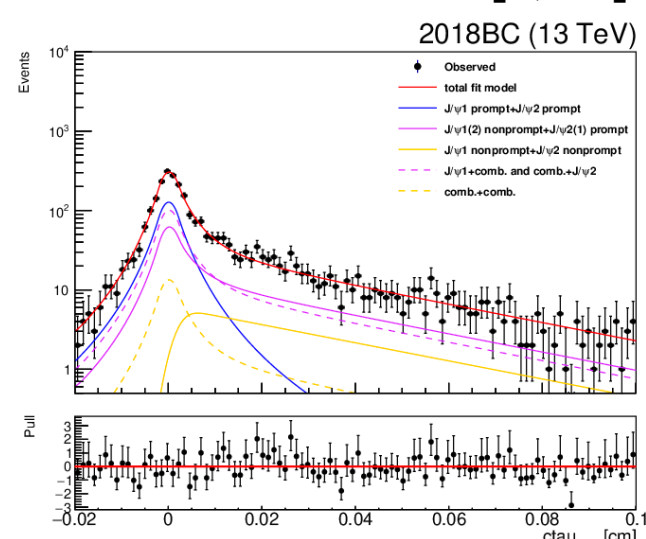
Four muon mass [5, 10]
