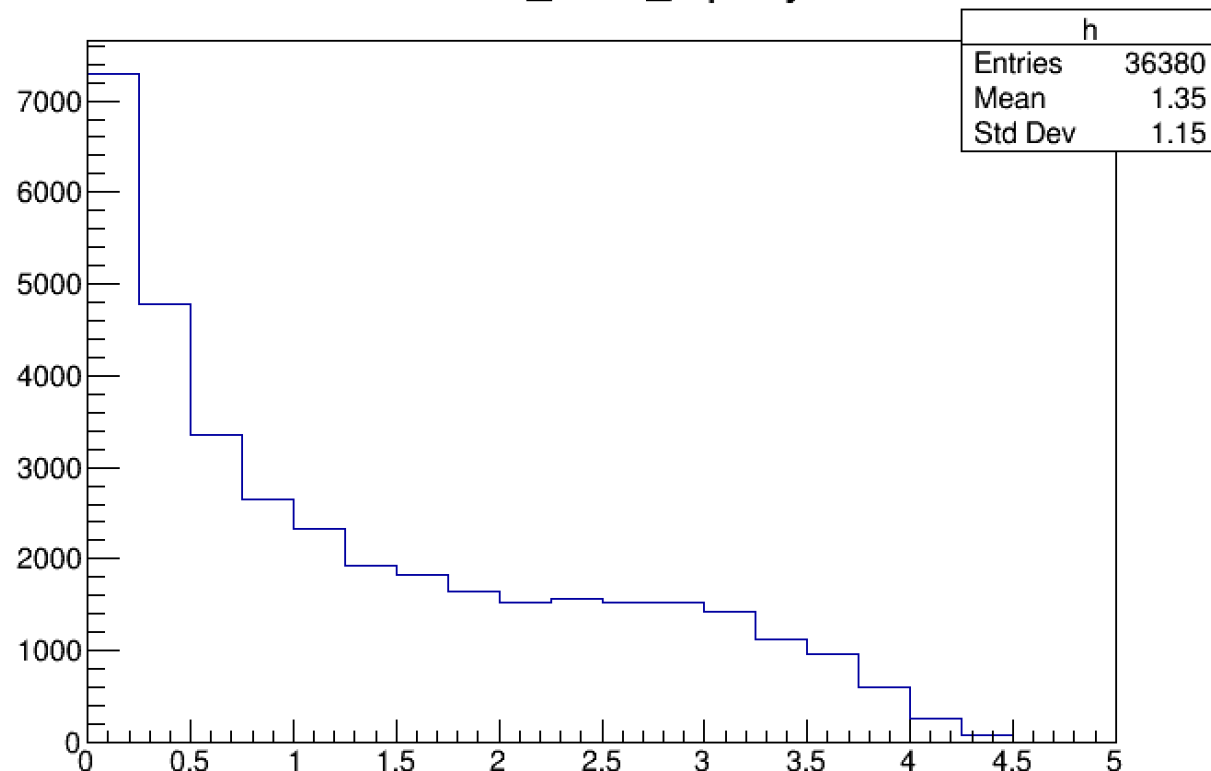
fourMu_Delta_rapidity
