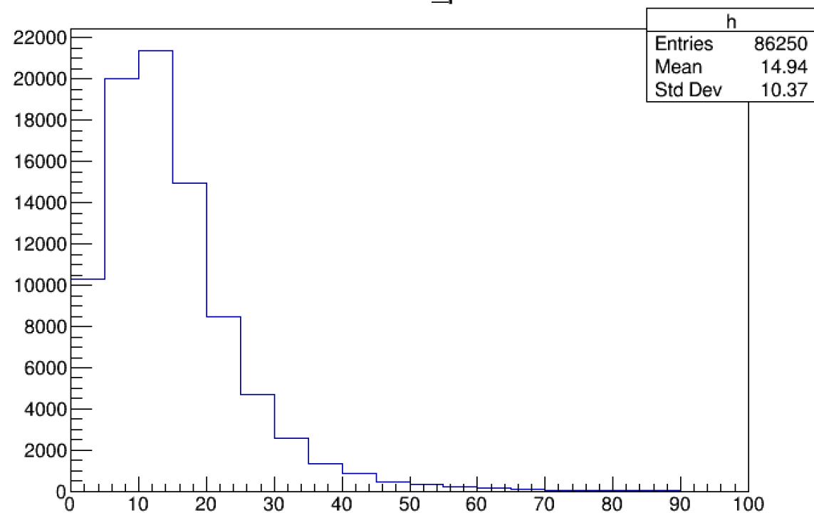
fourMu_pt
