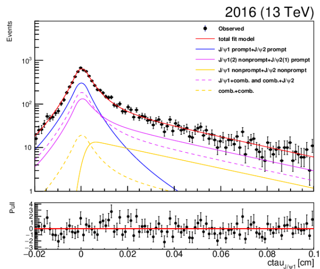
Four muon mass [5, 10]
