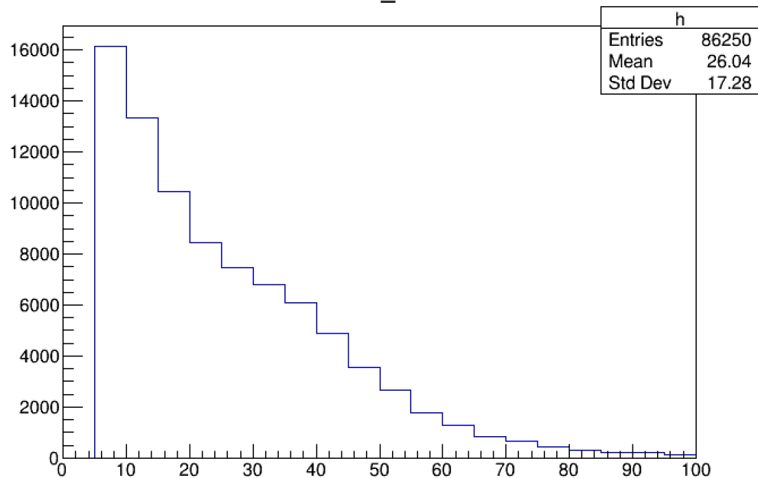
fourMu_mass
