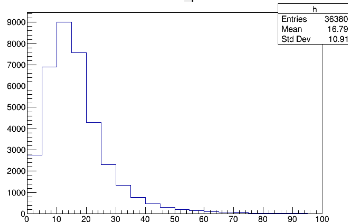
fourMu_pt
