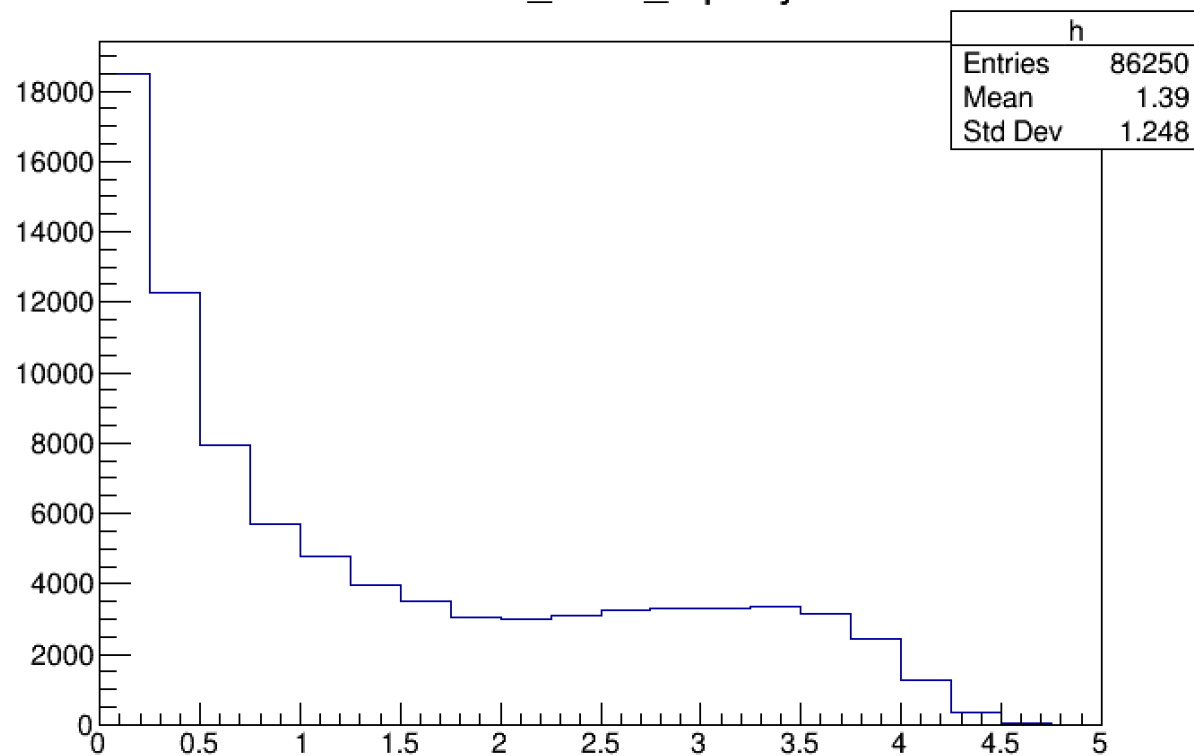
fourMu_Delta_rapidity
