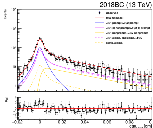
Four muon mass [0, 10]
