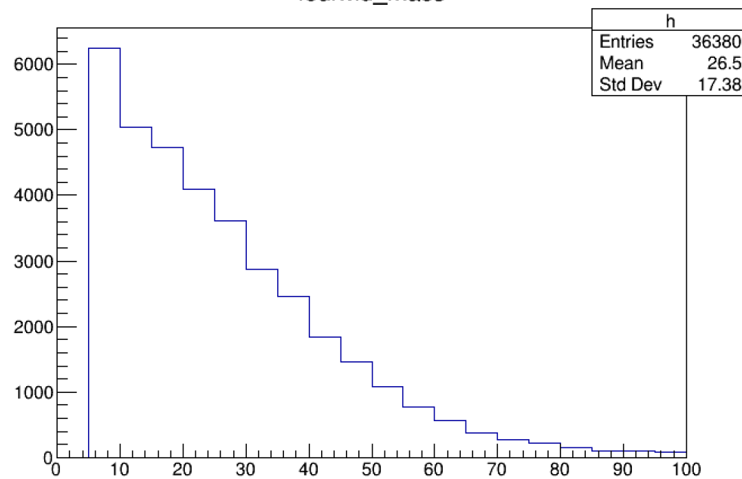
fourMu_mass
