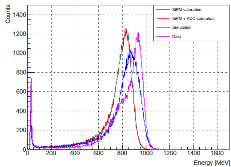
50 GeV
