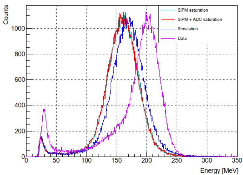
10 GeV
