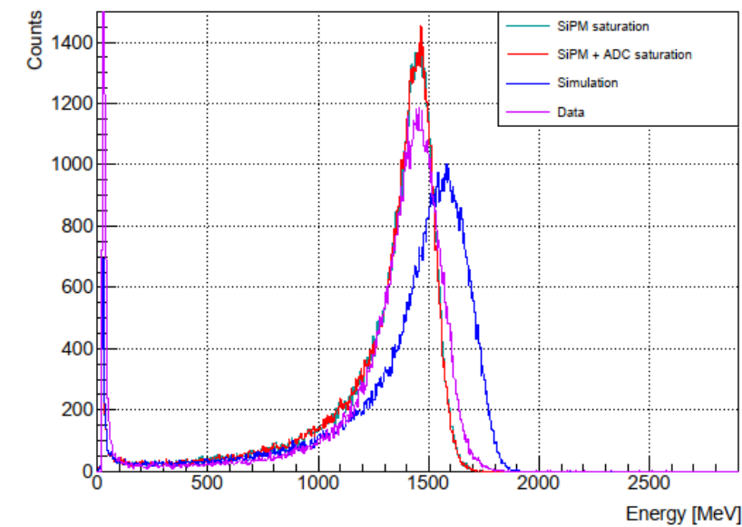
90 GeV
