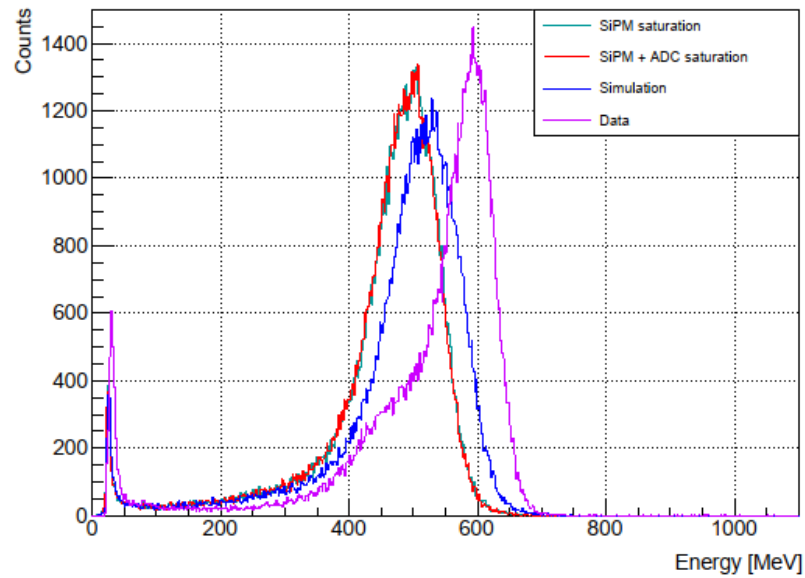
30 GeV
