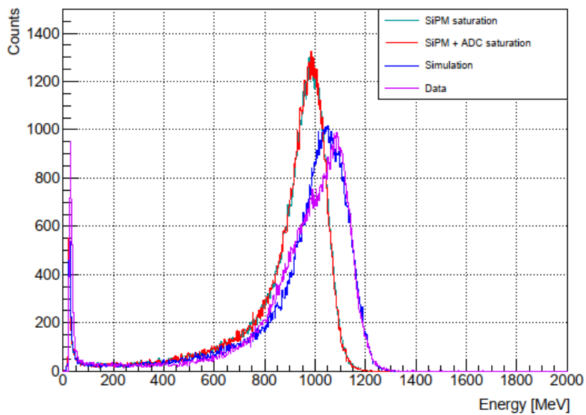
60 GeV
