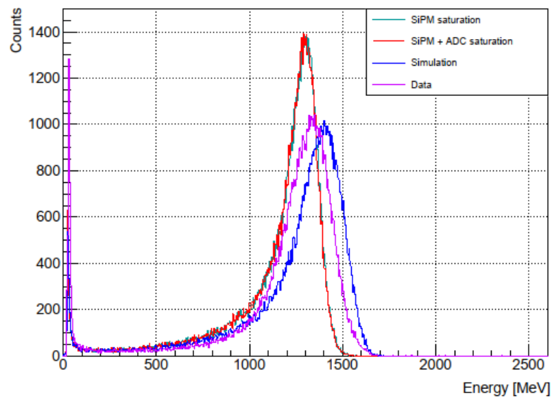
80 GeV
