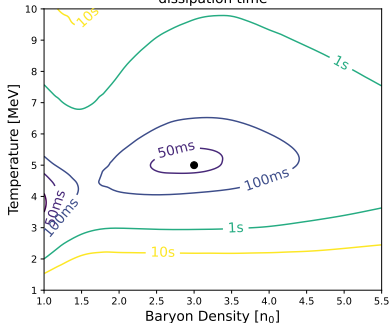
QMC-RMF3 equation of state
