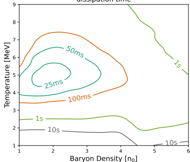
IUF equation of state
