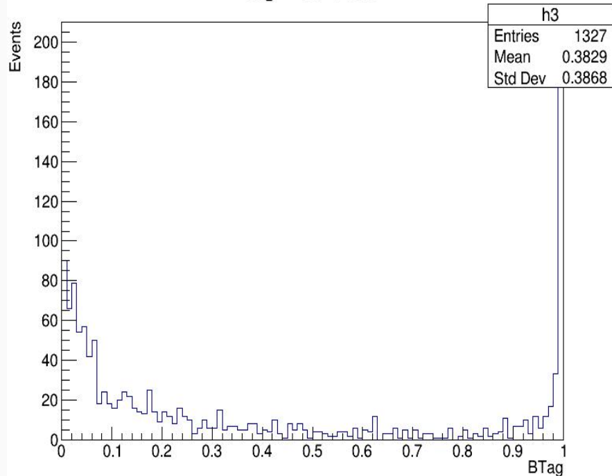
Btag Distribution
