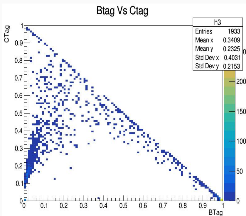
P2 (other-jets)
