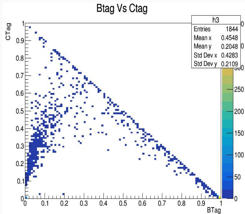
P1 (other-jets)
