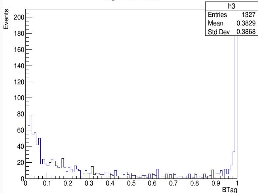
Btag Distribution
