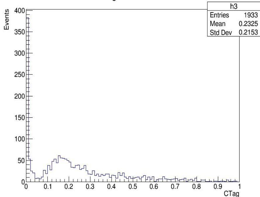
Ctag Distribution
