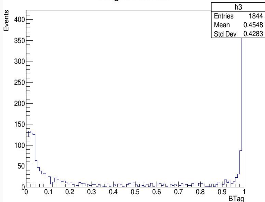
Btag Distribution
