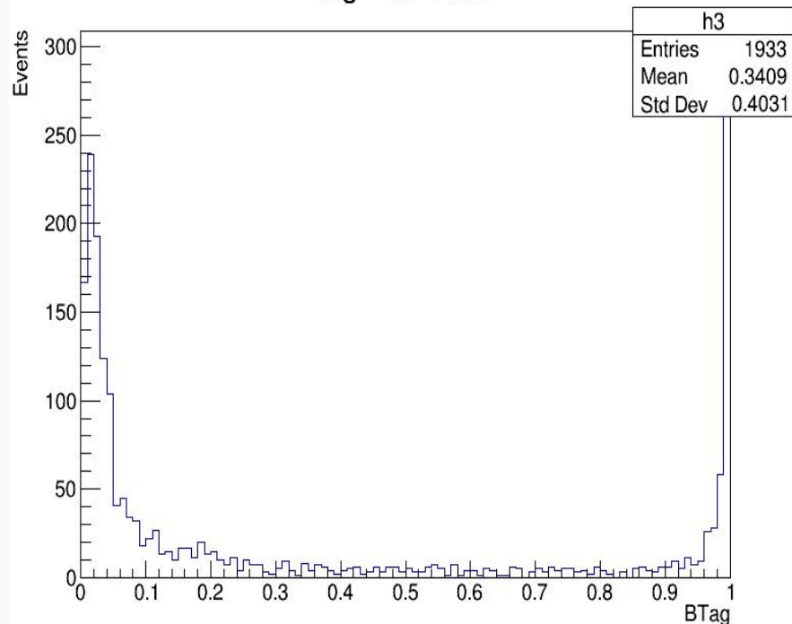
Btag Distribution
