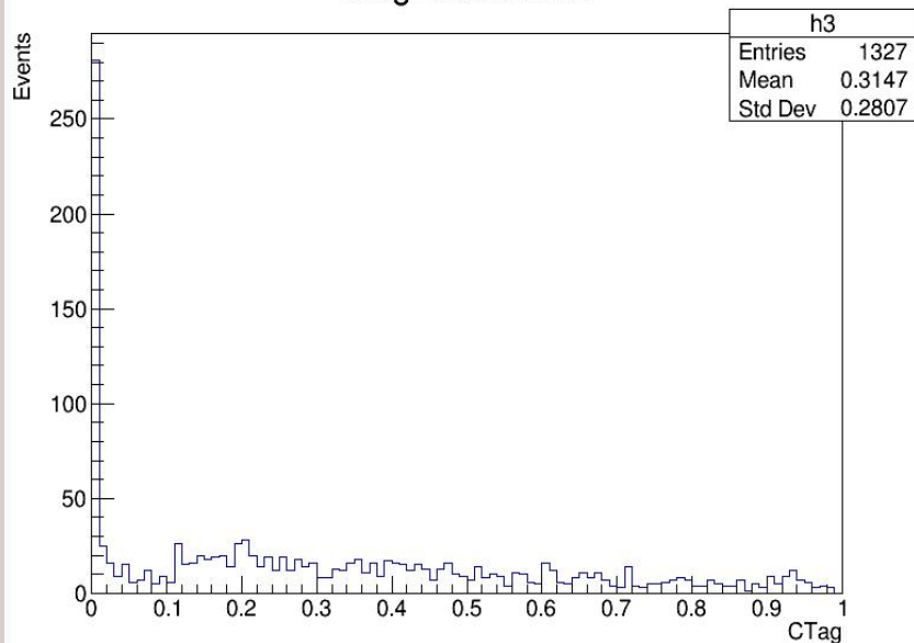
Ctag Distribution
