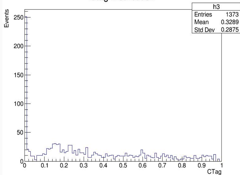
Ctag Distribution
