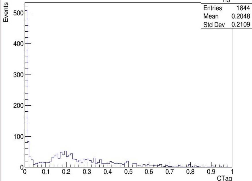
Ctag Distribution
