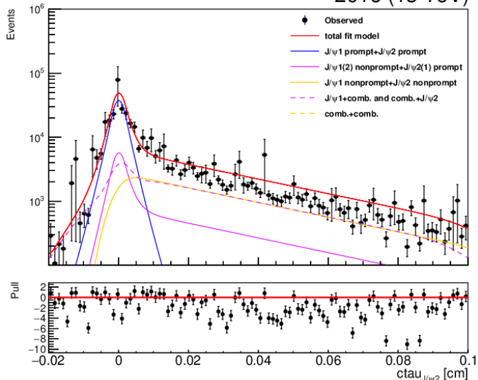
2016 (13 TeV)
