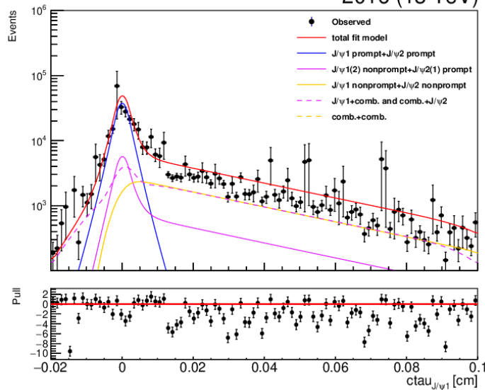
2016 (13 TeV)
