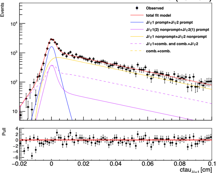
2016 (13 TeV)
