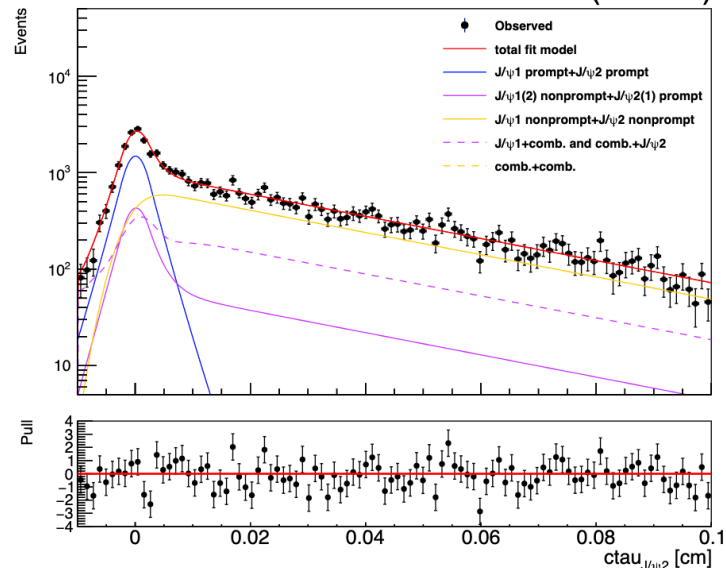
2016 (13 TeV)
