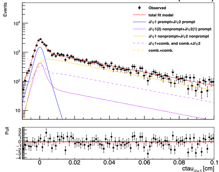
2016 (13 TeV)
