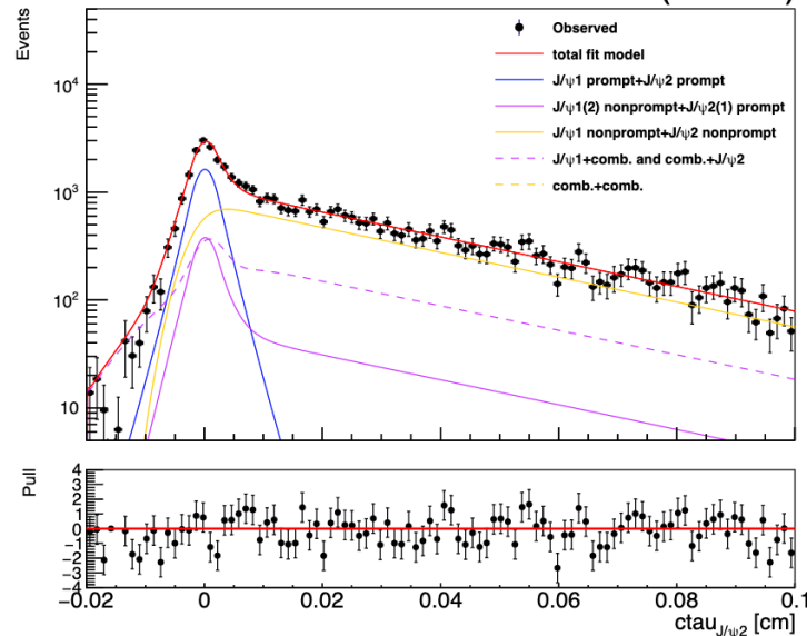
2016 (13 TeV)
