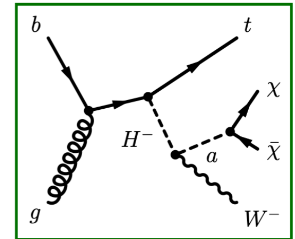
E_T^{\text{miss}} + tW
