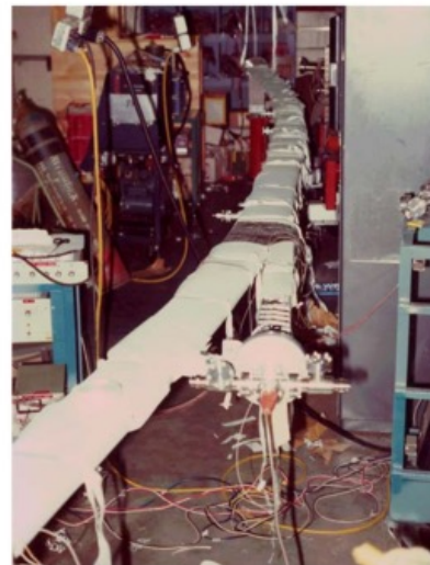
Figure 24. SPEAR bending magnet vacuum chamber with the 1st port to extract synchrotron radiation for experiments (Herman Winick collection).
