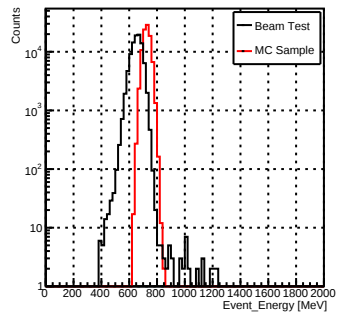
Event_Energy_e-_40GeV
