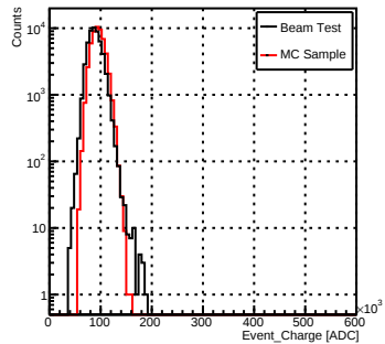
HighGain_e-_50GeV
