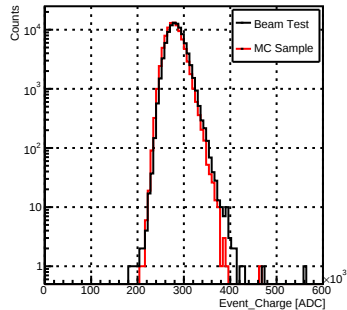
HighGain_e-_70GeV
