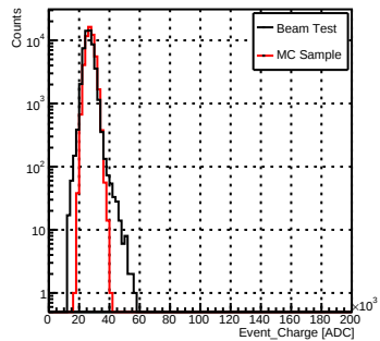
LowGain_e-_50GeV
