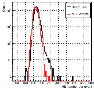
NHit_e-_60GeV
