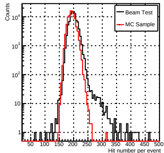
NHit_e-_80GeV
