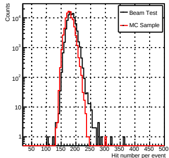
NHit_e-_70GeV
