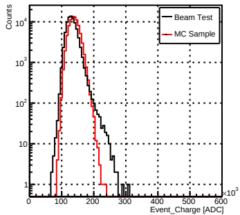
HighGain_e-_60GeV
