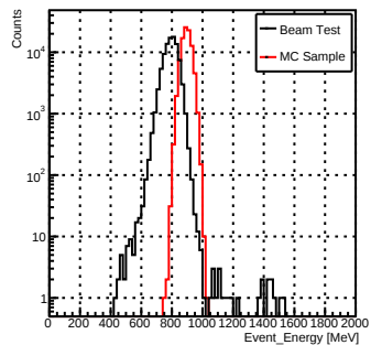
Event_Energy_e-_50GeV
