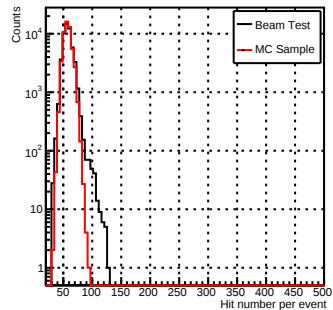
NHit_e-_50GeV
