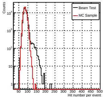
NHit_e-_60GeV
