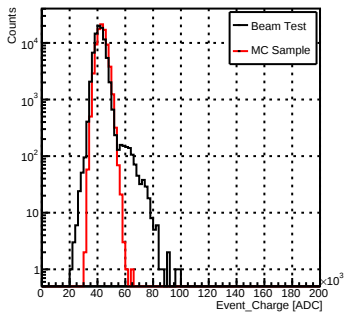
LowGain_e-_60GeV
