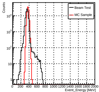
Event_Energy_e-_20GeV
