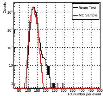
NHit_e-_80GeV
