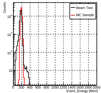
Event_Energy_e-_10GeV
