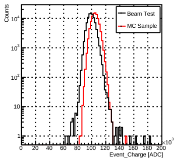
LowGain_e-_70GeV
