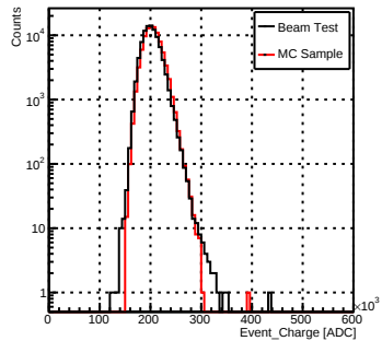
HighGain_e-_80GeV
