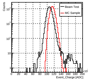
LowGain_e-_80GeV
