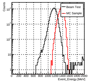
Event_Energy_e-_80GeV
