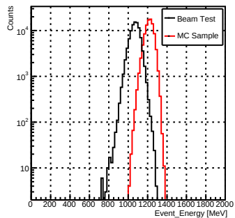
Event_Energy_e-_70GeV
