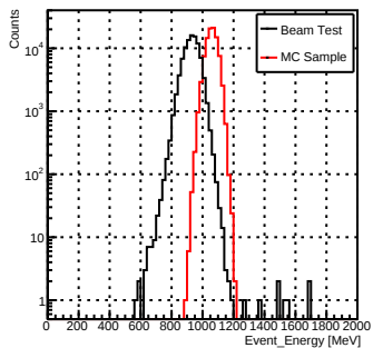
Event_Energy_e-_60GeV
