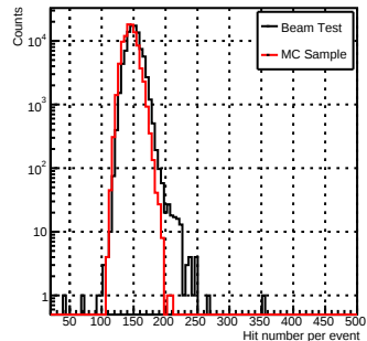
NHit_e-_50GeV
