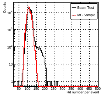
NHit_e-_70GeV
