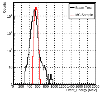
Event_Energy_e-_30GeV
