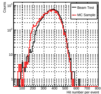
NHit_pi-_70GeV
