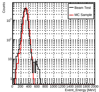
Event_Energy_pi_20GeV
