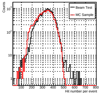
NHit_pi-_60GeV
