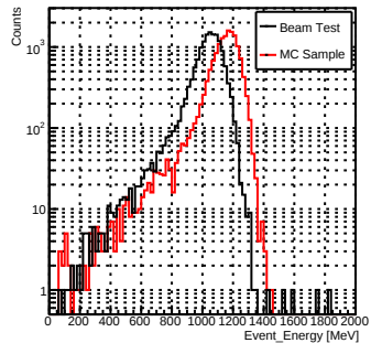
Event_Energy_pi_70GeV
