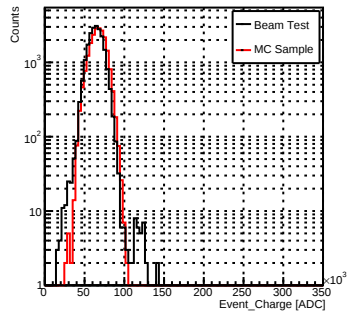
LowGain_pi-60GeV
