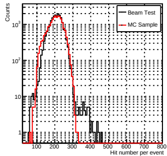
NHit_pi-_30GeV
