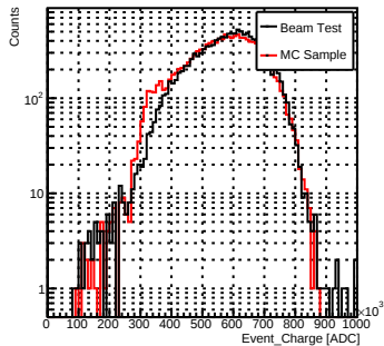
HighGain_pi_80GeV
