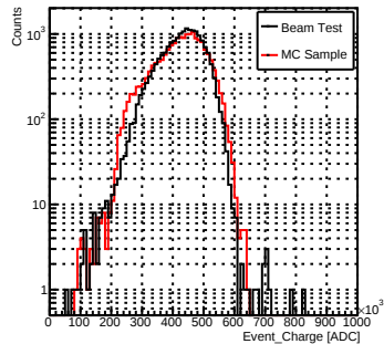
HighGain_pi_50GeV
