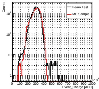
HighGain_pi_30GeV
