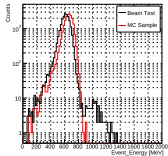
Event_Energy_pi_40GeV
