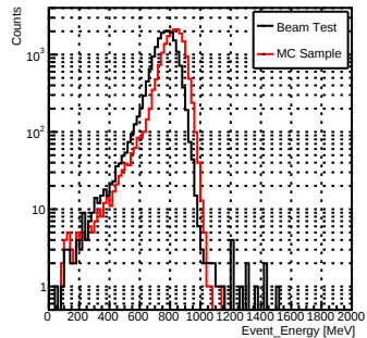
Event_Energy_pi_50GeV
