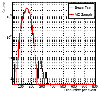
NHit_pi-_20GeV
