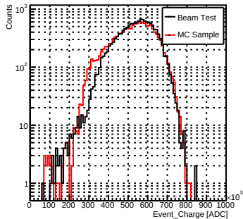
HighGain_pi_70GeV
