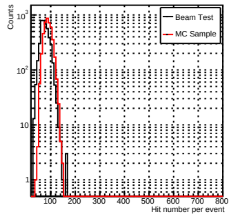
NHit_pi-_10GeV
