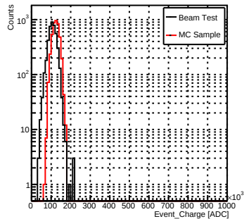
HighGain_pi_10GeV
