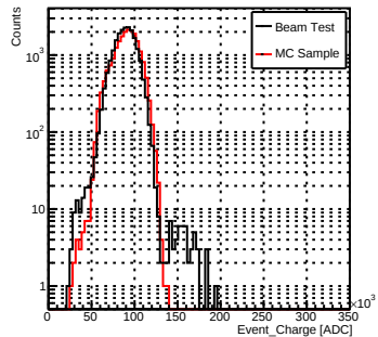
LowGain_pi-70GeV
