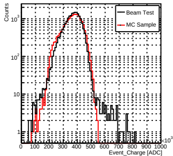
HighGain_pi_40GeV
