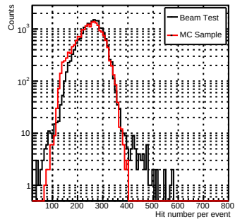
NHit_pi-_40GeV
