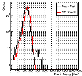
Event_Energy_pi_30GeV
