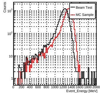
Event_Energy_pi_80GeV
