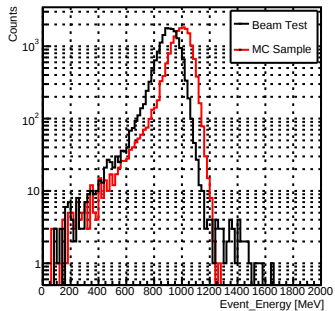
Event_Energy_pi_60GeV
