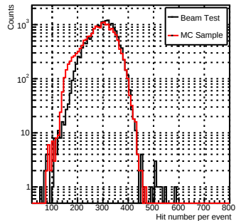
NHit_pi-_50GeV
