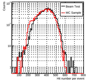
NHit_pi-_80GeV
