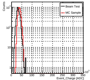
LowGain_pi-50GeV
