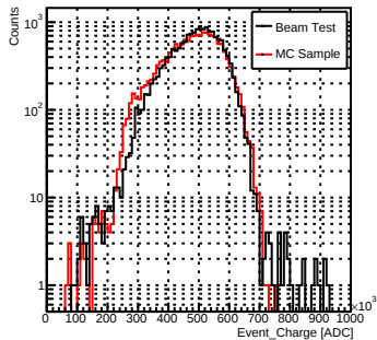
HighGain_pi_60GeV
