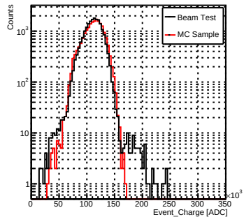
LowGain_pi-80GeV
