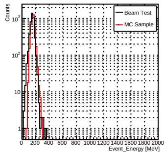
Event_Energy_pi_10GeV
