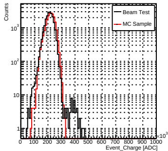
HighGain_pi_20GeV
