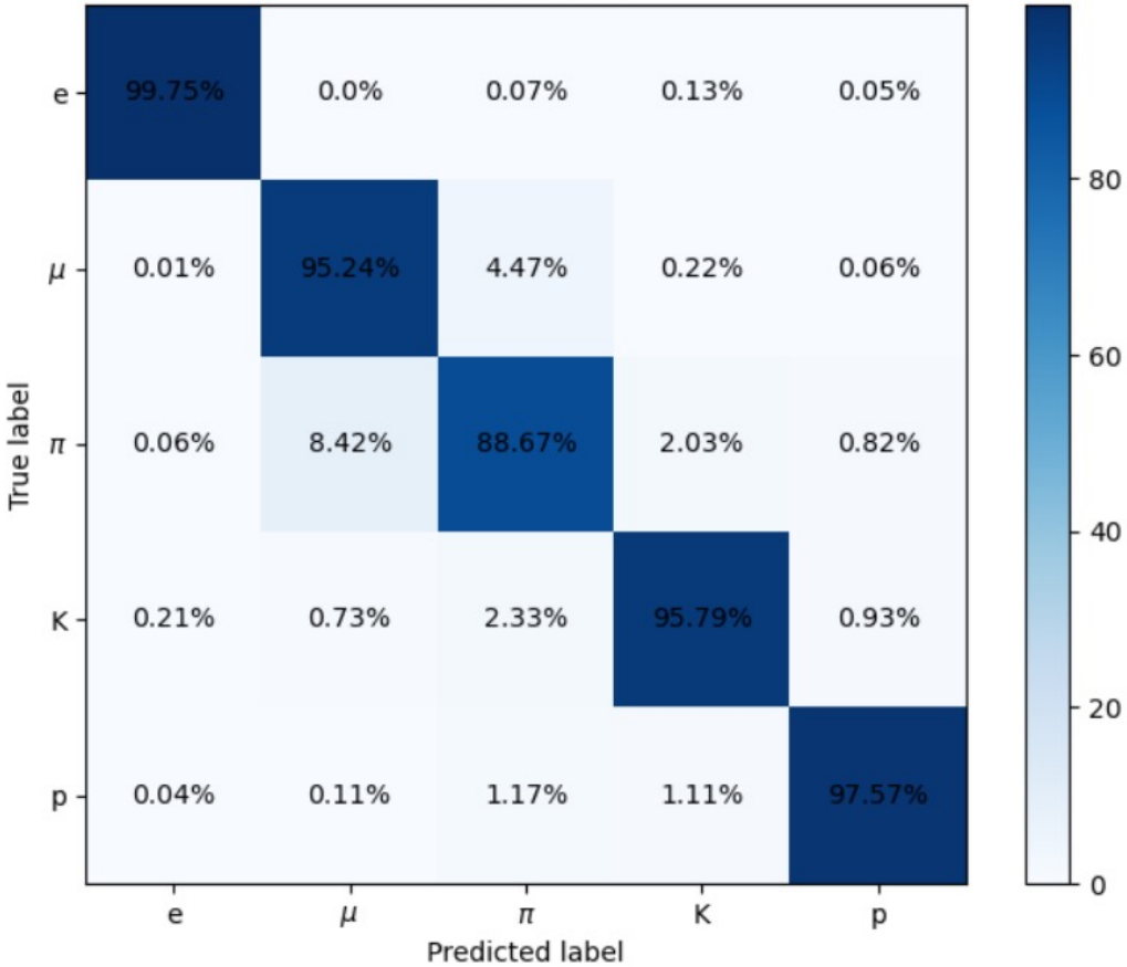
Confusion matrix
