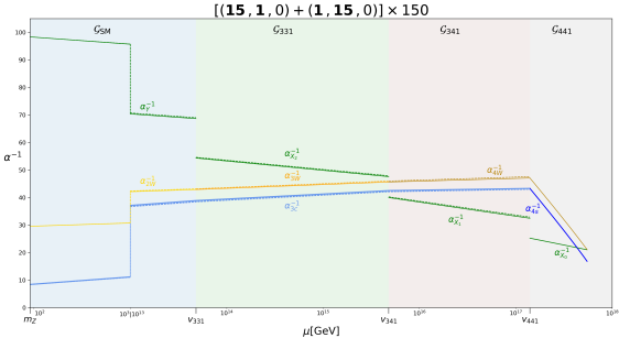
Figure: The RGEs of the SU(8) theory with 150 additional Higgs fields of (\mathbf{15}, \mathbf{1}, 0)_{\text{H}} \oplus (\mathbf{1}, \mathbf{15}, 0)_{\text{H}} . [2406.09970]
