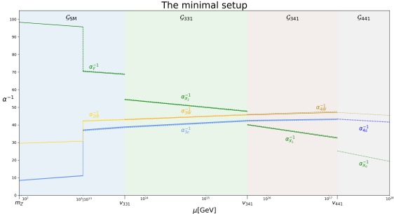
Figure: The RGEs of the minimal SU(8) setup. [2406.09970]
