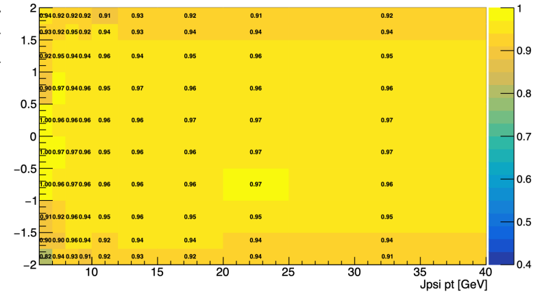
vertex probability
