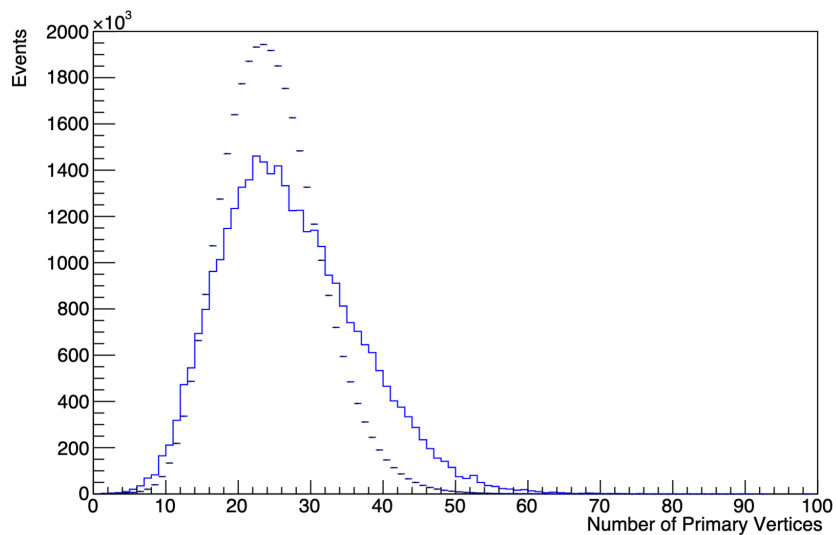
no cut
