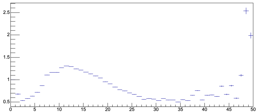
corrector
