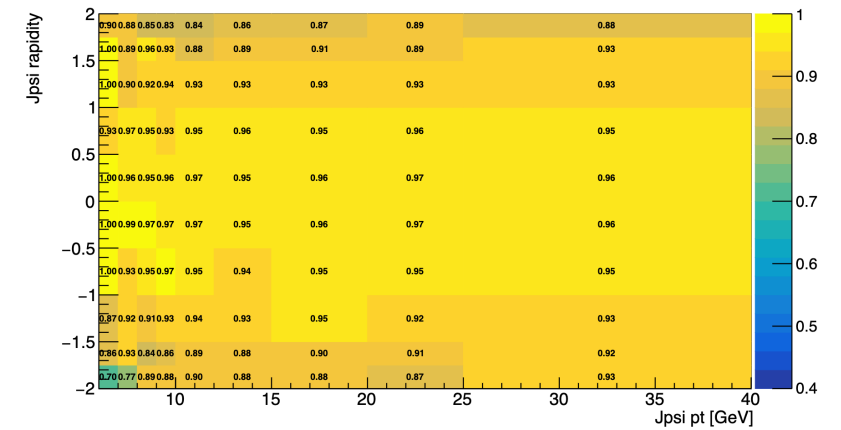
vertex probability
