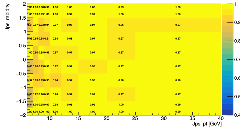
selection probability
