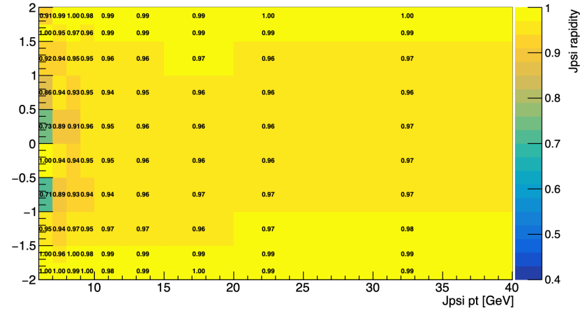
selection probability
