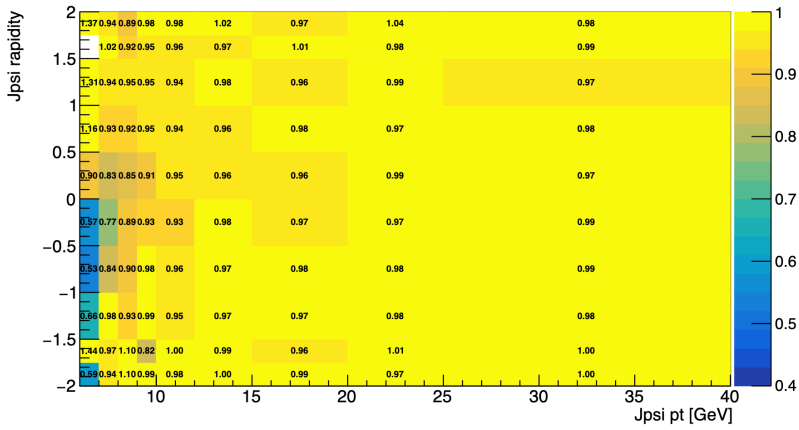
reconstruct probability
