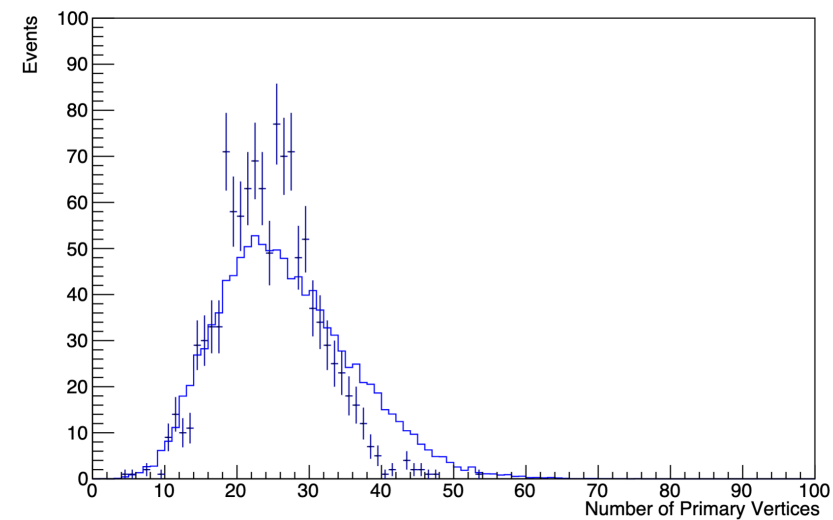
four mu fit and \mu_{pt} > 3.5
