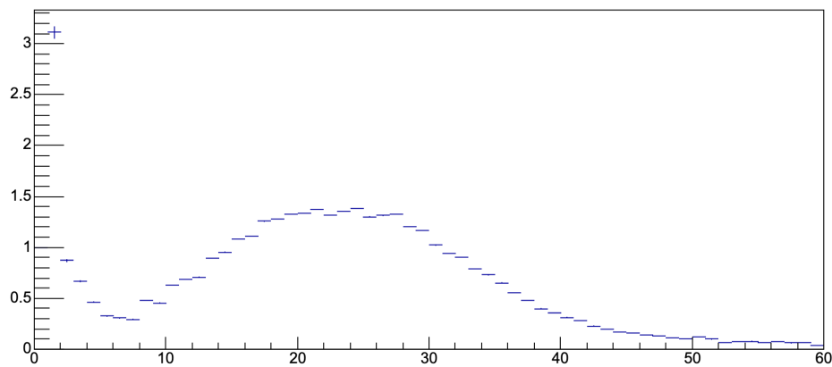
corrector
