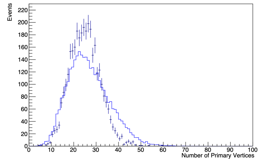
\mu_{pt} > 3.5
