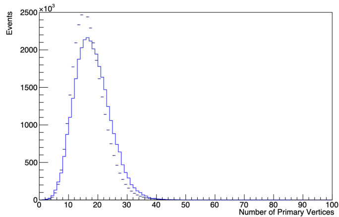
no cut
