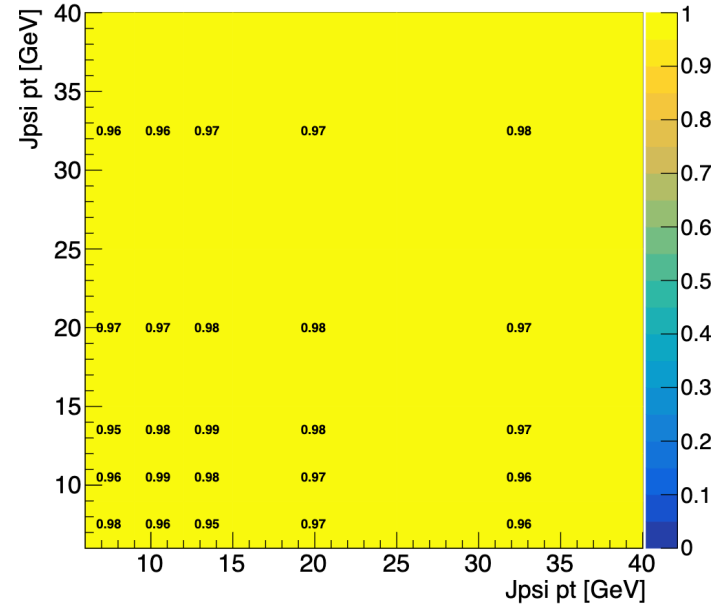
pass triMatched probability
