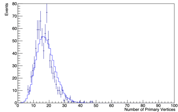
apply fourmu fit and mu_pt>3.5GeV
