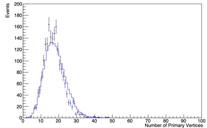
mu_pt>3.5GeV
