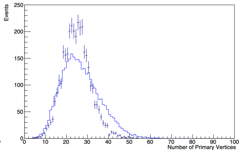
four mu fit
