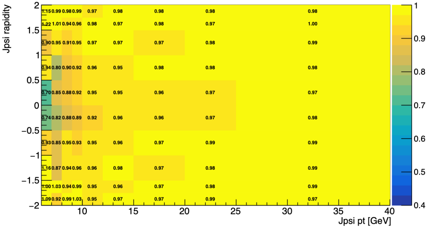
reconstruct probability
