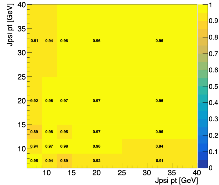
pass triMatched probability
