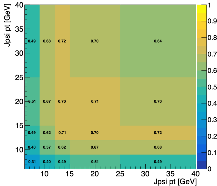
pass HLT probability
