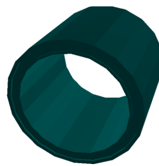
DD4hep_MultiLayerTracker
