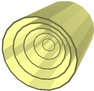
DD4hep_SiTrackerBarrel
