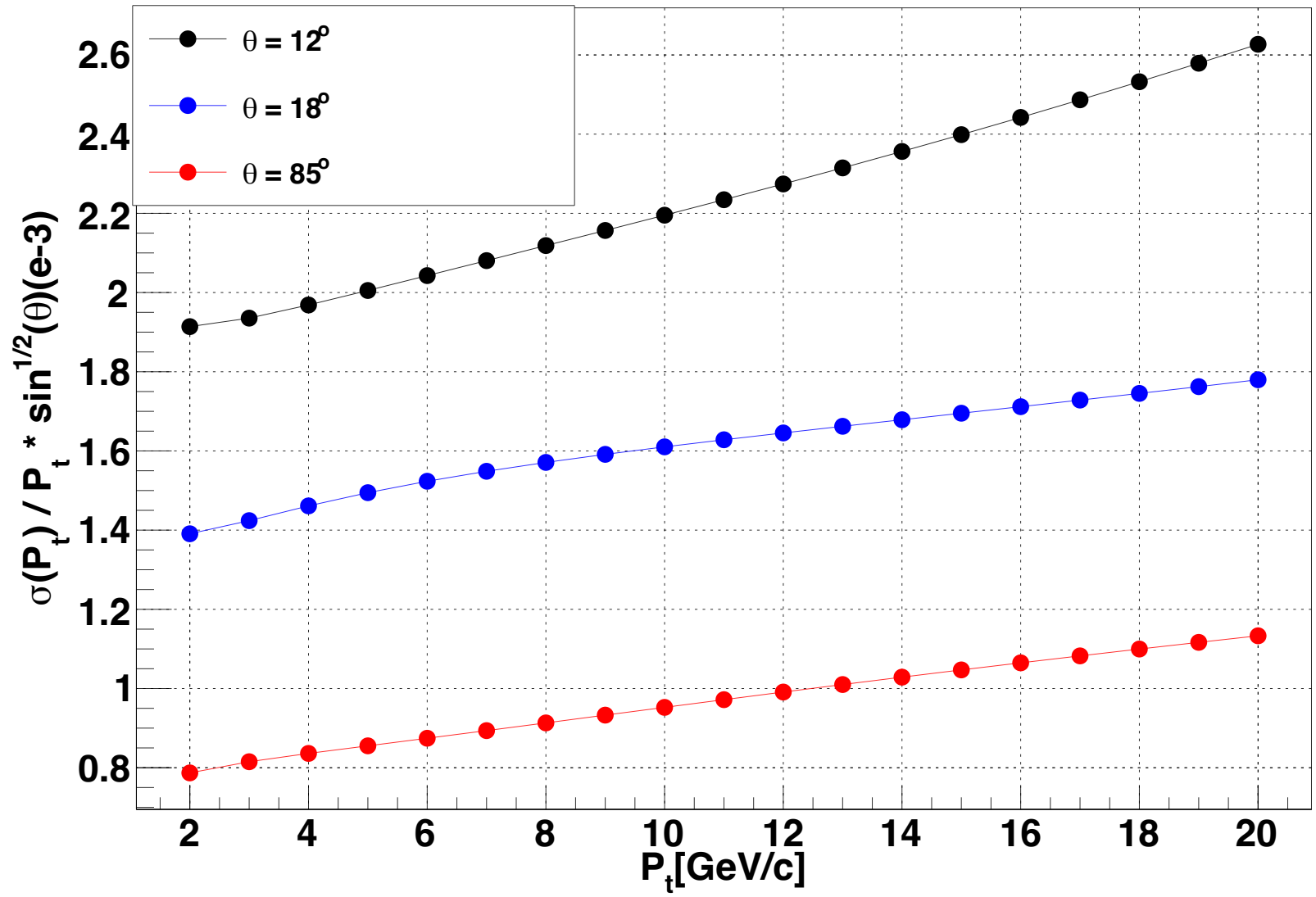
P_t resolution vs P_t for different polar angles
