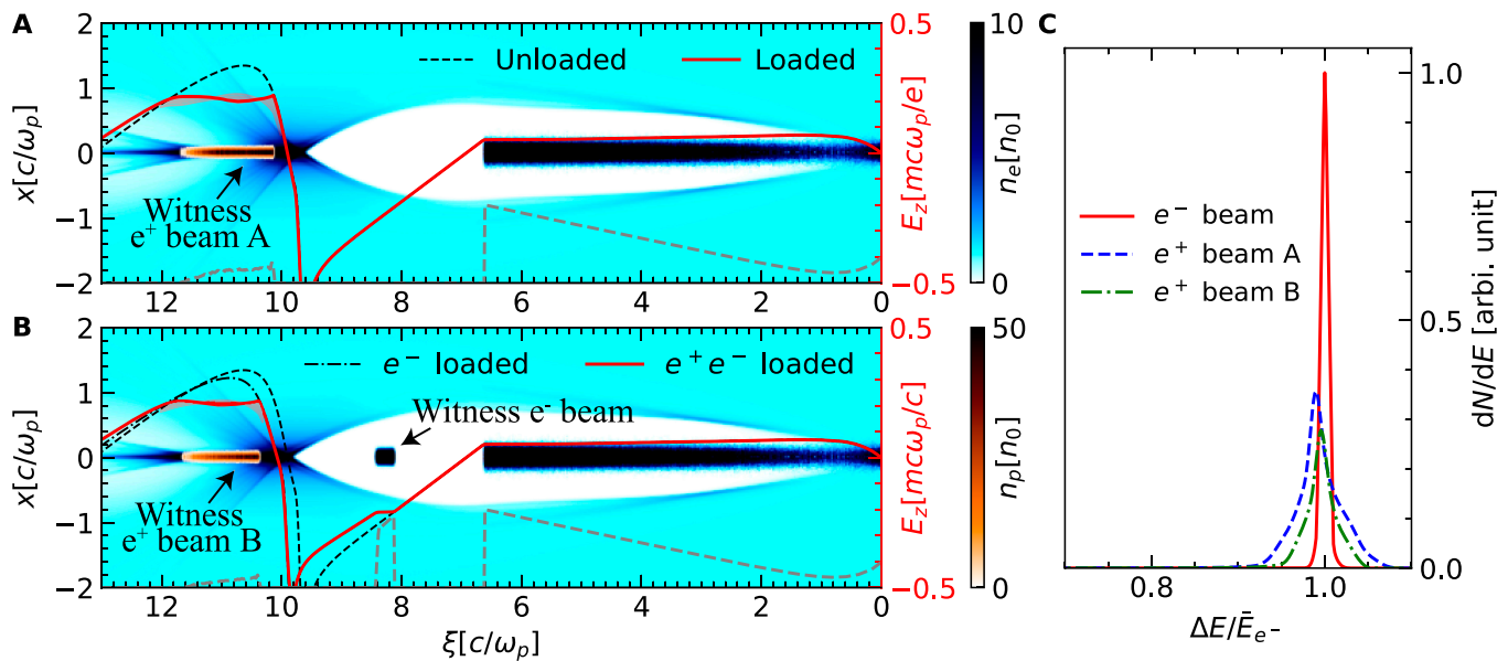
Fig. 4. Configurations of the HTR (A) positron and (B) simultaneous electron and positron acceleration. Gray dashed lines denote the beam current profile. (C) Spectra of the accelerated electron and positron beams.
