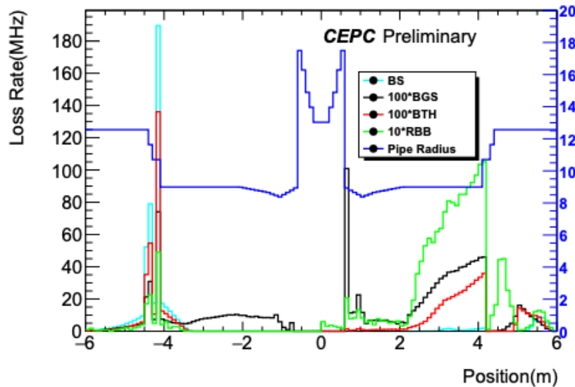
(a) Without collimators
