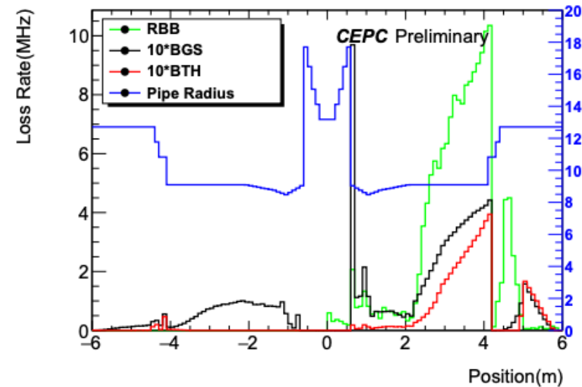
(b) With collimators
