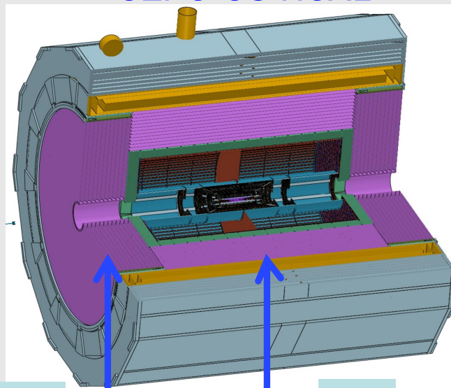
➤ CEPC-GS-HCAL
