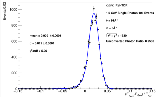
A RooPlot of " (E_{\text{Reco}} - E_{\text{Gen}}) / E_{\text{Gen}} "
