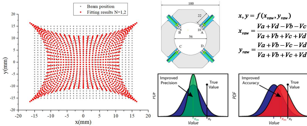
Figure 1.8 The beam position monitors (BPMs) inside flanges will have detect beam bunches that can steer the IP z position. The BPMs single beam pipes before the quadrupole magnets can be precise to 1 \mu\text{m} on the beam x,y positions.
