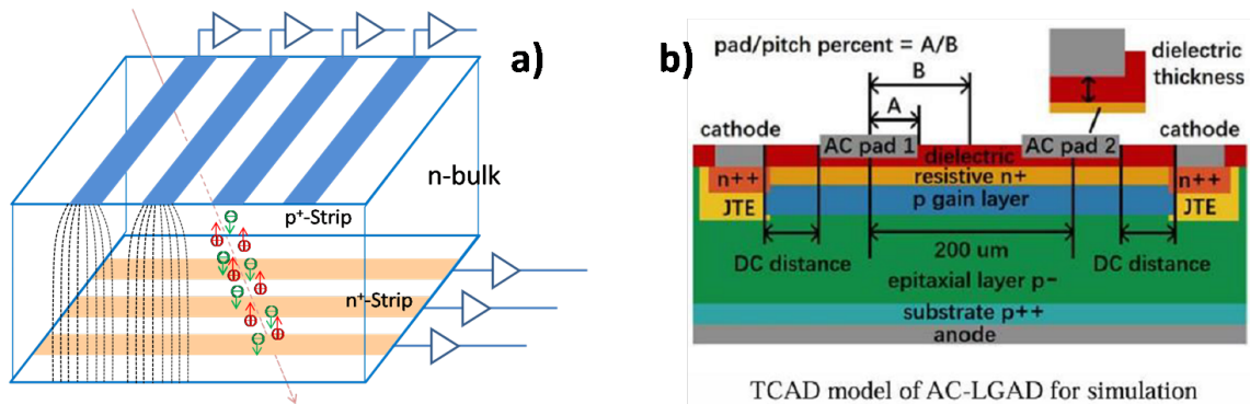
Figure 1.18 Options of silicon position detector: a) the traditional double-sided strip detector, and b) AC-coupled LGAD detector with double AC layers for 2D impact position measurement.
