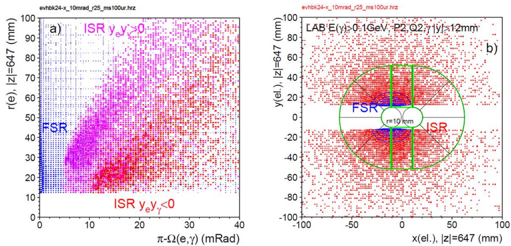
Figure 1.14 Event with radiative photon ( E_\gamma > 0.1 \text{ GeV} ) are plotted for e, \gamma separation. a) the scattered electron position in front of LYSO is plotted for the LAB frame x-y radius vs e, \gamma opening angle in the same z-hemisphere. b) the electron hit positions in LAB x-y frame are shown. In case of FSR both e and \gamma are close beam pipe; with an ISR, e and \gamma are spread wider.
