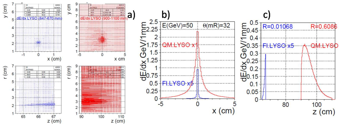
Figure 1.19 Electromagnetic shower of 50 GeV electrons at 32 mRad vertical at 90^\circ . The dE/dx depositions are plotted in the LYSO modules of 2X_0 before flange (Fl.LYSO) and 17.4X_0 before the quadrupole magnet (QM.LYSO). In a) the dE/dx depositions are plotted in x - y and r - z positions with r = \sqrt{x^2 + y^2} the radius in LAB frame, projection in x axis and z axes, that is normalized per event.
