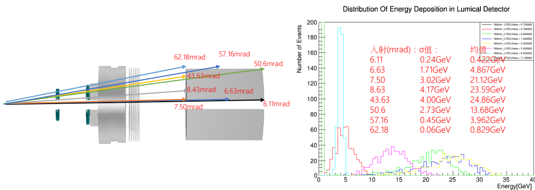
Figure 1.22 The scattered electrons of BHLUMI with projected truth directions
