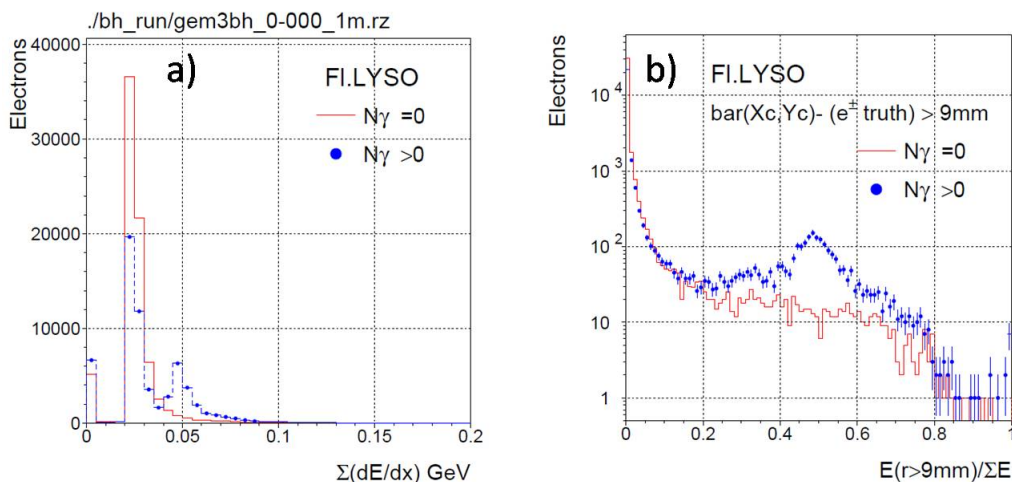
Figure 1.20 The scattered electrons of BHLUMI with projected truth directions entering LYSO at |z| = 64.7 mm, |y| > 12 mm, are simulated with GEANT. The energy deposits of electrons in a half-circle module are plotted in a). The double peak with photon could be with an FSR adjacent to the electrons. The fraction of energies in LYSO bars 9 mm off the projected electron direction is plotted in b), indicating the observable of a photon that can be identified by the LYSO bar segmentation.
