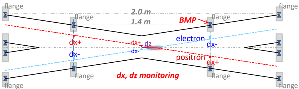
Figure 1.23 The beam currents at IP region is illustrated for offsets to be measured with Beam Position Monitor.
