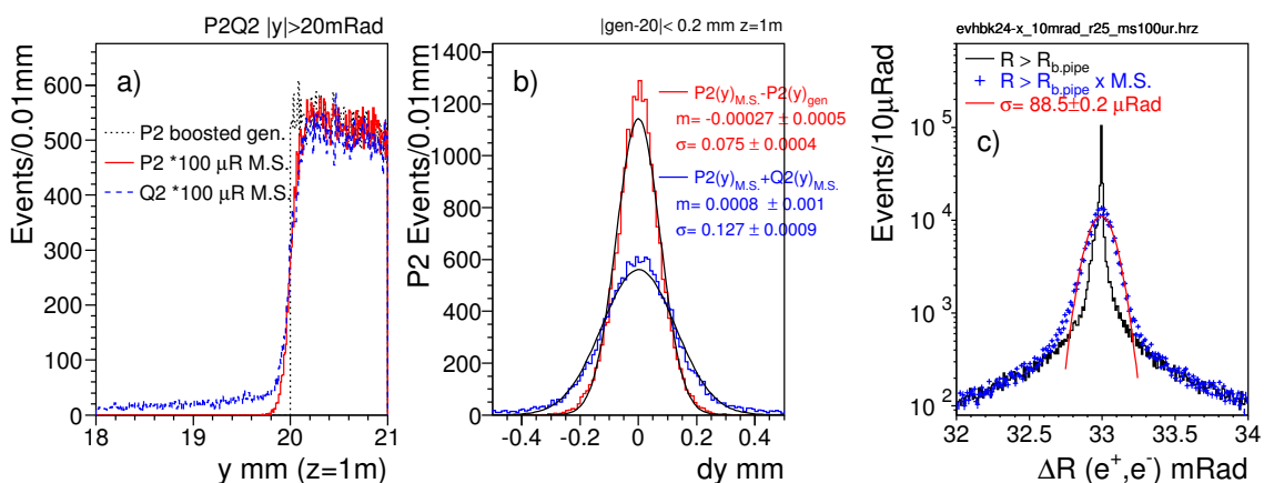
Figure 1.24 The scattered electrons (P2) and positrons (Q2) both accepted within the fiducial edges of LumiCal at |z| = 1 \text{ m} are plotted in a) for the distribution in |y| . The dotted is the BHLUMI generated P2 being cut at |y| > 20 \text{ mm} . The multiple scattering (M.S.) smeared P2 is plotted in red solid line. The Q2 in the other z -side is plotted in blue dashed, where the tail are events having radiative photons. The smearing width is with
