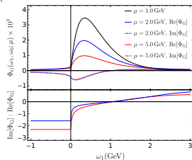
Numerics for the RG evolution:
