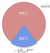
m_b^{\text{OS}} -composition
