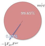
m_e^{\text{OS}} -composition
