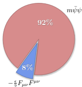
m_t^{\text{OS}} -composition
