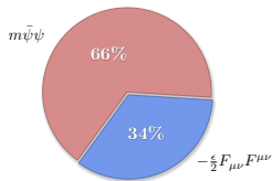
m_c^{\text{OS}} -composition
