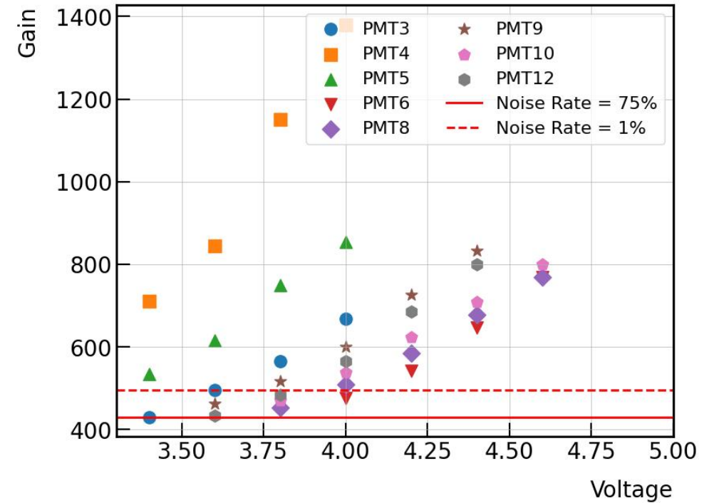
Gain vs Voltage for Different PMTs
