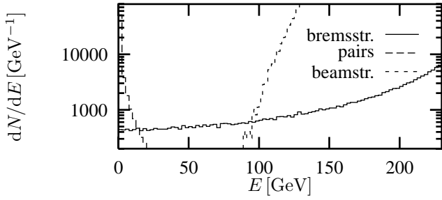
Figure 6: The low energy particle spectra for the TESLA parameters due to the pair production, bremsstrahlung and beamstrahlung.
