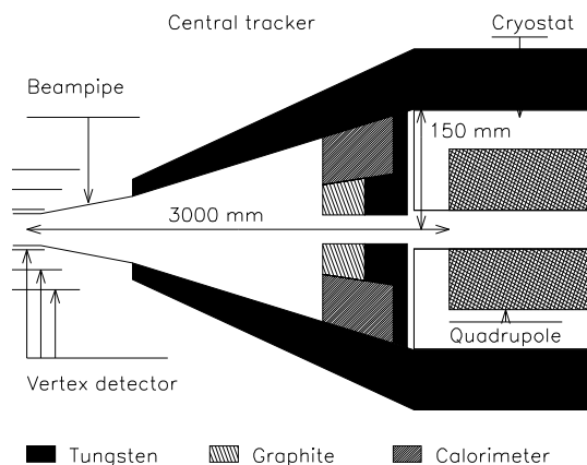
Figure 5: The layout of the mask in the detector of TESLA.
