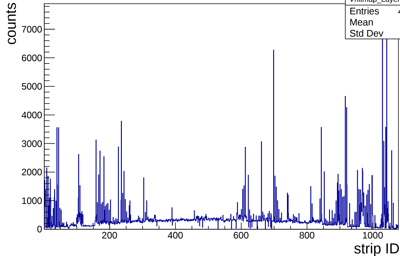
hit map, V strip, Layer2, bottom
