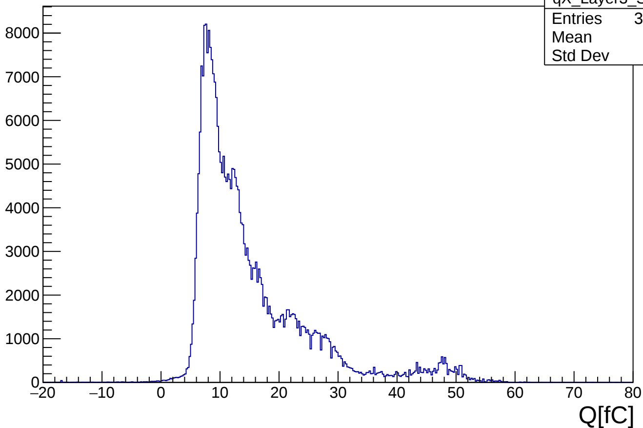
distribution of Q, X strip, Layer3, up
