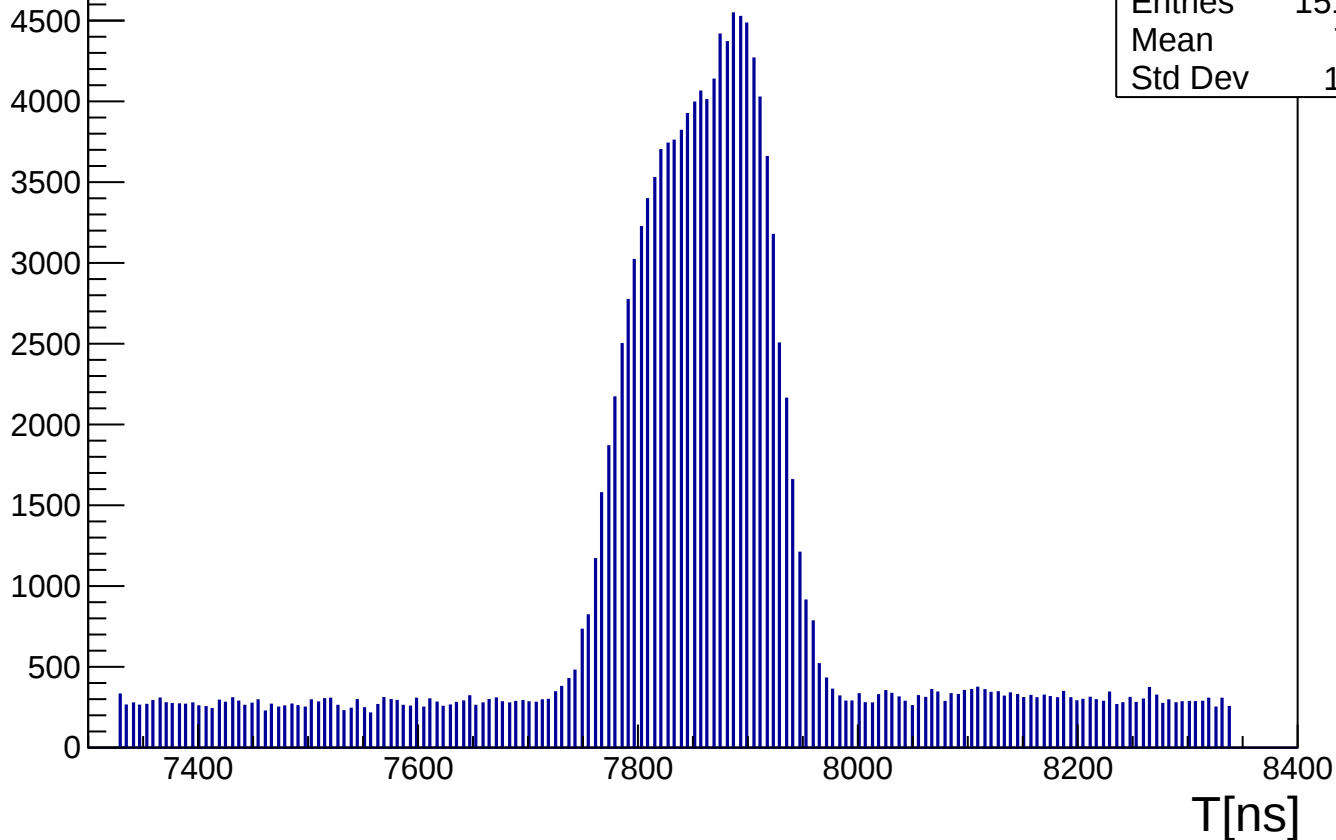
distribution of T, X strip, Layer2, up
