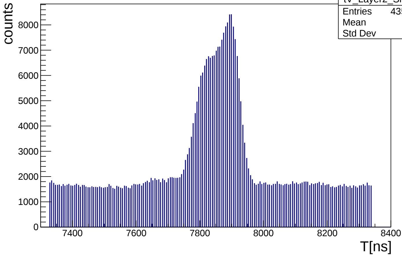
distribution of T, V strip, Layer2, bottom
