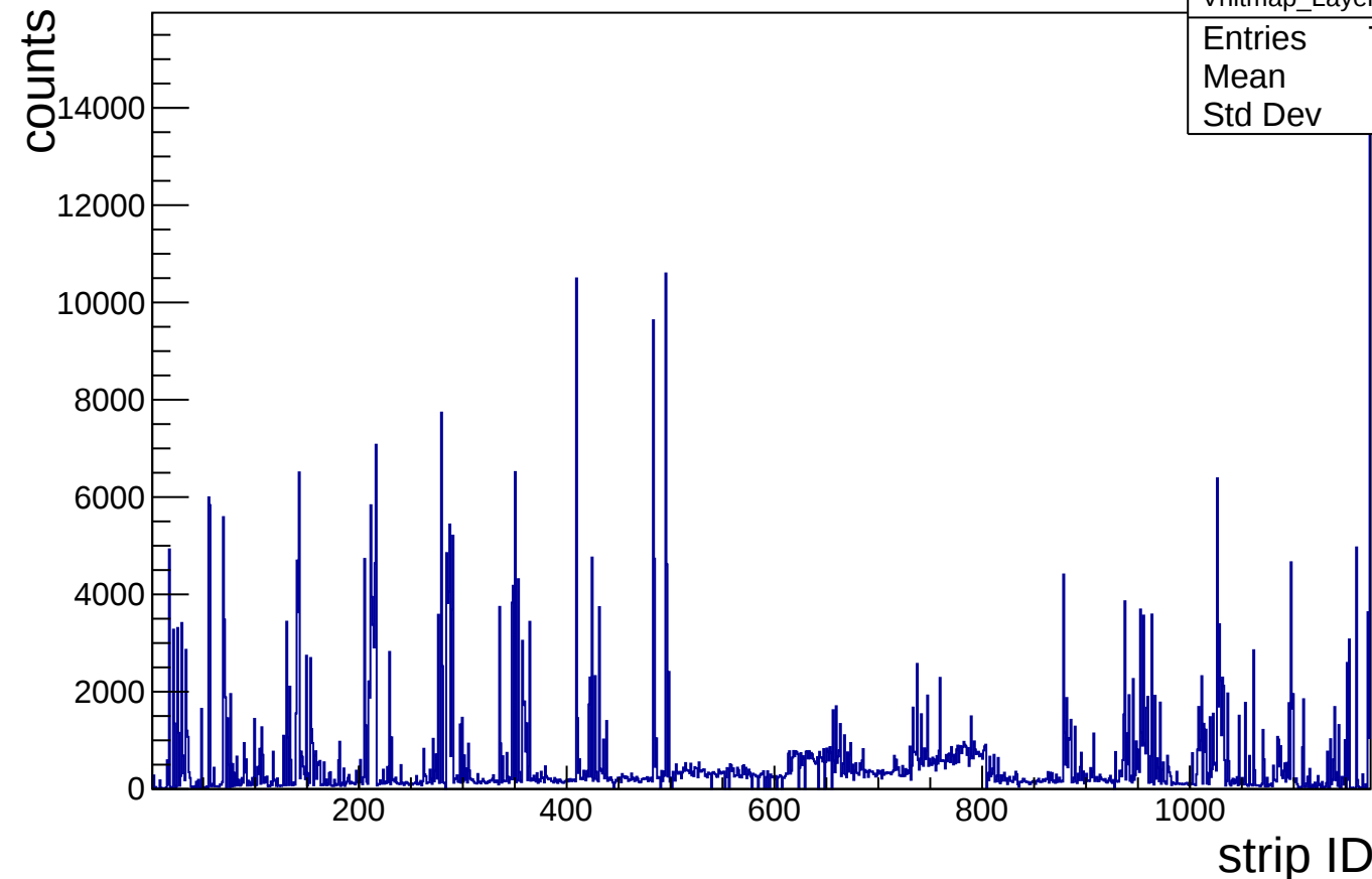
hit map, V strip, Layer1
