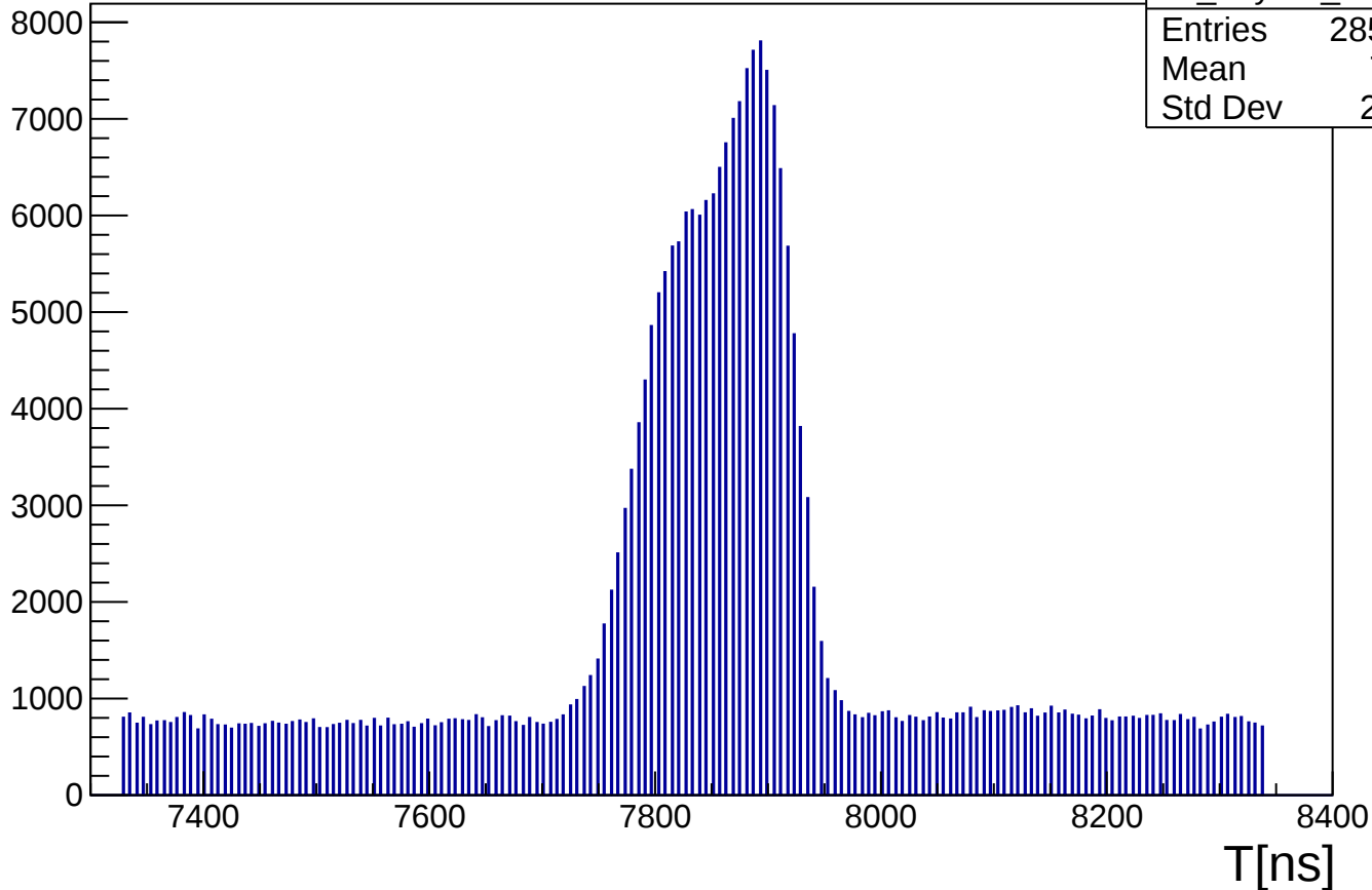
distribution of T, X strip, Layer2, bottom
