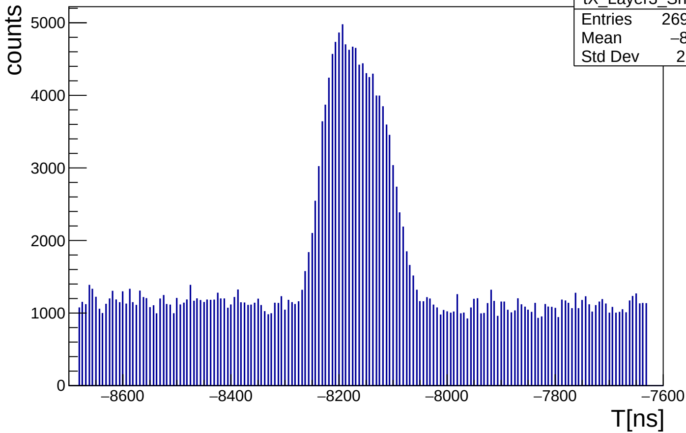
distribution of T, X strip, Layer3, bottom
