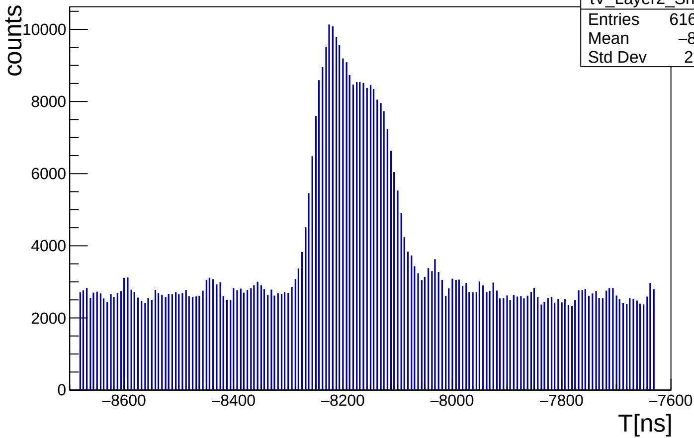
distribution of T, V strip, Layer2, bottom
