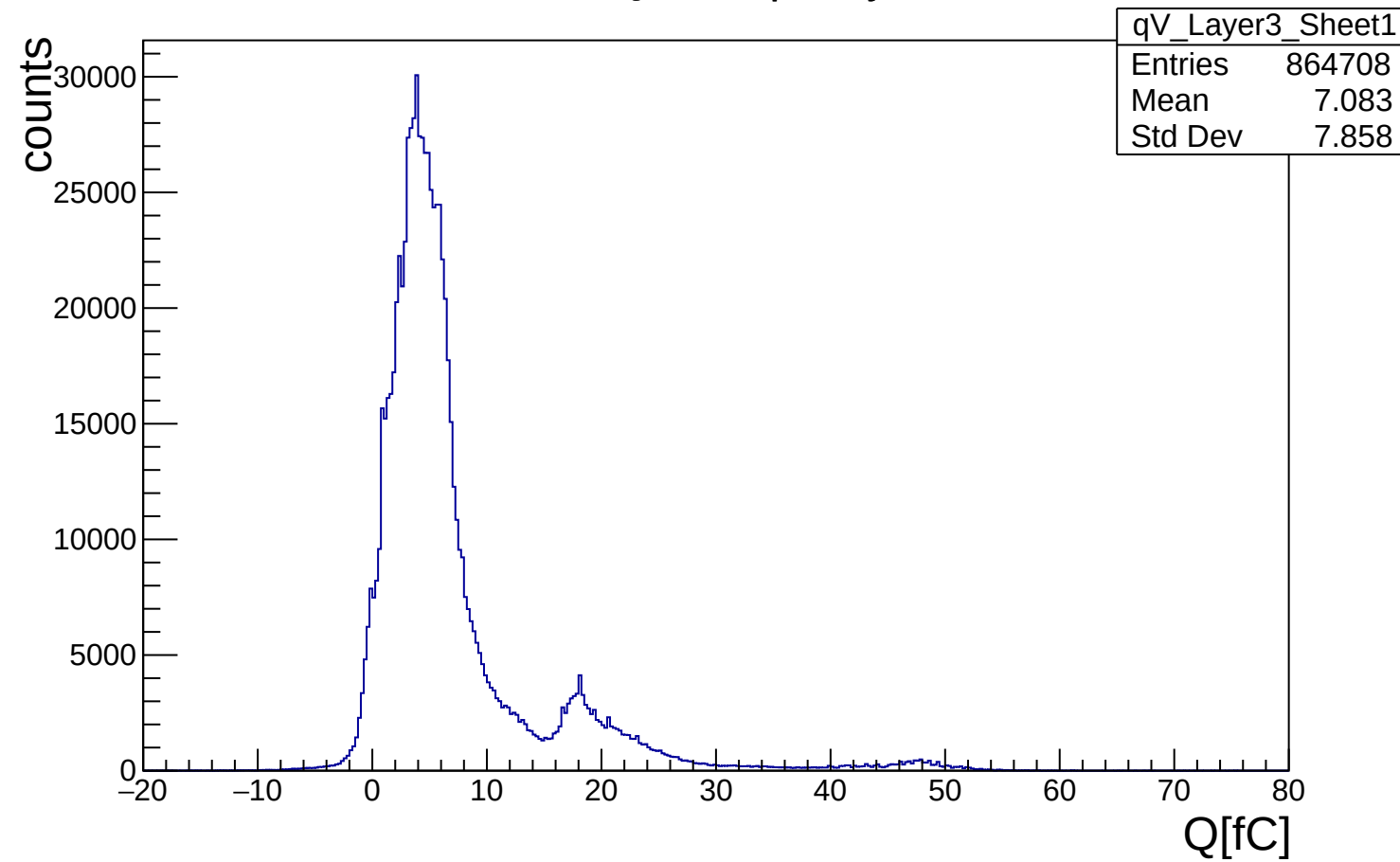
distribution of Q, V strip, Layer3, bottom
