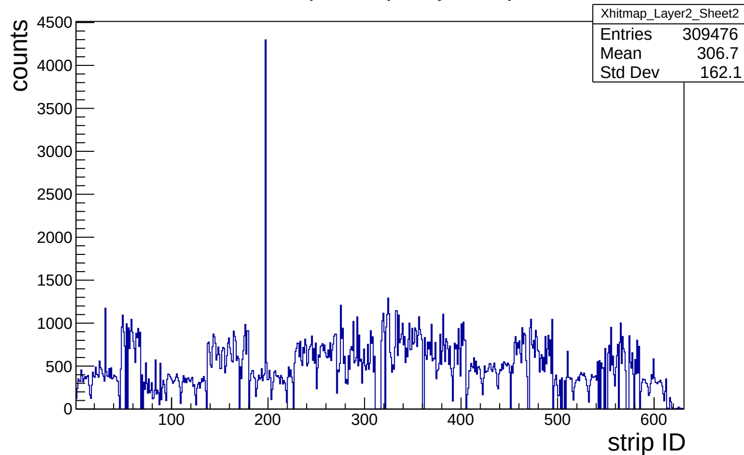
hit map, X strip, Layer2, up
