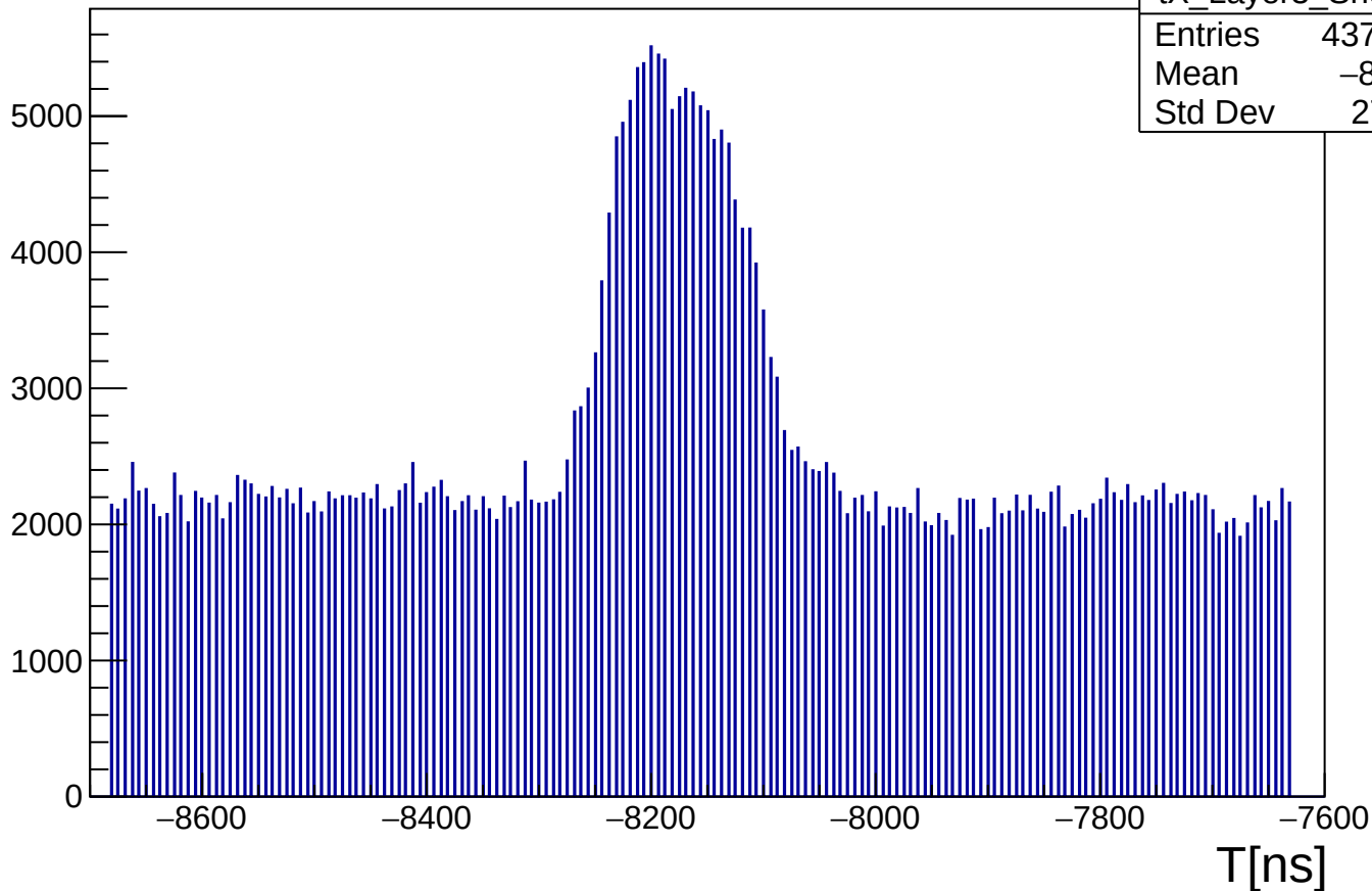
distribution of T, X strip, Layer3, up
