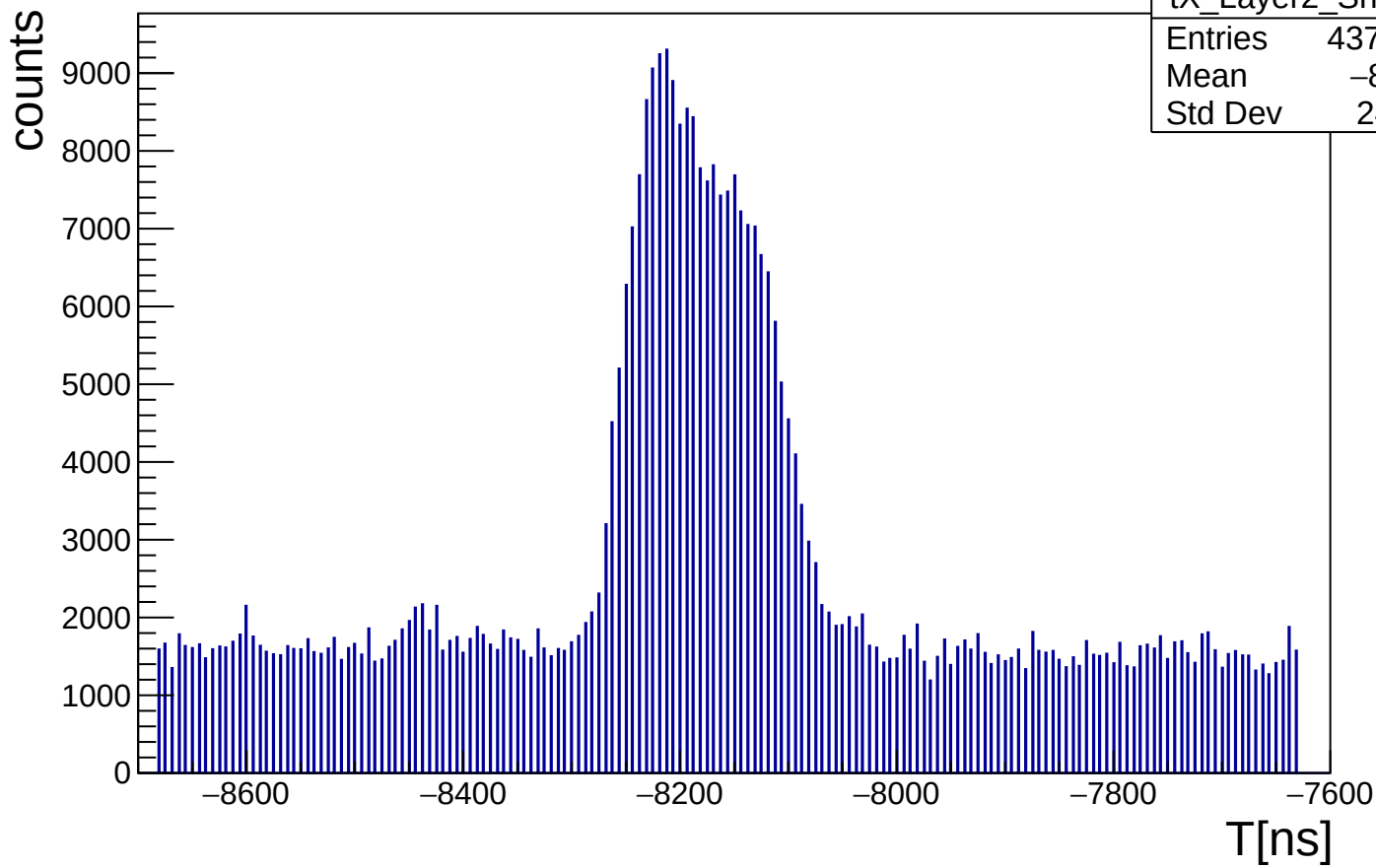
distribution of T, X strip, Layer2, bottom
