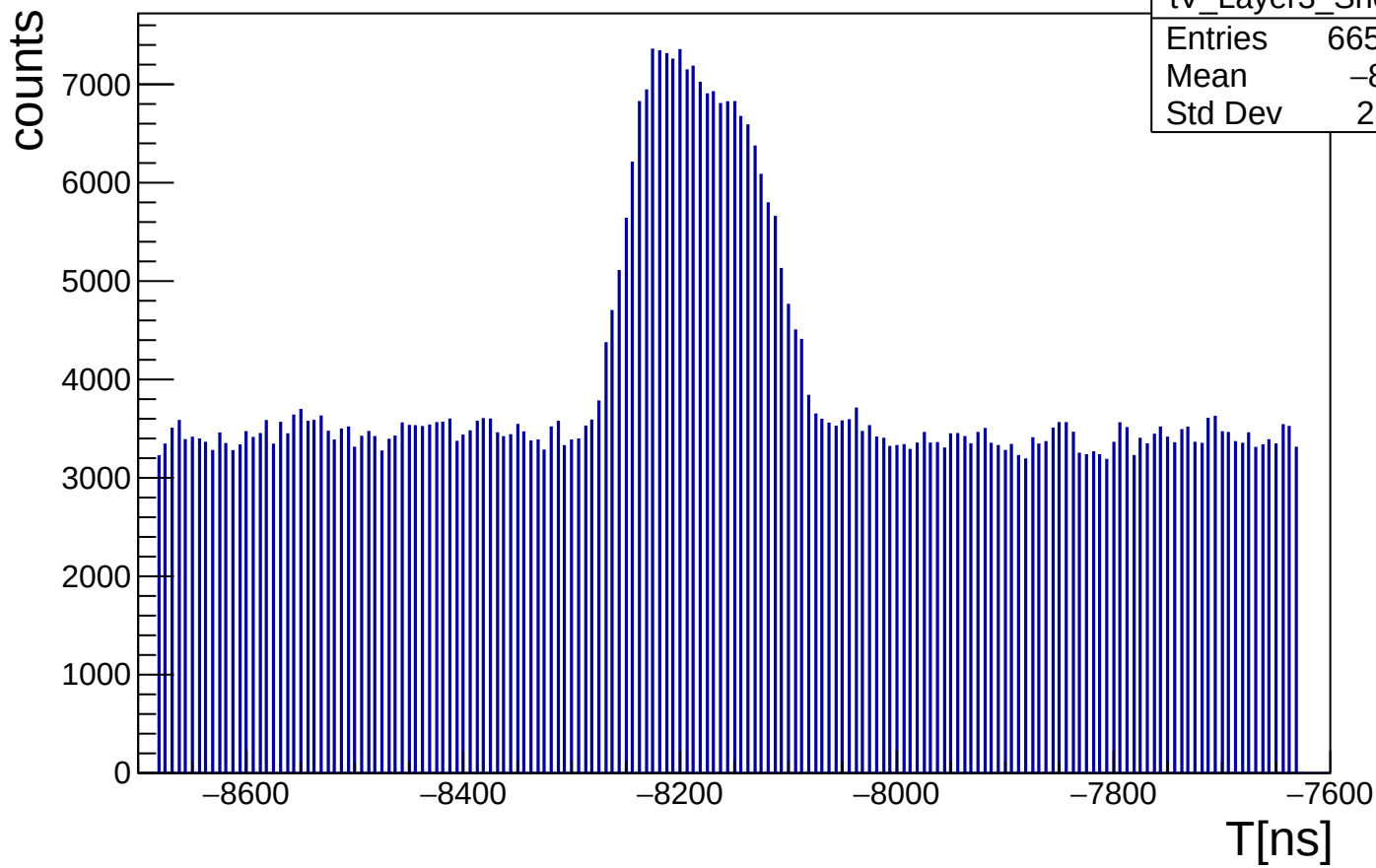
distribution of T, V strip, Layer3, up
