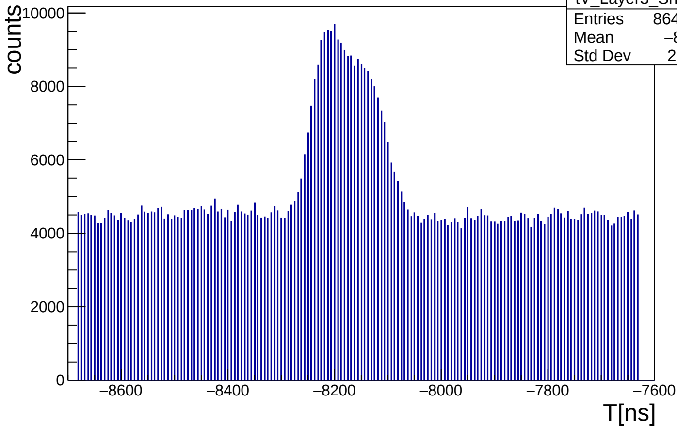
distribution of T, V strip, Layer3, bottom
