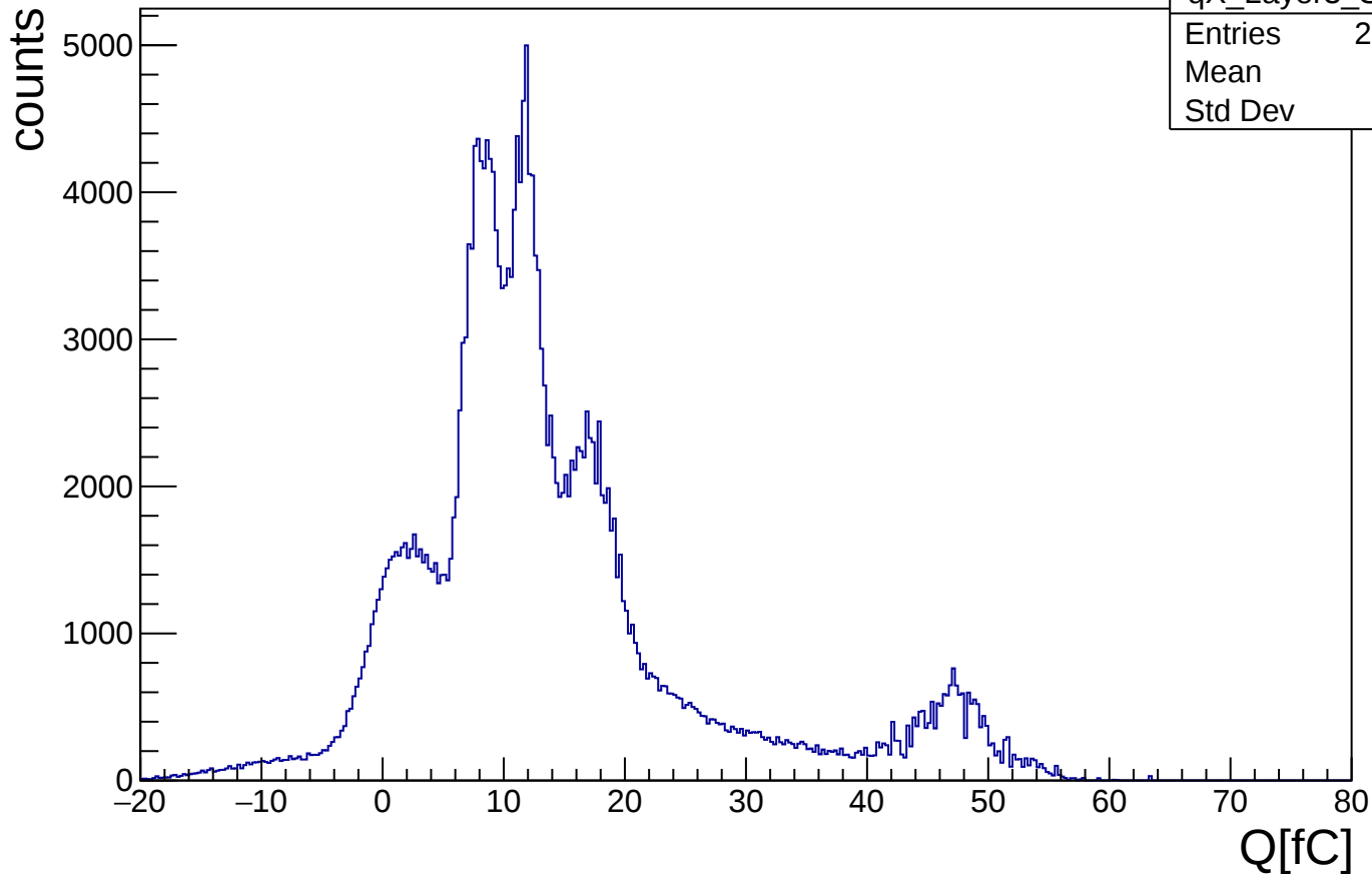
distribution of Q, X strip, Layer3, bottom
