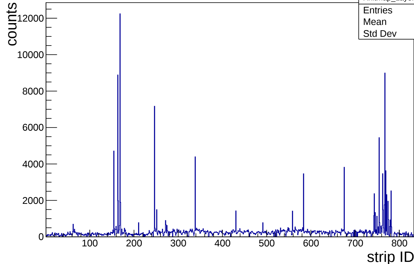
hit map, X strip, Layer3, bottom
