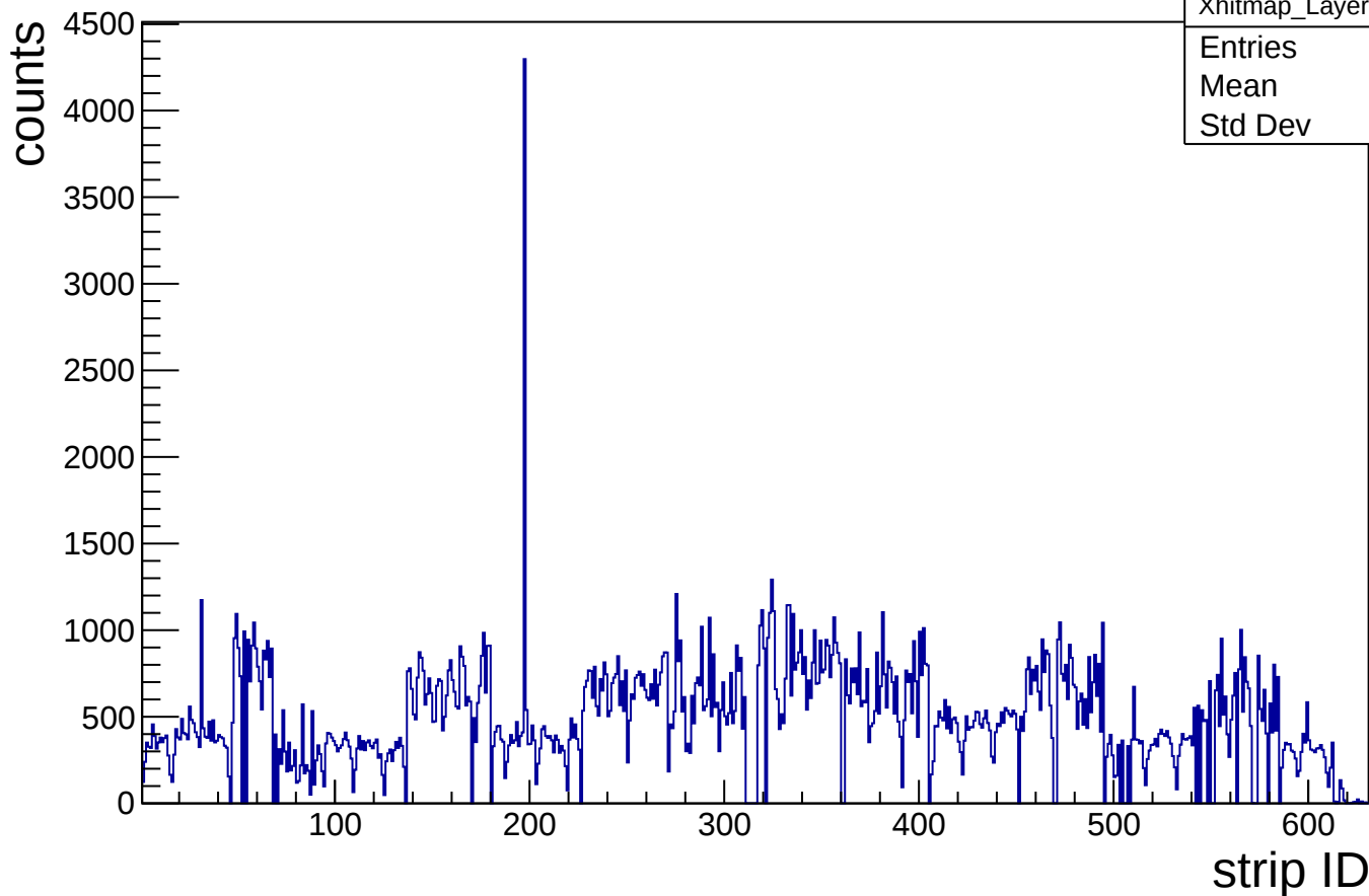
hit map, X strip, Layer2, up
