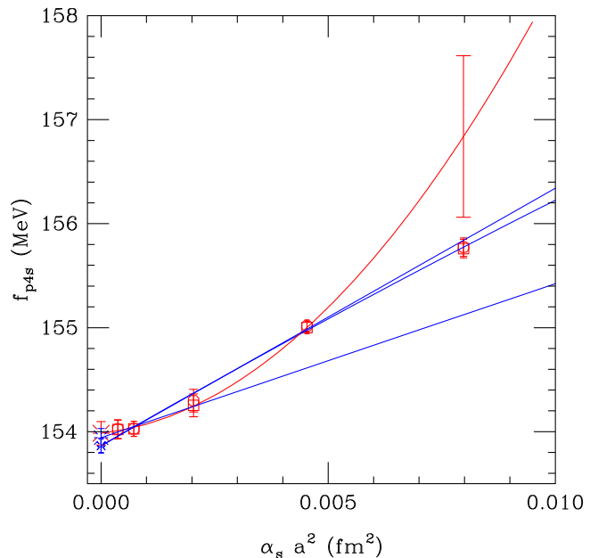
FIG. 5. Continuum extrapolations for f_{p4s} on the physical quark mass ensembles. Our central fit, shown in red, is quadratic in \alpha_s a^2 excluding the 0.15 fm data. Alternative fits used for estimating systematic error are shown in blue. These include a quadratic fit including all the data, a linear fit including data up to 0.12 fm, and a linear fit including data up to 0.09 fm. The large error bar on the central fit line shows the statistical error on this fit at 0.15 fm, the point that is not included in this fit.
