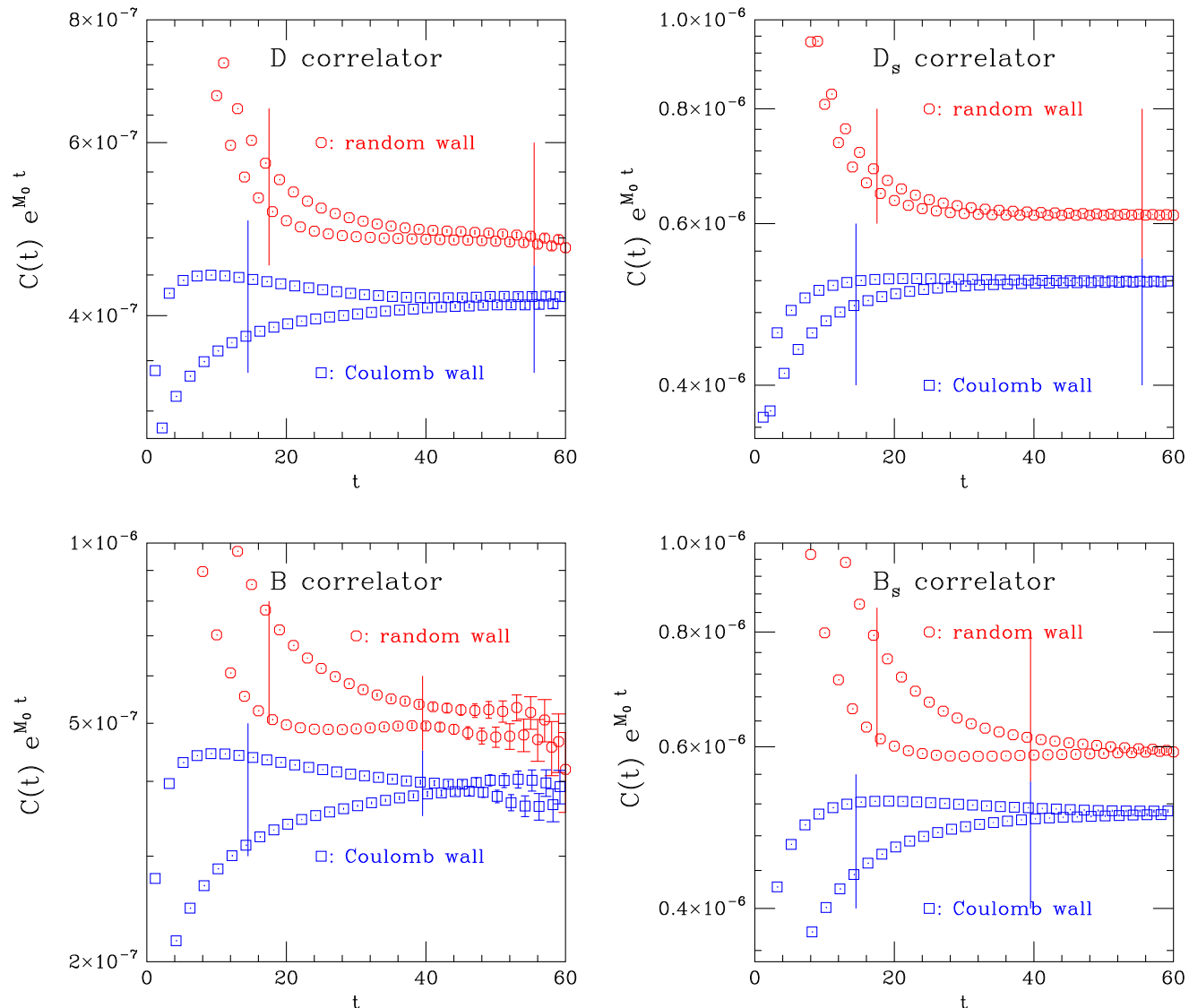
FIG. 2. Pseudoscalar correlators for the D (top left), D_s (top right), B (bottom left), and B_s (bottom right) mesons on the a \approx 0.042 fm physical-quark-mass ensemble. Here the valence charm-quark mass is equal to the sea charm-quark mass, and the bottom-quark mass is equal to 4.5 times the charm-quark mass. The red octagons are the random-wall source correlator and the blue squares the Coulomb-wall correlator. Both correlators have been rescaled by e^{M_0 t} where M_0 is the ground-state mass; the random-wall correlators have also been multiplied by an arbitrary factor to make the vertical scale convenient. The vertical lines show the fit ranges used in the 3 + 2 state fits in our analysis. The D - and D_s -meson fits have p -values 0.66 and 0.71 respectively, while the B - and B_s -meson fits have p -values 0.29 and 0.40 respectively. (The oscillatory behavior in t comes from the positive parity states in the correlator.)
