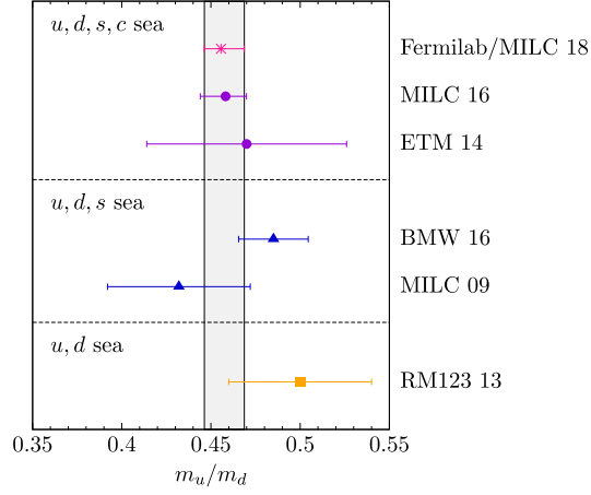
FIG. 13. Comparison of m_u/m_d in Eq. (7.25) (magenta burst) with previous unquenched lattice-QCD calculations [101–105].
