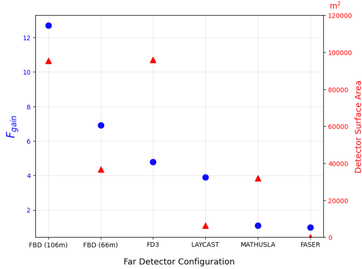
FIG. 59: The gain factor F_{\text{gain}} (left axis) and the corresponding detector surface area (right axis) are shown for various far detector configurations. FBD (106m) has \Delta L set as 100m and FBD (66m) has \Delta L set as 60m.
