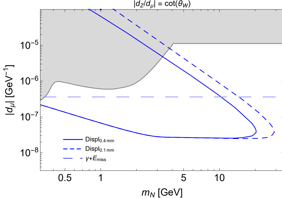
FIG. 70: The potential of FCC-ee to m_N and the dipole coupling |d_\mu| at the 90% C.L. at the Z -pole with a luminosity of 150 \text{ ab}^{-1} . The solid and short-dashed blue lines correspond respectively to the vertex transverse displacement of 0.4 mm and 0.1 mm, and the long-dashed light blue line denotes the sensitivity corresponding to the \gamma +missing energy signature. The sensitivities at CEPC can be obtained by a simple rescaling of the luminosity via \sqrt{150/100} \simeq 1.22 . Taken from Ref. [558].
