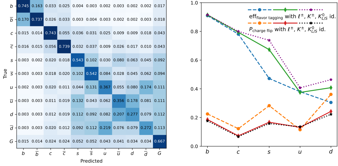
FIG. 5: Jet origin identification performance of full simulated Higgs/ Z to di-jet processes with CEPC conceptual detector [29]. LEFT: The confusion matrix M_{11} with perfect identification of leptons and charged hadrons. RIGHT: Jet flavor tagging efficiency and charge flip rates for quark jets with different scenarios of particle identification: with only lepton identification, plus identification of charged hadrons, plus identification of neutral kaons.
