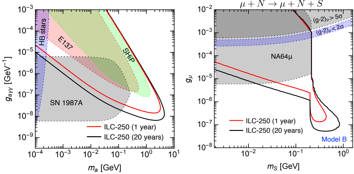
FIG. 55: Both plots are extracted from Ref. [409] and show discovery sensitivities of the beam-dump experiment at the ILC to the ALPs and new scalar particles. Left: sensitivities in the ALP-photon-photon coupling g_{a\gamma\gamma} vs. ALP mass m_a plane, where red and black curves correspond to the bounds of sensitivity for ILC-250 GeV at 95% C.L. with 1- and 20-year statistics; the shaded regions are constraints for E137 from Ref. [411], SN 1987A from Ref. [411, 412], HB stars from Ref. [413], and SHiP from Ref. [411, 414, 415]. Right: sensitivities in the g_\mu vs. m_S plane for Model B ( S couples to muons only, i.e. g_\mu \neq 0 , g_e = g_\tau = 0 ), where the signal process contains a muon in the initial state (i.e. \mu + N \rightarrow \mu + N + S ); the gray shaded regions are constraints from NA64μ and muon g - 2 from Ref. [416]; note that, although the results for m_S > 2m_\mu are absent for NA64μ, it would also have a sensitivity in that region generally.
