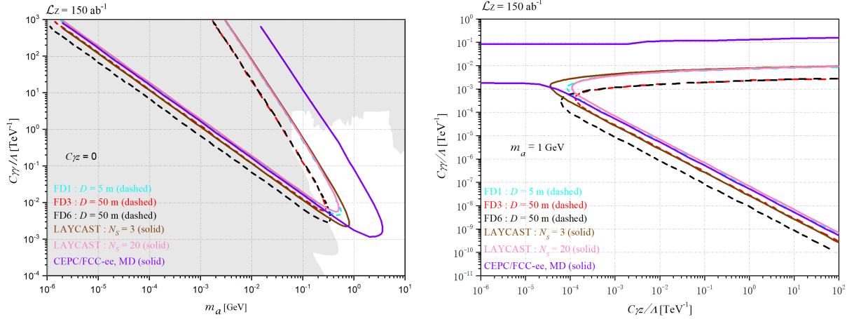
FIG. 52: Left: when C_{\gamma Z} = 0 , sensitivity reaches of representative far detectors FD1, FD3, FD6, LAYCAST and the CEPC/FCC-ee’s main detector (MD) with integrated luminosity \mathcal{L}_Z = 150 \text{ ab}^{-1} in the C_{\gamma\gamma}/\Lambda vs. m_a plane. Right: when both C_{\gamma Z} and C_{\gamma\gamma} are free parameters, sensitivity reaches with m_a = 1 \text{ GeV} in the C_{\gamma\gamma}/\Lambda vs. C_{\gamma Z}/\Lambda plane with \mathcal{L}_Z = 150 \text{ ab}^{-1} . Taken from Ref. [368, 369].
