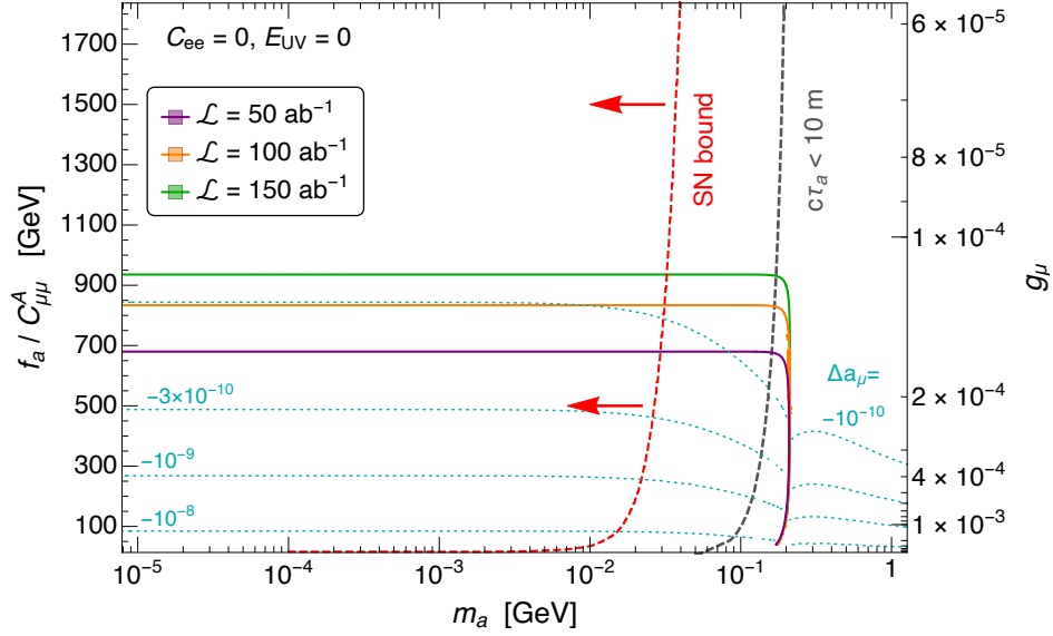
FIG. 44: Prospected CEPC/FCC-ee 95% CL exclusion on the (m_a, f_a/C_{\mu\mu}^A) plane for a muonic ALP ( C_{ee}^A = 0, E_{UV} = 0 ) with different assumptions for the integrated luminosity \mathcal{L} , as indicated. On the right side of the dashed grey line the proper decay length of the ALP is c\tau_a < 10 m. The region to the left of the red dashed line is excluded by SN1987A data, according to the analysis in [382]. The dotted cyan contours show the ALP contribution to the anomalous magnetic moment of the muon, \Delta a_\mu \equiv (g - 2)_\mu/2 . Taken from Ref. [74].
