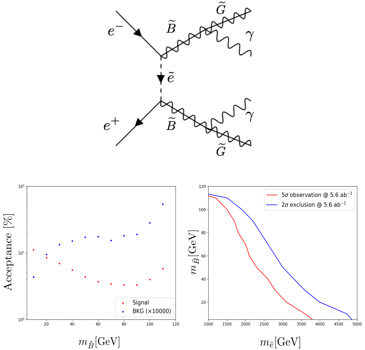
FIG. 61: Top : representative diagram illustrating light bino production. Bottom left : acceptance of signal and background processes as functions of m_{\tilde{B}} . Here the acceptance of the background process has been multiplied by 10,000. Bottom right : 2\sigma exclusion and 5\sigma observation limits on the m_{\tilde{e}} - m_{\tilde{B}} plane at a future lepton collider running with an integral luminosity 5.6 \text{ ab}^{-1} and center-of-mass energy 240 GeV. Regions below the red (blue) curves are observable (excluded).
