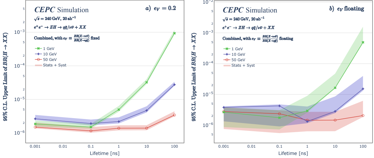
FIG. 37: (Color online) 95% C.L. upper limit on the branching ratio (BR) for the Higgs boson ( H ) decay into pairs of LLPs ( X_1 X_2 ) via e^+ e^- \rightarrow ZH , where \epsilon_V is the ratio \frac{BR(X \rightarrow \nu \bar{\nu})}{BR(X \rightarrow q \bar{q})} . a) : a fixed ratio \epsilon_V = 0.2 , b) : a floating \epsilon_V . The shaded areas indicate statistical and systematic uncertainties combined. Taken from Ref. [69].
