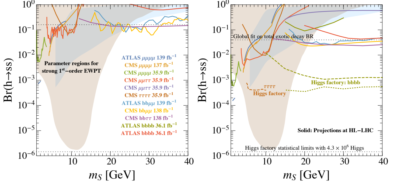
FIG. 22: Updated version of figure from Ref. [52], the Higgs exotic decay h \rightarrow ss \rightarrow XXYY as a probe for the FOEWPT, where X and Y denote the SM particles. Left: the current bounds; Right: the future projections. The s \rightarrow SM decays are assumed to be mediated by h - s mixing [200]. The expected HL-LHC reach for exotic decay branching ratio (4% [201]) and the statistical limit of 4.3 \times 10^6 Higgs at future lepton colliders are shown as upper and lower horizontal dotted lines, respectively. The FOEWPT parameter space is shown in brown and light blue shadowed regions for various benchmarks [198, 199]. Dashed lines are the projected reach of future lepton colliders. See the text for the details.
