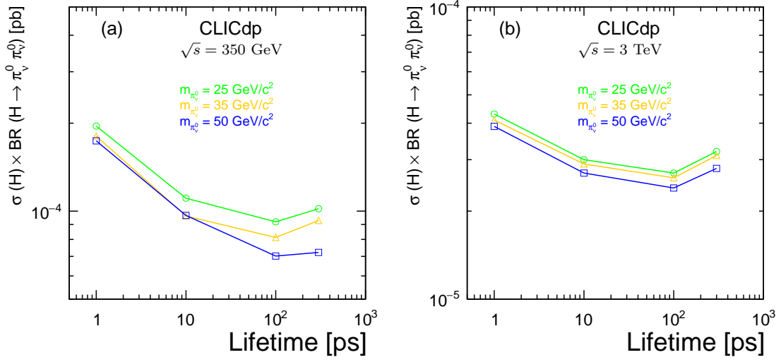
FIG. 41: Expected 95% CL cross-section upper limits on the \sigma(H) \times BR(H \rightarrow \pi_v^0 \pi_v^0) , within the model [374], for three different \pi_v^0 masses: 25 GeV (green), 35 GeV (yellow), 50 GeV (blue), as a function of \pi_v^0 lifetime for \sqrt{s} = 350 GeV (a) and \sqrt{s} = 3 TeV (b). Since physics is the same, sensitivities can be interpreted as the results at the CEPC with upgraded CM energies. Taken from Ref. [370].
