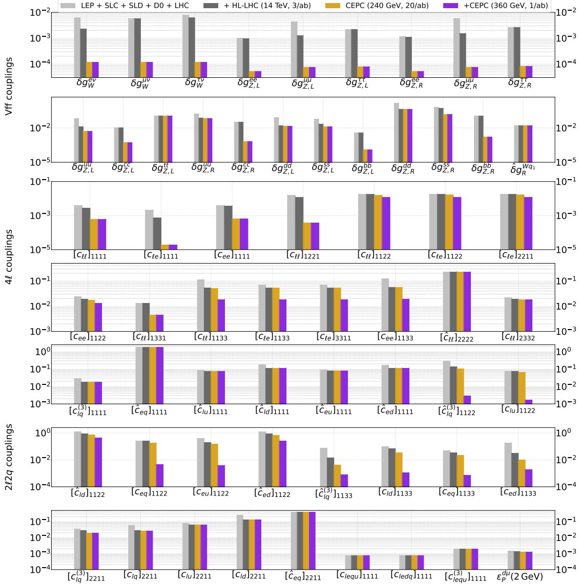
FIG. 94: Same as Fig. 93 but for the electroweak and 4-fermion operators.
