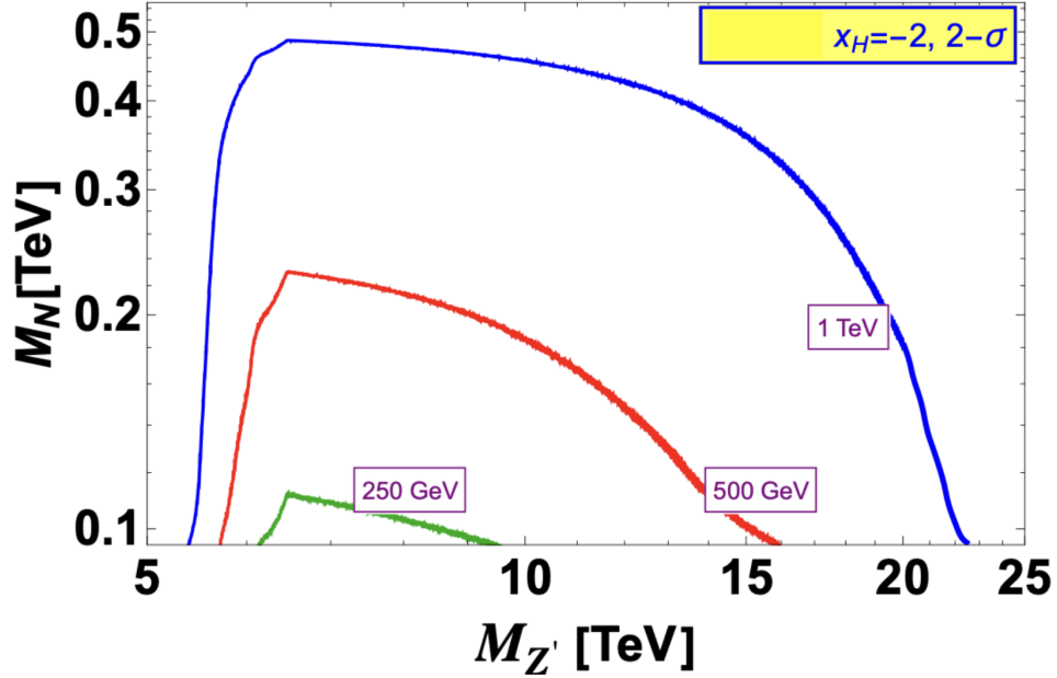
FIG. 75: 2\text{-}\sigma contour of the M_N - M_{Z'} plane at the electron-positron colliders at different center of mass energies studying same-sign dilepton plus four jet final states. Taken from Ref. [548]
