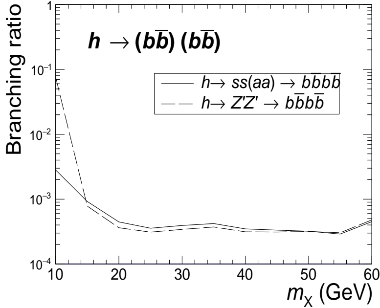
FIG. 8: The 95% C.L. exclusive bound on \text{Br}(h \rightarrow (\bar{b}b)(\bar{b}b)) , based on Ref. [33].
