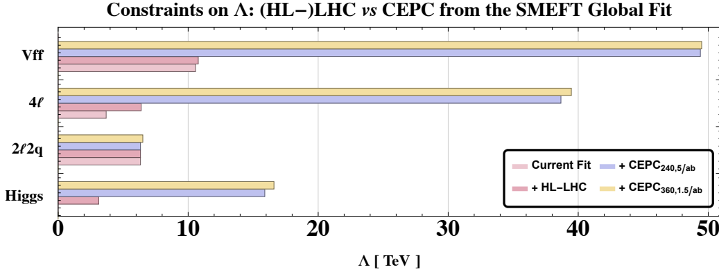
FIG. 95: Sensitivity to the cutoff scale \Lambda from the SMEFT global fit at the 95% CL. The y axis shows the optimal reach from electroweak physics (“Vff”), pure leptonic four-fermion operator induced physics (“4 \ell ”), semileptonic four-fermion operator induced physics (“2 \ell 2q”), and Higgs physics (“Higgs”).
