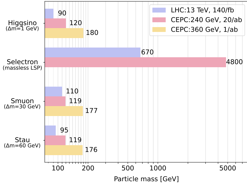
FIG. 66: The exclusion reaches for higgsino and slepton at CEPC and LHC. The compressed SUSY particles are picked for the comparison except for selectron.
