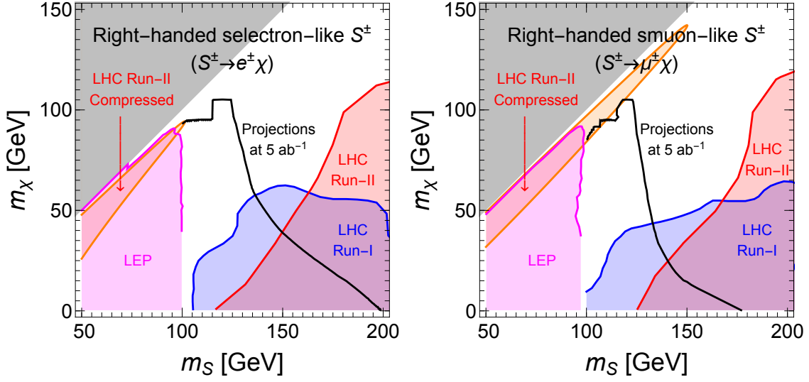
FIG. 24: Current constraints on right-handed selectron-like ( Left Panel ) and smuon-like ( Right Panel ) scalar S in the (m_{\text{DM}}, m_S) plane [45]. Black lines show CEPC projections at 5 \text{ ab}^{-1} from the Drell-Yan process e^+e^- \rightarrow S^{\pm(*)}S^\mp with S^\mp \rightarrow \ell^\mp \chi (allowing one off-shell S^{\pm(*)} ). Sensitivity extends to m_S > \sqrt{s}/2 = 120 \text{ GeV} via off-shell S^{\pm(*)} contributions. The
