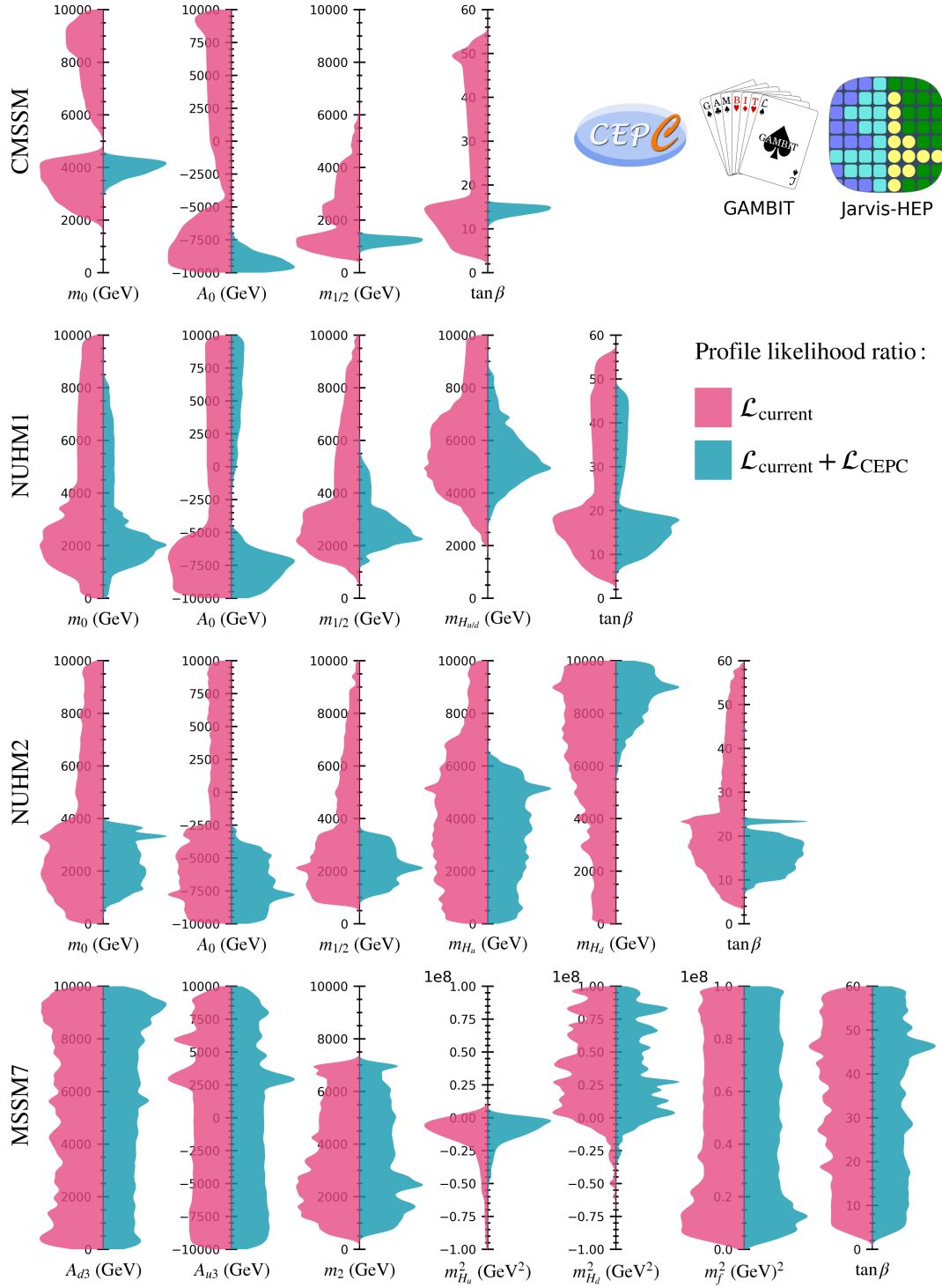
FIG. 99: One-dimensional profiled likelihood ratio for the global fit of the CMSSM, NUHM1, NUHM2, and MSSM7 models, using the present experimental data (left parts) and considering additional CEPC measurements (right parts).
