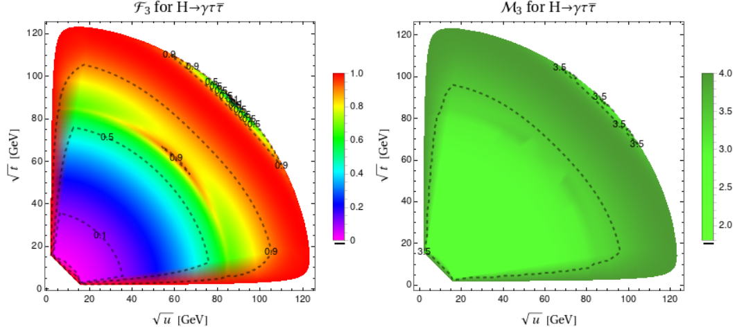
FIG. 90: Dalitz plot representation for genuine multipartite entanglement (left) and Bell non-locality (right) quantifiers for the SM Higgs boson's h \rightarrow \tau^+ \tau^- \gamma decay. The Mandelstam variables t and u correspond to the subsystems photon-lepton and photon-anilepton.
