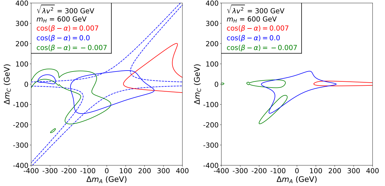
FIG. 98: Three-parameter fitting 95% C.L. range of \Delta m_A - \Delta m_C plane, focusing on the \cos(\beta - \alpha) dependence (given by different colored lines), for Higgs and Z -pole precision constraints individually (left panel), and combined constraints (right panel) in the Type-II 2HDM. More details are shown in Ref. [741].
