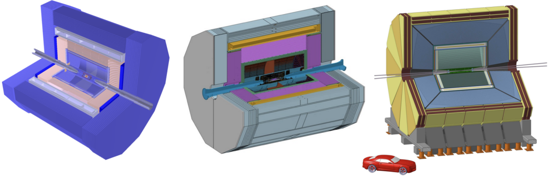
FIG. 3: Schematic layouts of LEFT: CEPC CDR detector [11], MIDDLE: Ref-TDR detector [20], and RIGHT: IDEA detector [21].
