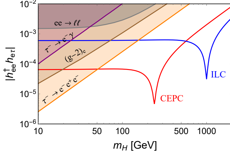
FIG. 80: Prospects of |h_{ee}^\dagger h_{e\tau}| from searches of e^+e^- \rightarrow e^\pm\tau^\mp , \mu^\pm\tau^\mp at CEPC (red, \sqrt{s} = 240 GeV, \mathcal{L} = 5 ab ^{-1} ) and ILC (blue, 1 TeV and 1 ab ^{-1} ). The shaded regions are excluded by current limits. Figure from Ref. [552].
