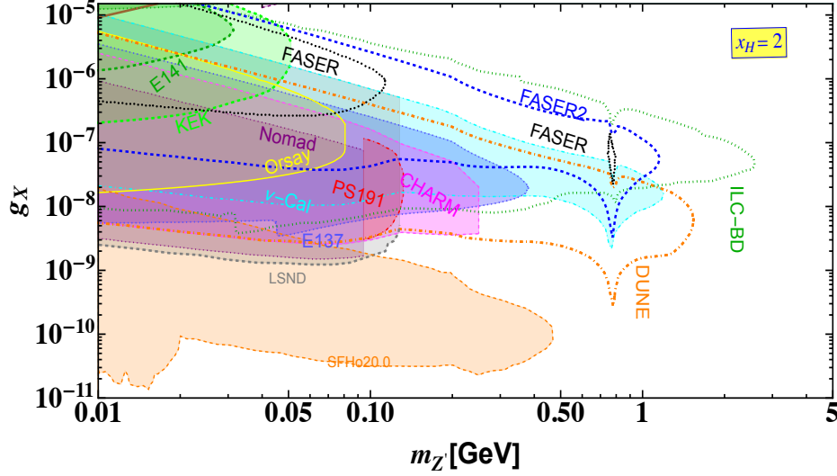
FIG. 57: Limits in the m_{Z'} - g_X plane for x_H > 0 and x_\Phi = 1 considering 10 MeV \leq m_{Z'} \leq 5 GeV, showing the regions that could be probed by FASER, FASER2, ILC-Beam dump, and DUNE. The parameter space is compared with existing bounds from different beam-dump experiments and a cosmological observation of supernova SN1987A (SFHo20.0), respectively. Taken from Ref. [418].
