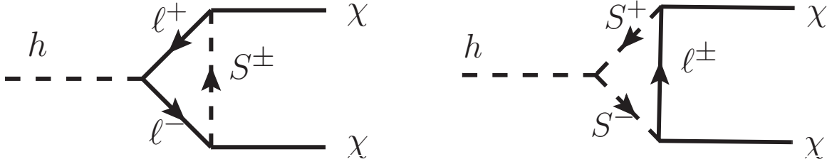
FIG. 11: The one-loop induced Higgs invisible decay (from Ref.[45]). The cross-diagrams for Majorana fermion \chi are not shown here but are included in the calculation.
