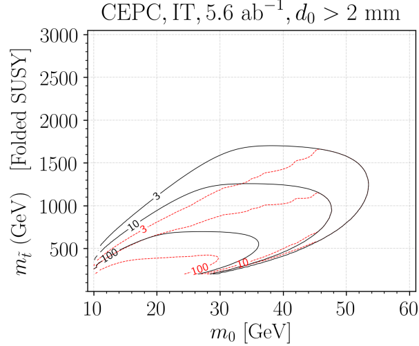
FIG. 39: Sensitivity reaches of \log_{10}(N_{\text{signal}}) at the CEPC for the Folded SUSY model.
