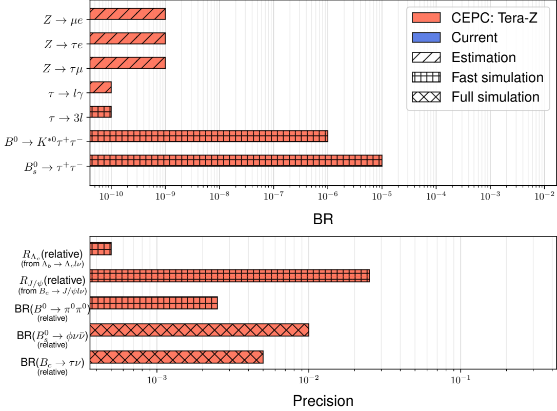
FIG. 68: Summary plot of relevant flavor physics probes at CEPC. The upper and lower parts of the plot correspond to the BR upper limits reached and the sensitivities of SM processes. The current limits of \tau \rightarrow 3\ell and \ell\gamma channels are taken as the best one among all lepton flavor combinations.
