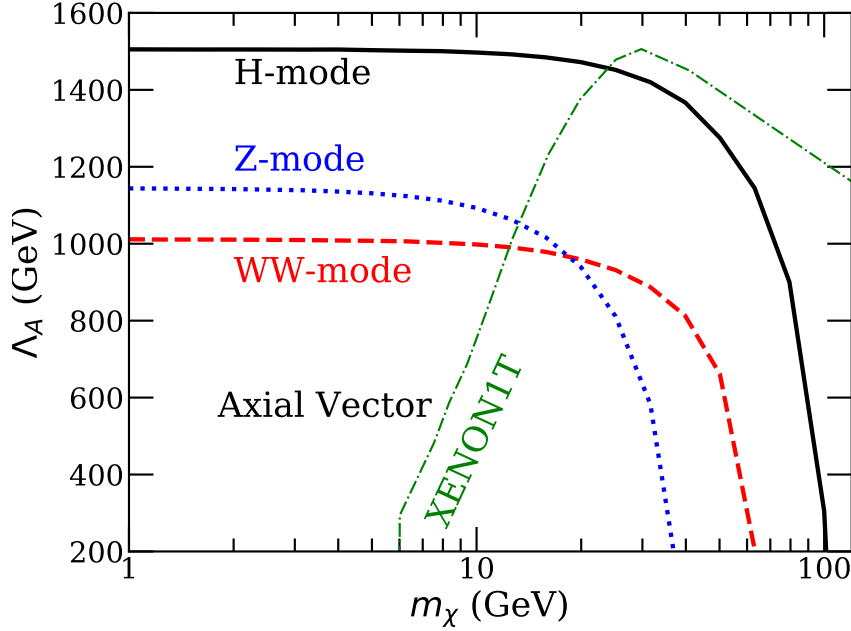
FIG. 31: Expected 95% CL constraints on \Lambda_A in the three CEPC running modes. Also shown are the Xenon1T constraints on \Lambda_A [311].
