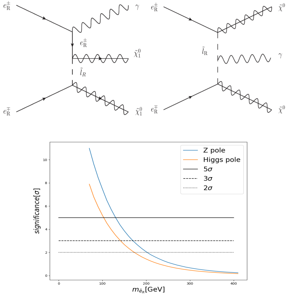
FIG. 63: Top: Representative diagram illustrating heavier selectron production. Bottom: Significance of exclusion ability.
