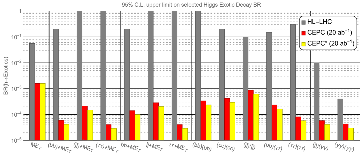
FIG. 7: The 95% C.L. upper limit on selected Higgs exotic decay branching fractions at HL-LHC and CEPC, based on Ref [33].
