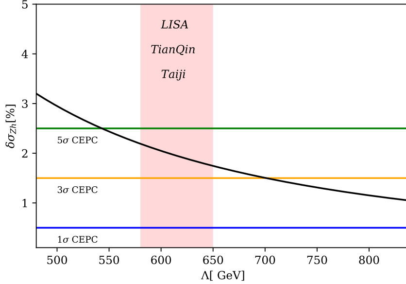
FIG. 20: The observational abilities of different experiments for the FOEWPT in the SMEFT.
