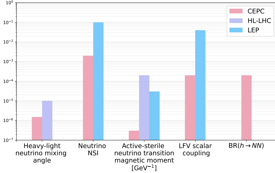
FIG. 83: Prospects of neutrino physics observables at the CEPC, in comparison with the LEP limits and LHC prospects. See text for more details.
