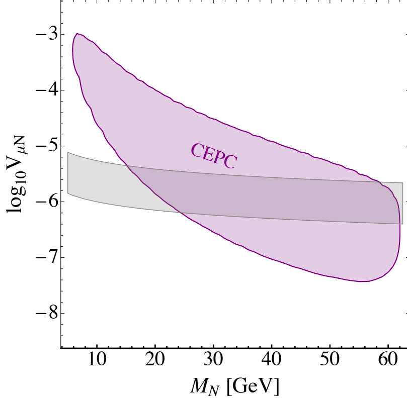
FIG. 74: Excluded regions in the (M_N, V_{\mu N}) parameter space at 95% CL assuming no observation of a single displaced vertex for the 20 \text{ ab}^{-1} CEPC (purple). The grey band indicates the parameter region where a light neutrino mass in the interesting range is generated, 0.01 \text{ eV} < m_\nu = |V_{\mu N}|^2 m_N < 0.3 \text{ eV} . We fix the Higgs-BSM mixing \sin \alpha = 0.3 . Adapted from Ref. [547].
