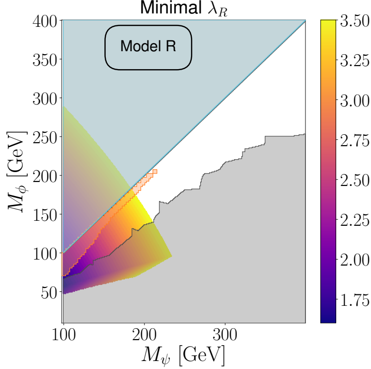
FIG. 88: A simplified BSM scenario with a scalar and a fermion. The color-coding shows the minimal coupling to right-handed muons to explain the muon g - 2 . Outside of this colored region, the muon g - 2 cannot be explained within 1\sigma . The shaded grey region shows the LHC exclusions and the shaded orange region is excluded by compressed spectra. The shaded blue region (top left) is excluded due to a charged stable particle.
