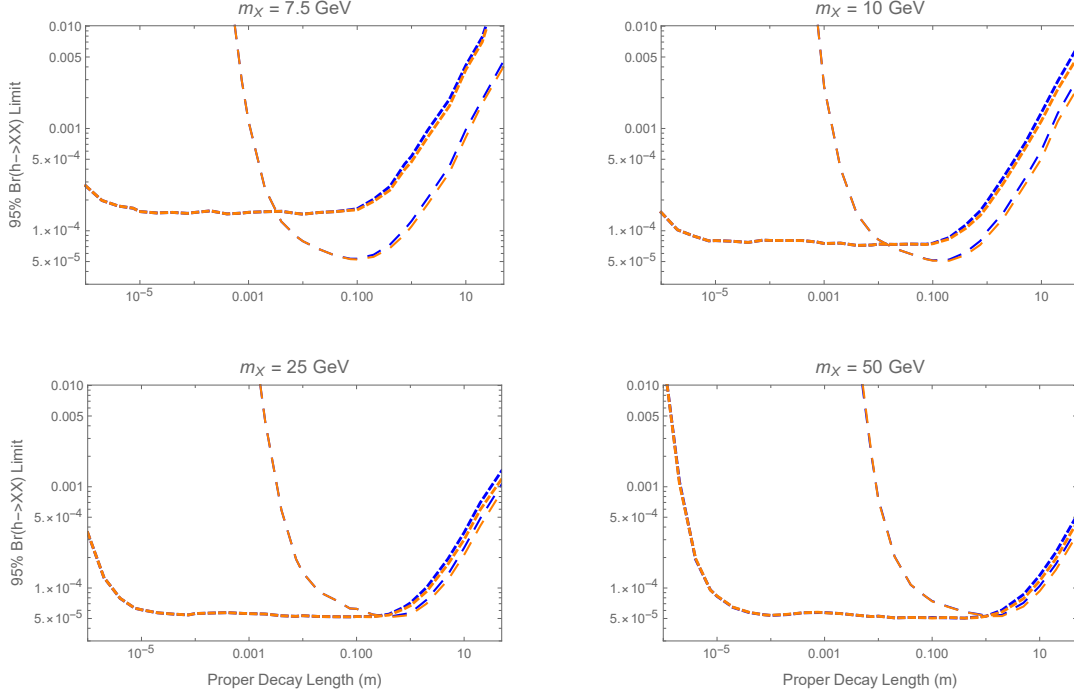
FIG. 38: Projected 95% h \rightarrow XX branching ratio limits as a function of proper decay length for a variety of X masses. Blue lines are for CEPC and orange lines are for FCC-ee, and where only one is visible they overlap. The larger dashes are the ‘long lifetime’ analysis and the smaller dashes are the ‘large mass’ analysis. Taken from Ref. [70].
