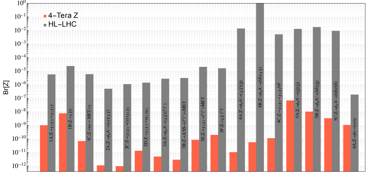
FIG. 10: The reach for the branching ratio of various exotic Z decay modes at the future Z -factories (rescaled to four Tera Z ) and the HL-LHC at 13 TeV with \mathcal{L} = 3 \text{ ab}^{-1} [61]. The sensitivities, in general, generally also depend on model parameters, such as the masses of the mediator and dark matter. In this figure, we take the best case for each category.
