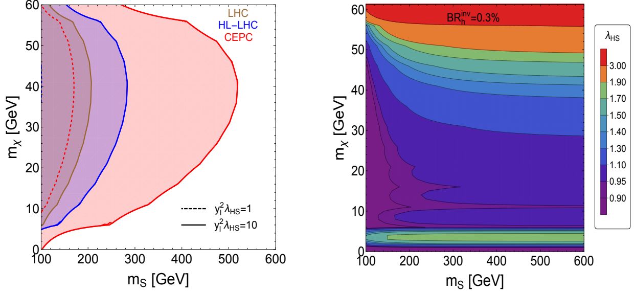
FIG. 12: Left : The Higgs portal coupling \lambda_{HS} (Eq. 3) and the fermion portal coupling y_\ell (Eq. 2) can induce the Higgs invisible decay h \rightarrow \bar{\chi}\chi at one-loop level. Constraints on the coupling combination y_\ell^2 \lambda_{HS} are derived from searches for invisible Higgs decays at the LHC, HL-LHC ( \text{BR}_{h \rightarrow \text{inv}} < 3.5\% ), and CEPC ( \text{BR}_{h \rightarrow \text{inv}} < 0.3\% ). The recent CEPC Technical Design Report (TDR) [12] projects an improved limit of \text{BR}_{h \rightarrow \text{inv}} < 0.07\% with an upgraded integrated luminosity of 20 \text{ ab}^{-1} during Higgs operation, which could further tighten the bound on y_\ell^2 \lambda_{HS} by a factor of two. Right : For each mass point (m_S, m_\chi) , the fermion portal coupling y_\ell is set to its thermal value y_\ell^{\text{th}} , as required by the observed dark matter relic abundance. Constraints on the Higgs portal coupling \lambda_{HS} are then derived using the CEPC limit on the invisible Higgs branching fraction \text{Br}(h \rightarrow \text{inv}) < 0.3\% .
