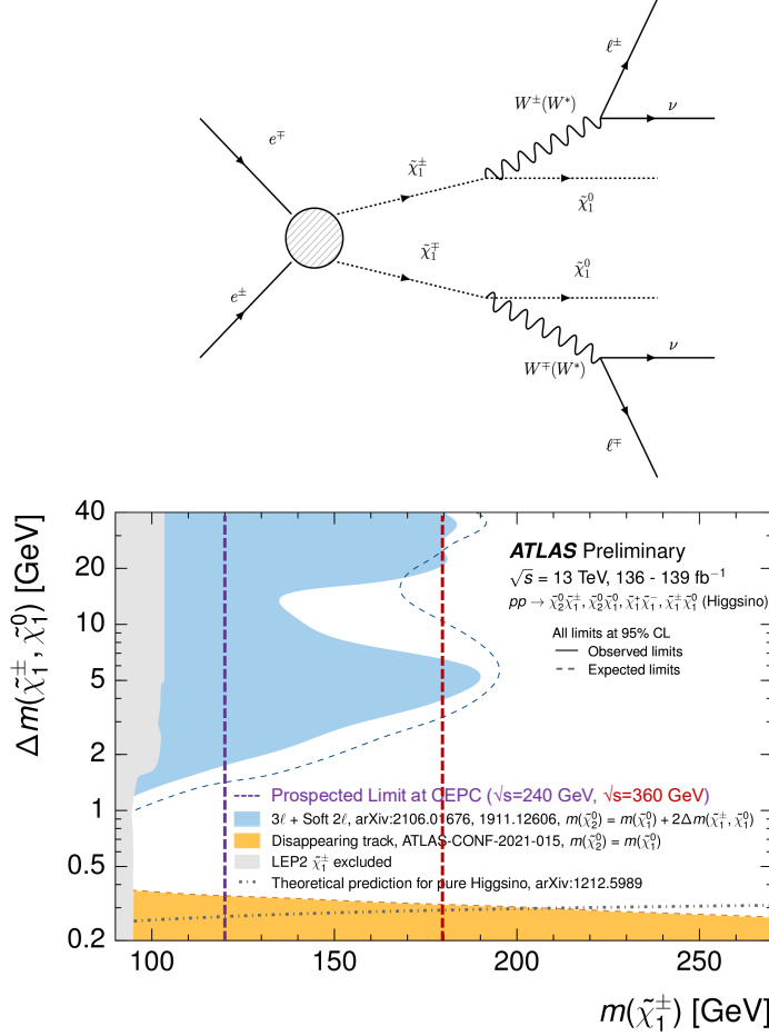
FIG. 60: Top : Representative diagram for the pair production of charginos and subsequent decay into a dilepton final states. Bottom : Projected limits at the CEPC (purple dotted) in comparison ATLAS observed and expected exclusion limits on simplified SUSY models for chargino-pair production with Higgsino-like LSP. The observed limits from the LEP are shown in light grey.
