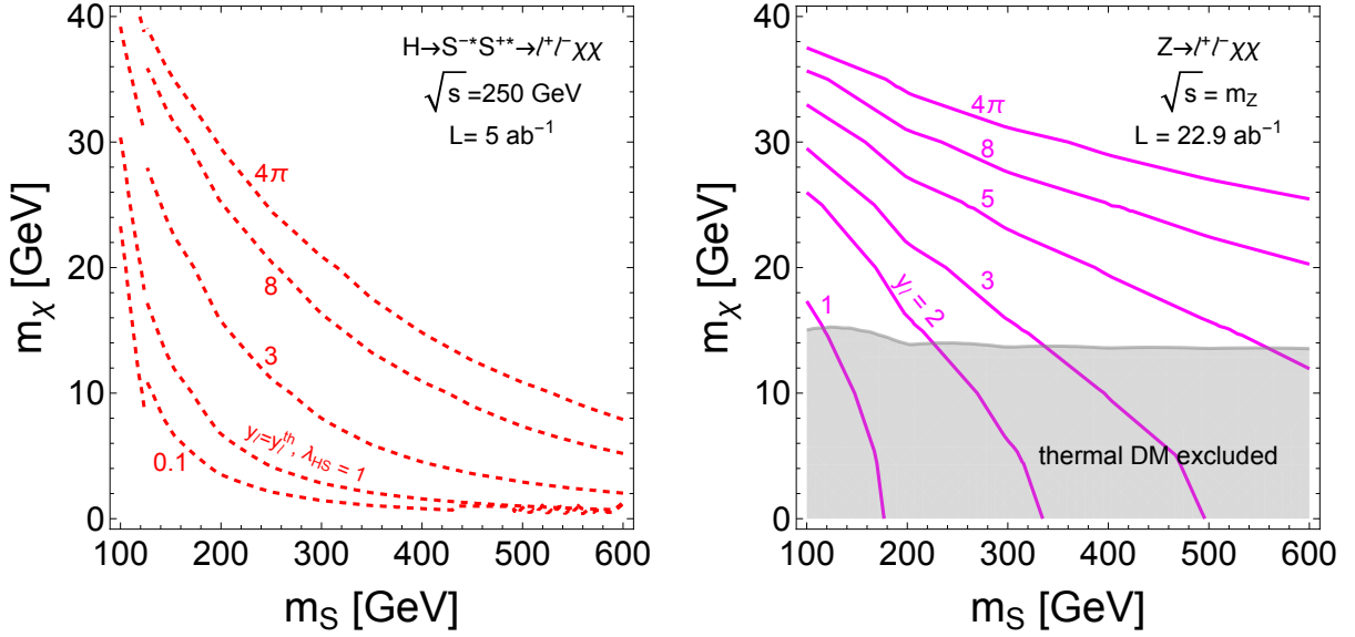
FIG. 9: Left: The Higgs exotic decay h \rightarrow S^{+(*)} S^{-(*)} \rightarrow \ell^+ \chi \ell^- \chi , mediated by off-shell charged scalars S^\pm , probes the Higgs portal coupling \lambda_{HS} (Eq. 3) and the Fermion portal coupling y_\ell (Eq. 2). Since the cross section for the DM annihilation process \bar{\chi}\chi \rightarrow \ell^+ \ell^- scales as y_\ell^4 , we fix y_\ell = y_\ell^{\text{th}} to satisfy the thermal DM relic abundance for each point in the (m_S, m_\chi) 2D plane. The dashed red lines correspond to fixed values of \lambda_{HS} , with the lower-left corner of each line excluded by the Higgs exotic decay search h \rightarrow S^{\pm(*)} S^{\mp(*)} \rightarrow \ell^+ \chi \ell'^- \chi . Right: The exotic Z boson decay Z \rightarrow \ell^+ \chi \ell^- \chi , dominantly mediated by an off-shell S^\pm attached to the external charged lepton leg, probes the fermion portal coupling y_\ell (Eq. 2). The magenta contours show the 95% C.L. limits on y_\ell for each point in the (m_S, m_\chi) plane, derived from exotic Z \rightarrow \ell^+ \ell^- + \cancel{E} searches at a Tera- Z factory. For each mass configuration, the corresponding y_\ell is used to compute the thermal DM relic density, with the gray shaded region excluded by relic abundance constraints. Figures taken from Ref. [45].
