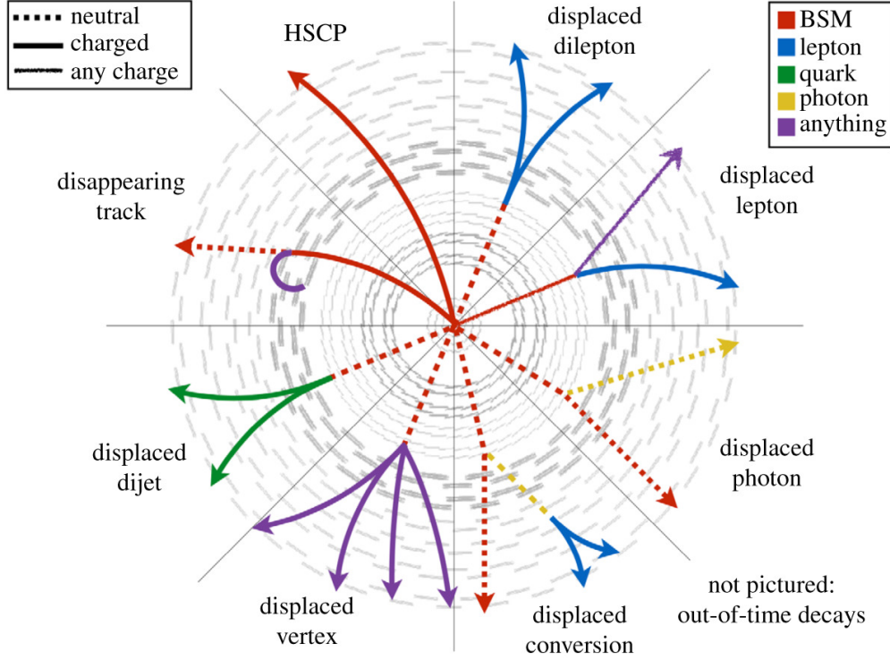
FIG. 36: Typical LLP signatures at the MD of a collider. Taken from Ref. [349].
