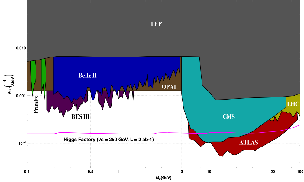
FIG. 84: Summary plot of the sensitivity to g_{a\gamma\gamma} that can be achieved at e^+e^- collider with \sqrt{s} = 250 GeV and an integrated luminosity 2 \text{ ab}^{-1} . Other existing constraints are also shown for comparison.
