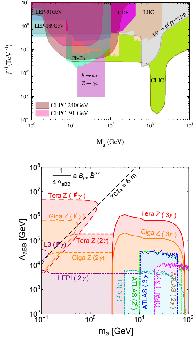
FIG. 85: Top panel: 95 C.L. sensitivity regions on the ALP coupling g_{a\gamma\gamma} as a function of M_a for the process e^+e^- \rightarrow \gamma\gamma e^+e^- at the 91 and 240 GeV runs of the CEPC. Bottom panel: sensitivity to the axion's coupling to the SM U(1)_Y hypercharge field at Z-factory.
