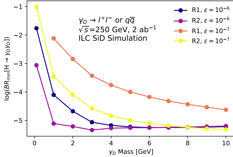
FIG. 42: The minimum branching ratio H \rightarrow \gamma_D \gamma_D to which SiD will be sensitive for \sqrt{s} = 250 GeV and 2 \text{ ab}^{-1} , when both leptonic and hadronic decays are reconstructed within the regions R1 and R2 , for \epsilon = 10^{-6}, 10^{-7} . Since physics is similar, sensitivities can be interpreted as the results at the CEPC with the same CM energy and integrated luminosity. Taken from Ref. [72].
