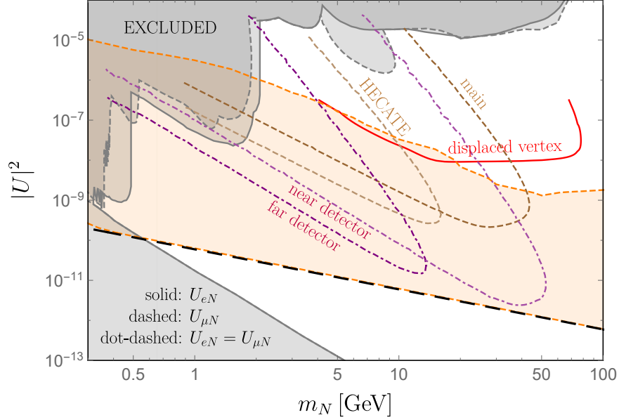
FIG. 69: Summary of prospects of heavy neutrino mass m_N and the heavy-light neutrino mixing |U|^2 at the CEPC. The solid lines are for U_{eN} : displaced vertex (red) [543]. The dashed lines are for U_{\mu N} : main detector and HECATE (darker and lighter brown) [407]. The dot-dashed lines are for U_{eN} = U_{\mu N} : main detector (near detector) and far detectors (lighter and darker purple) [75]. All the shaded regions are excluded by current limits, with solid for U_{eN} and dashed for U_{\mu N} [544]. The long dashed black line indicate the parameter space for the seesaw mechanism, while the shaded orange region is favored by the leptogenesis mechanism [545].
