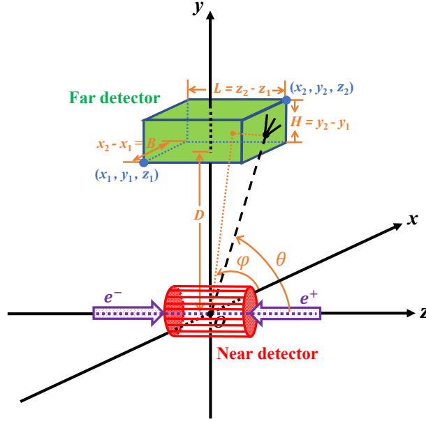
FIG. 47: The sketch displays the main detector (near detector, abbreviated as ND) and an example far detector. The dashed line indicates that one LLP is produced at the IP, travels through the main detector and decay inside the far detector. Taken from Ref. [75].
