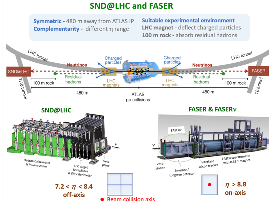
FIG. 45: Schematic pictures of the SND@LHC, FASER \nu , and FASER experiments. Taken from Ref. [386].
