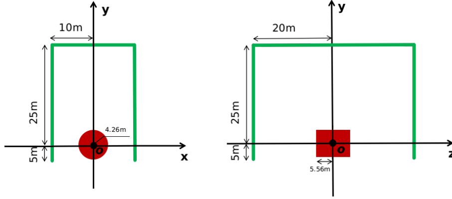
FIG. 48: The left and right plots show section views of the experimental setup in the xOy and yOz planes, respectively. In the plots, the red cylinder enclosing the coordinate origin represents the main detector of CEPC/FCC-ee. The green area depicts the proposed new far detector, LAYCAST, in the shape of a thin layer to be instrumented on the cavern surface. Take from Ref. [368].
