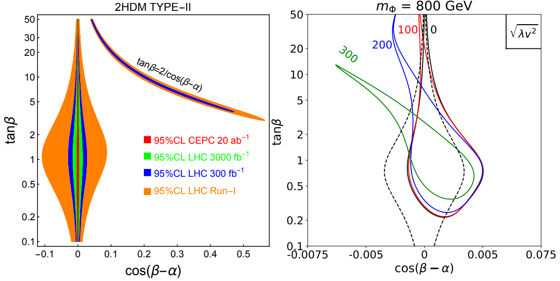
FIG. 97: The allowed region in the plane of \cos(\beta - \alpha) - \tan \beta at 95% C.L. for the Type-II of 2HDM, given LHC and CEPC Higgs precision measurements at tree level (left) and loop level under CEPC (right). For the tree-level global fit, the special “arm” regions for the Type-II is the wrong-sign Yukawa region. The right panel shows the parameter space varying the value \sqrt{\lambda v^2} with m_A = m_H = m_{H^\pm} = m_\Phi = 800 \text{ GeV} . The tree-level only global fit results are shown by the dashed black lines for comparison. More details are shown in Ref. [580].
