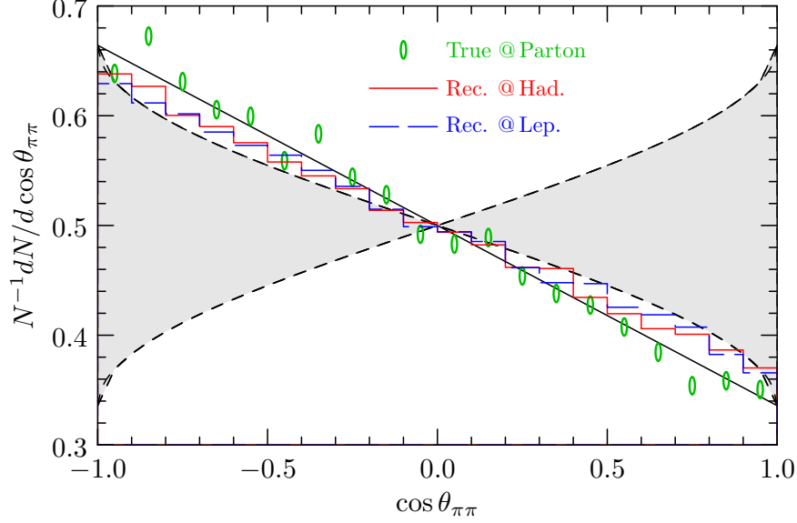
FIG. 89: Reconstructed distributions of \cos \theta_{\pi\pi} for Törnqvist's test of Bell inequality with h \rightarrow \tau^+\tau^- at the CEPC Higgs factory mode. 1\sigma test sensitivity is projected at the CEPC, represented by the red and blue histograms for hadronic and leptonic decay modes of Z boson, respectively. The gray-fitted region is the phase space consistent with classical prediction.
