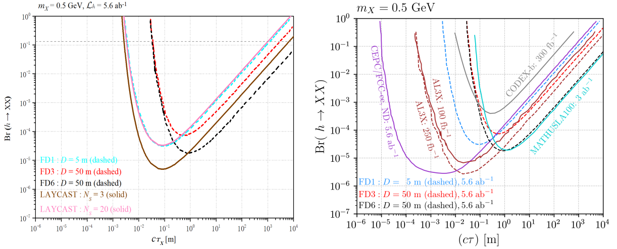
FIG. 50: Left: Sensitivity reaches of the CEPC/FCC-ee's far detectors FD1, FD3, FD6 and LAYCAST in the \text{Br}(h \rightarrow XX) vs. c\tau plane for m_X = 0.5 GeV. Right: Sensitivity reaches of the CEPC/FCC-ee's far detectors FD1, FD3, FD6, compared with predictions for the CEPC/FCC-ee's main detector (near detector, abbreviated as ND) and for AL3X, CODEX-b and MATHUSLA100. Taken from Ref. [75, 368].
