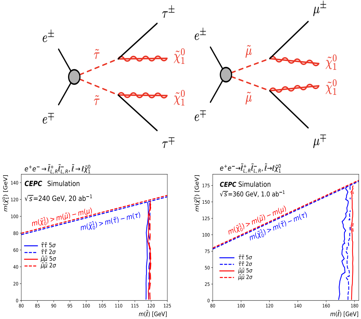
FIG. 62: Top : representative diagram illustrating the pair production of charged staus (smuons) and subsequent decay into a two-tau (two-muon) final state. Bottom : The 5σ discovery contour (solid line) and 2σ exclusion contour (dashed line) for the direct stau production and direct smuon production with 5% flat systematic uncertainty. Left (Right) plot presents the center-of-mass energy of 240 (360) GeV.
