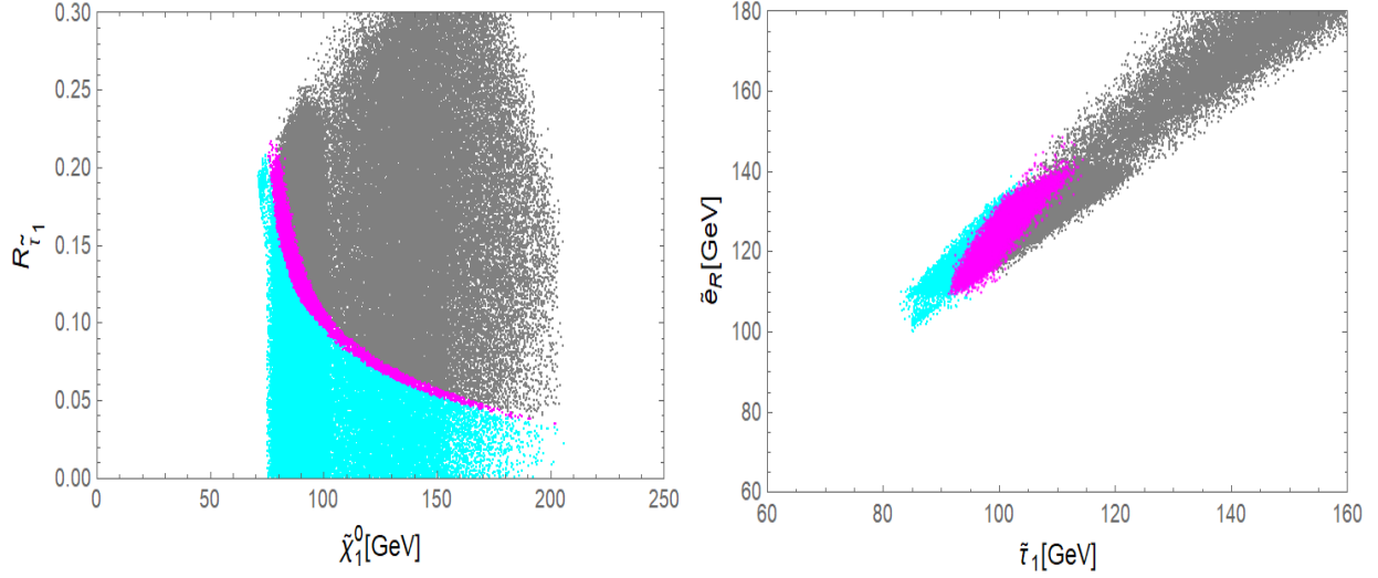
FIG. 65: Left: Bulk region in Generalized No-Scale \mathcal{F} - SU(5) . Right: Light right-handed slepton masses in this bulk region. Cyan, magenta, and gray points correspond to under-saturated, saturated, and over-saturated DM relic density.
