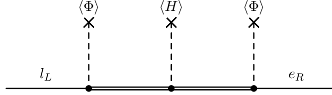
FIG. 91: A Feynman diagram which generates the charged lepton mass matrix. Plain lines represent the Standard Model charged leptons. Double lines represent heavy fermions. Dashed lines represent Higgs tadpoles as labeled.
