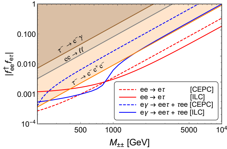
FIG. 81: Prospects of the Yukawa couplings |f_{ee}^\dagger f_{e\tau}| for the doubly-charged scalar H^{\pm\pm} production via the e^+e^- \rightarrow e\tau (red) and e^-\gamma \rightarrow e^+e^-\tau^- + \tau^+e^-e^- (blue) processes, at CEPC with \sqrt{s} = 240 GeV and an integrated luminosity of 5 ab ^{-1} (dashed) and ILC with \sqrt{s} = 1 TeV and 1 ab ^{-1} (solid). The shaded regions are excluded by current limits. Figure from Ref. [553].
