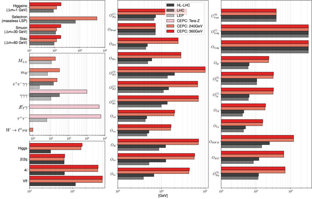
FIG. 101: The typical energy scale of New Physics that could be probed at the CEPC. The left column corresponds to a specialized New Physics Model of SUSY, and exotic New Physics signal searches, including Axion-like particles, and scalar particles in seesaw Models. The middle and right columns correspond to New Physics search via EFT.
