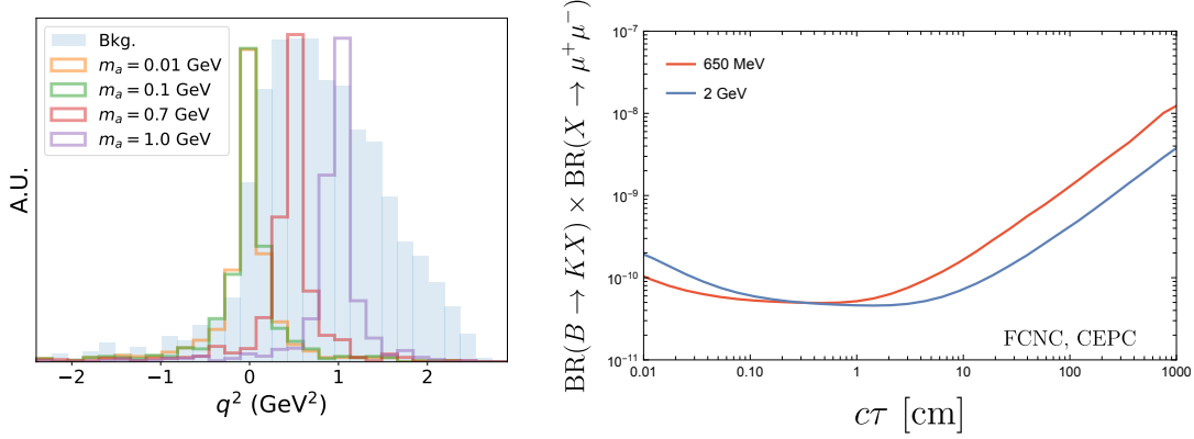
FIG. 67: Left: Reconstruction of invisible particle mass squared q^2 \equiv (p_\tau - p_\mu)^2 from \tau decays to \mu and an invisible BSM particle. Right: Projected sensitivity on FCNC B \rightarrow K X_{\text{LLP}}(\rightarrow \mu^+ \mu^-) as a function of X_{\text{LLP}} lifetime. Two mass benchmarks are shown as blue and red curves, respectively. Both plots are taken from [479].
