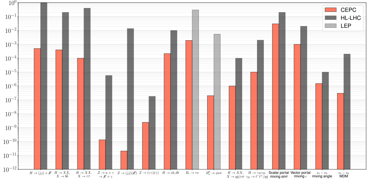
FIG. 100: Projected sensitivities of the CEPC and HL-LHC for various new physics scenarios, including exotic Higgs (first three categories) and Z -boson decays (categories 4-6), flavor-violating Higgs and B -meson decays (categories 7-9), long-lived particle searches (categories 10-11), scalar and vector portal mixing (categories 12-13), as well as sterile-active neutrino mixing and magnetic dipole moment interactions (last two categories). For flavor-violating B -meson decay channels, there are existing constraints from LEP only.
