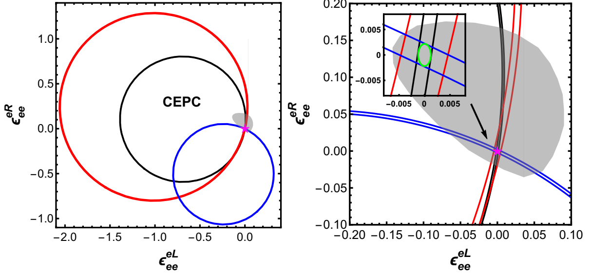
FIG. 77: Left panel: The allowed 90% C.L. region for electron-type neutrino NSI in the planes of (\epsilon_{ee}^{eL}, \epsilon_{ee}^{eR}) at future CEPC with 5.6 \text{ ab}^{-1} data of \sqrt{s} = 240 \text{ GeV} (Black), with 2.6 \text{ ab}^{-1} data of \sqrt{s} = 160 \text{ GeV} (Red), and with 16 \text{ ab}^{-1} data of \sqrt{s} = 91.2 \text{ GeV} (Blue), respectively. The allowed 90% C.L. regions arising from the global analysis of the LEP, CHARM, LSND, and reactor data [586], are shown in the shaded gray regions. Right panel: With all the data collected in all three running modes, the combined result is shown as the green region. Figure from Ref. [550]
