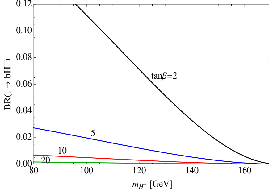
FIG. 14: \text{Br}(t \rightarrow bH^+) for \tan \beta = 2 (black), 5 (blue), 10 (red), 20 (green). The t decay into H^+ is larger for smaller m_{H^\pm} and smaller \tan \beta , from Ref.[88].
