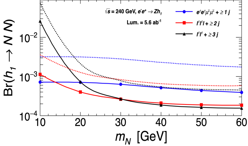
FIG. 73: The projected CEPC sensitivities to the decay branching ratio of h \rightarrow NN for 2-4 \ell channels at \sqrt{s} = 240 GeV with a luminosity of 5.6 \text{ ab}^{-1} . The 2\sigma and 5\sigma sensitivities are shown as the solid and dashed lines, respectively. Adapted from Ref. [546].
