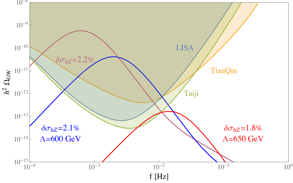
Fig. 21: General prediction of hZ cross section deviation to SM and its corresponding GW signals in the SMEFT under the condition of FOEWPT [184, 195].
