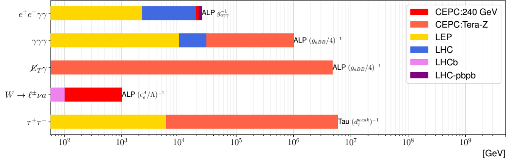
FIG. 92: Energy reach in representative exotic search channels at the CEPC. Note the maximal reach may apply to different parameter regions between experiments.
