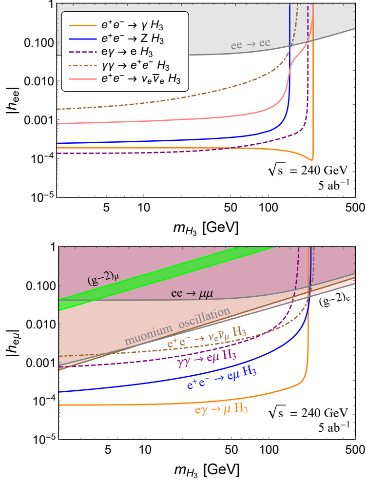
FIG. 79: Prospects of the couplings |h_{ee}| (top) and |h_{e\mu}| (bottom) from the on-shell production of H_3 at CEPC (240 GeV and 5 \text{ ab}^{-1} ), in the channels of e^+e^- \rightarrow (\gamma/Z)H_3 , e\gamma \rightarrow \ell H_3 , e^+e^- , \gamma\gamma \rightarrow \ell_\alpha^\pm \ell_\beta^\mp H_3 and e^+e^- \rightarrow \nu \bar{\nu} H_3 . The shaded regions are excluded by current limits, while the yellow band corresponds to the muon g - 2 discrepancy at 2\sigma C.L.
