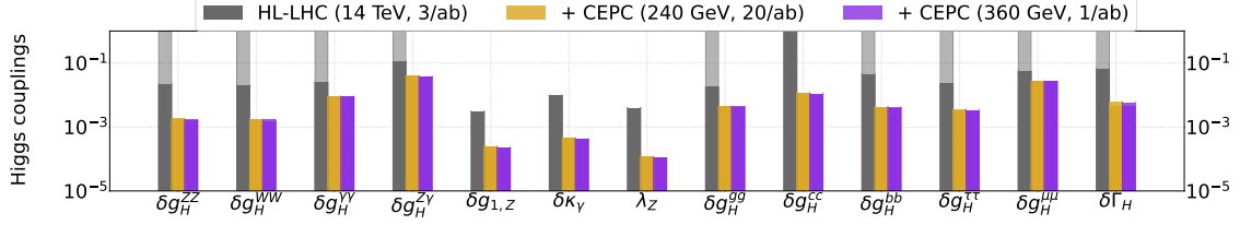
FIG. 93: 1\sigma relative uncertainties on the SMEFT operators as shown along the horizontal axis from a global analysis of the Higgs couplings. The light bars are obtained by taking the total Higgs decay width \Gamma_H as a free parameter, and the dark bars those with a constrained \Gamma_H .
