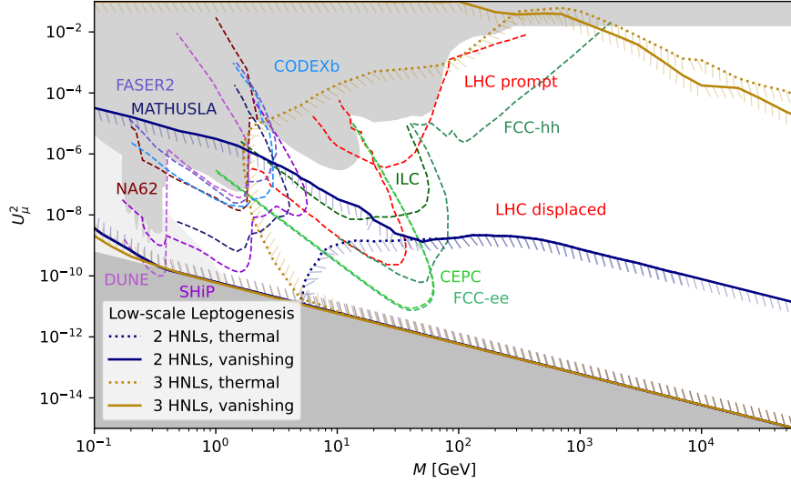
FIG. 82: Theoretical predictions of the HNL mass M and the ranges of U_\mu^2 in the framework of leptogenesis, with two or three HNL flavours in the case of NO, for both vanishing and thermal initial HNL abundances. The shaded region in gray is excluded by existing limits. complemented by the updated BBN bounds (light gray) and the lower bound from the seesaw mechanism (darker gray) [624–626]. The colored lines indicate prospects at existing and future experiments. Adapted from Ref. [545].
