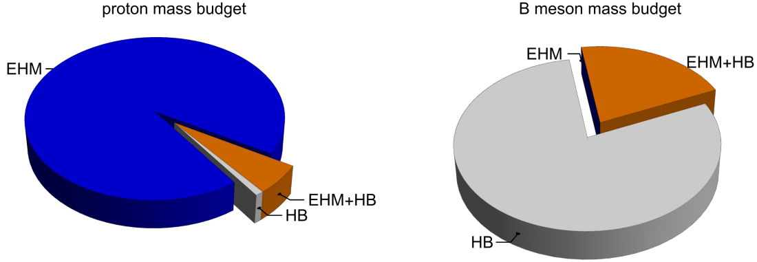
FIG. 87: Poincaré-invariant decompositions of hadron masses: (A) proton; (B) B -meson. EHM is the source of 94% of the proton mass; by itself, the HB accounts for just 1%; and the remaining 5% is generated by constructive EHM+HB interference. In stark contrast, EHM alone produces none of the B -meson mass. Instead, the HB is responsible for 79%; yet, there is a sizeable EHM+HB interference term. See Refs. [671, 672] for details.
