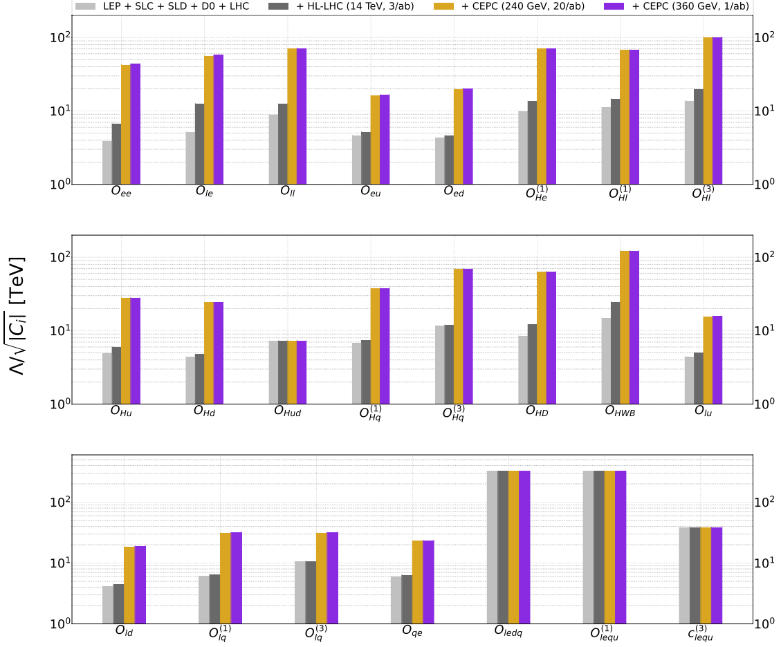
FIG. 96: Lower bounds on \Lambda/\sqrt{|C_i|} at the 95% CL as presented in the Warsaw basis, assuming flavor universality and one operator at a time.
