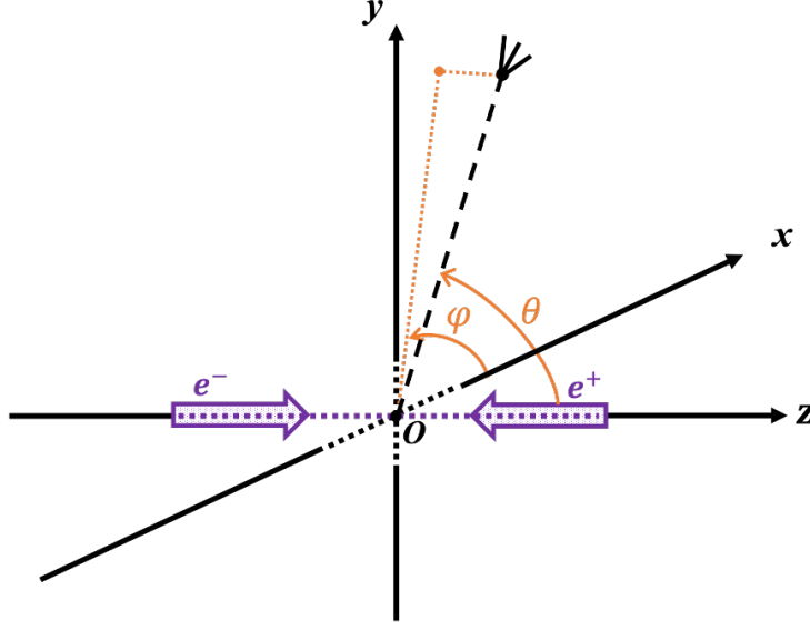
FIG. 35: Sketch of the production and decay of a LLP at electron-positron colliders.
