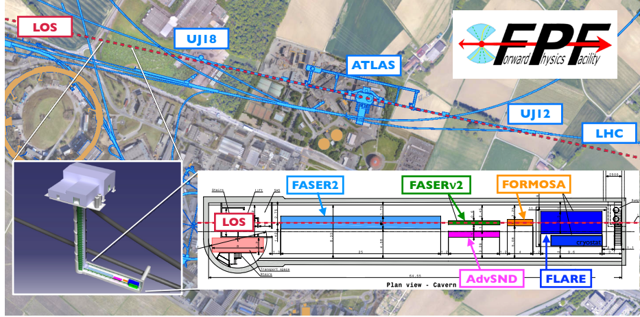
FIG. 46: The preferred location for the FPF, a proposed new cavern for the HL-LHC era. The FPF will be 65 m-long and 8.5 m-wide and will house a diverse set of experiments to explore the many physics opportunities in the far-forward region. Taken from Ref. [391].
