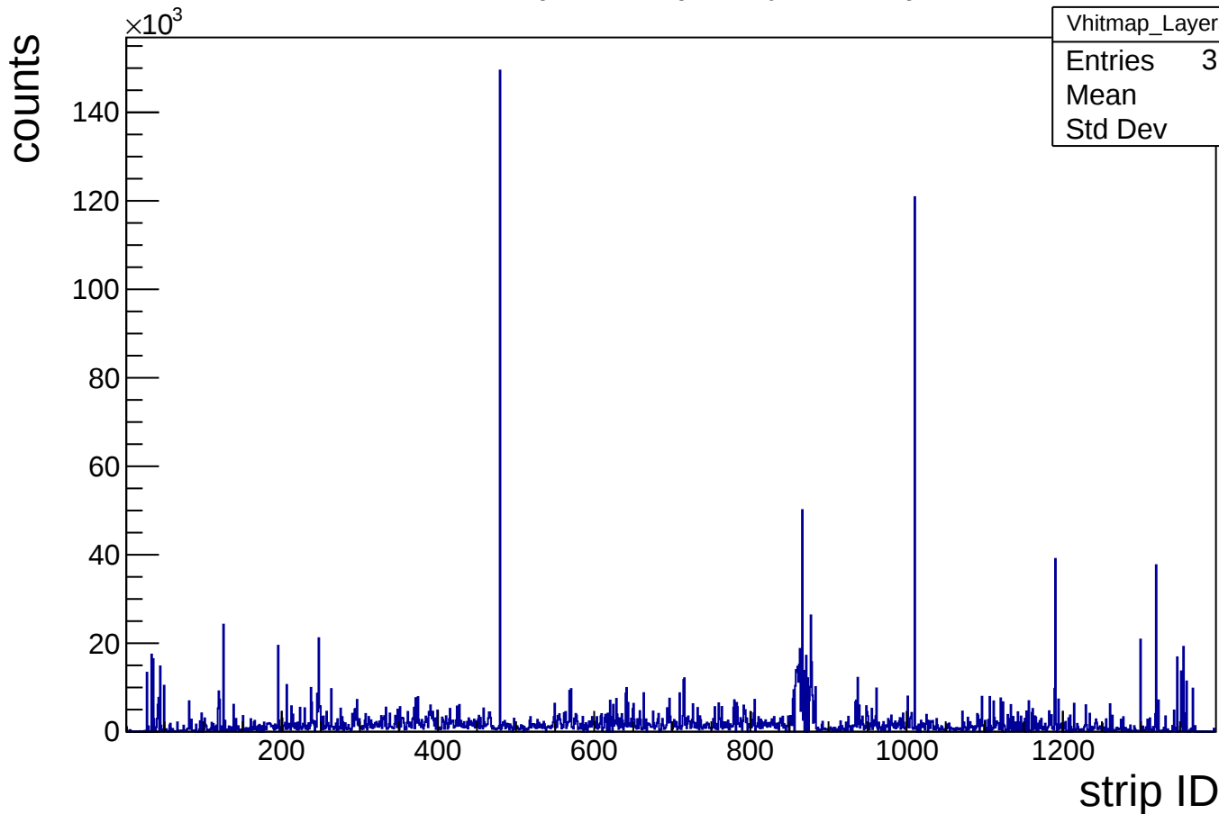
hit map, V strip, Layer3, top
