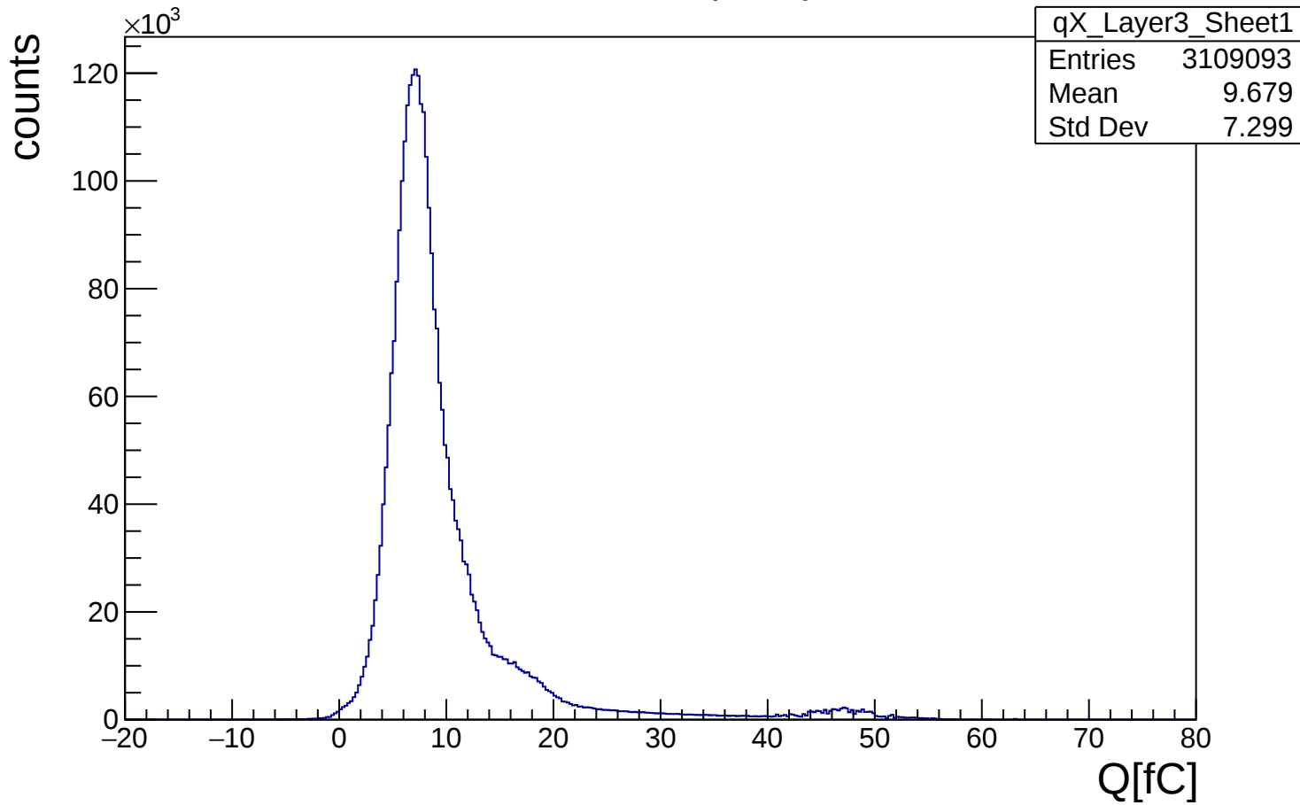
distribution of Q, X strip, Layer3, bottom
