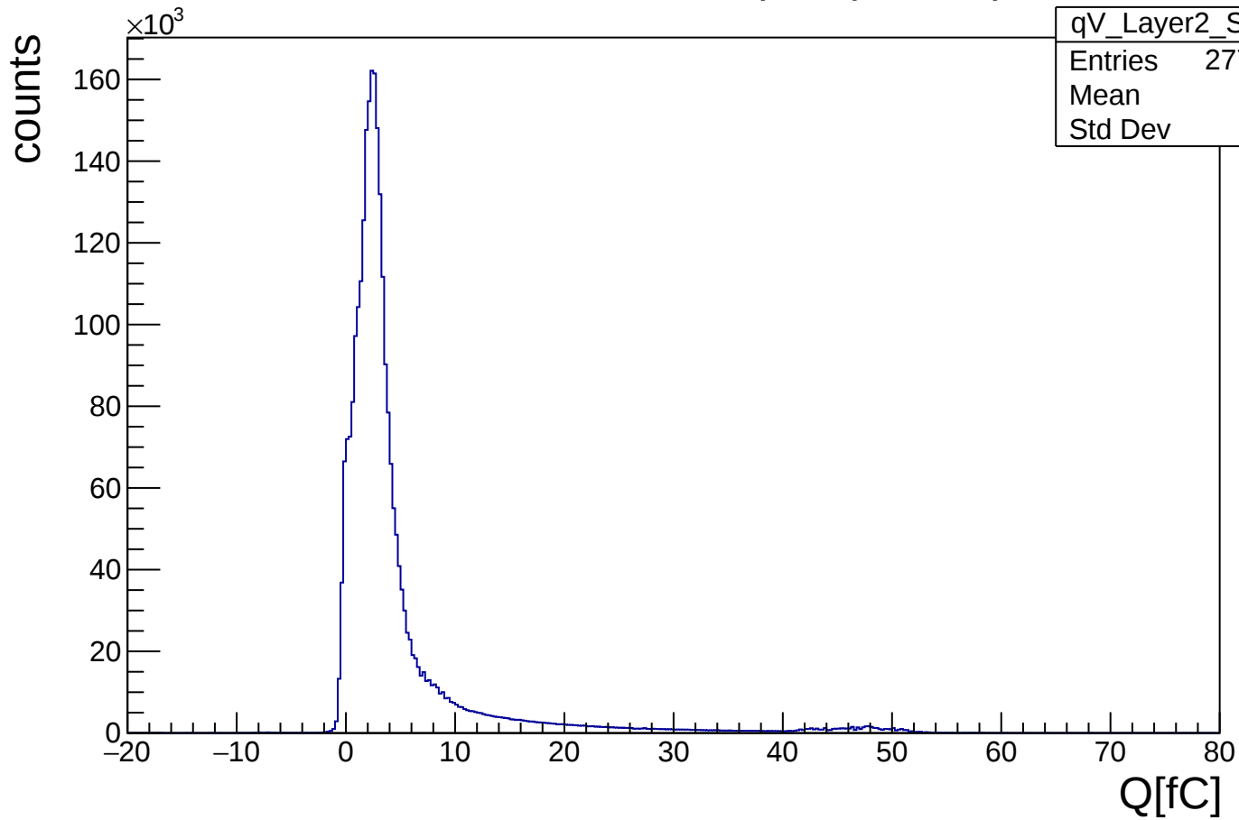
distribution of Q, V strip, Layer2, top
