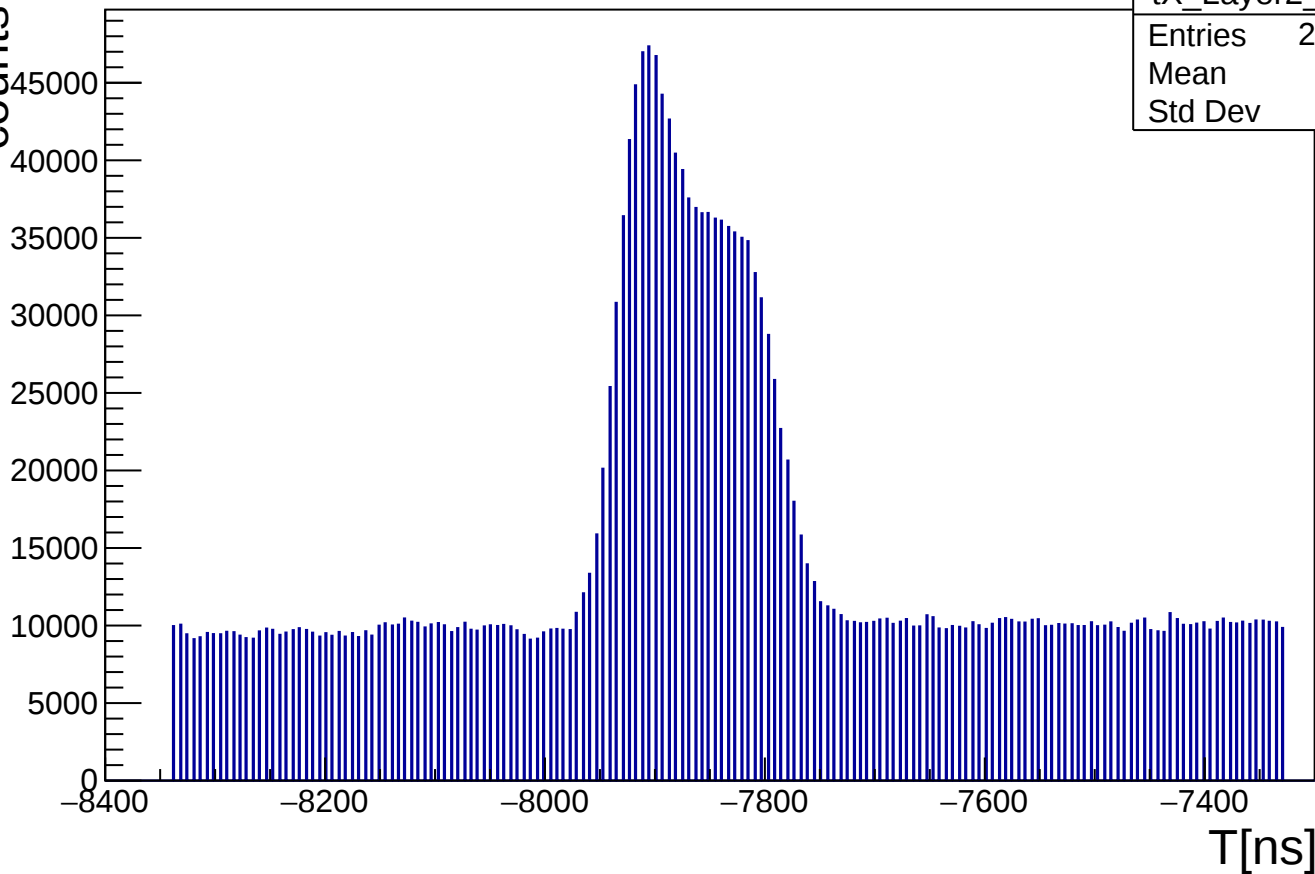
distribution of T, X strip, Layer2, bottom
