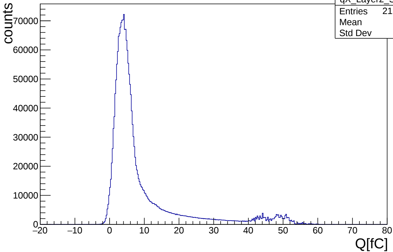
distribution of Q, X strip, Layer2, top
