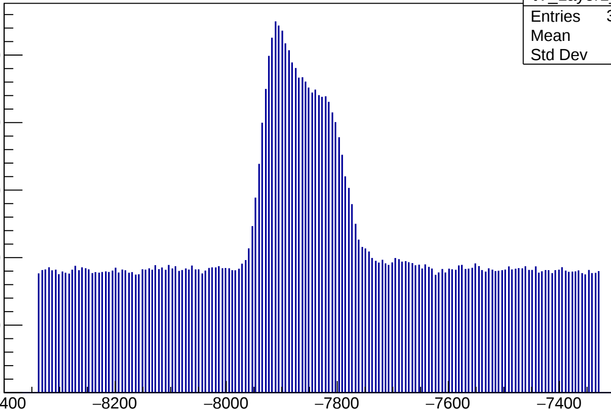
distribution of T, V strip, Layer1
