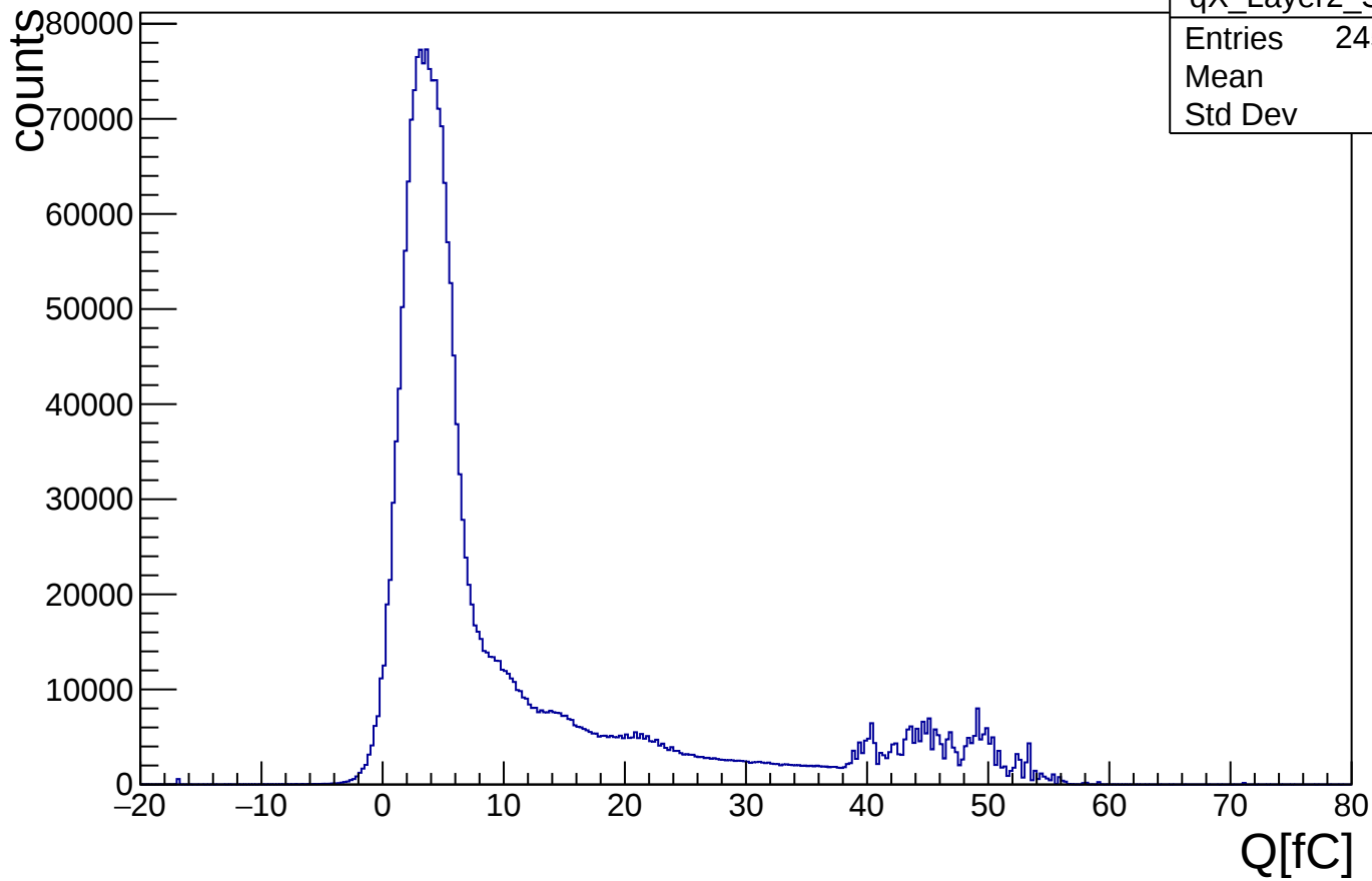
distribution of Q, X strip, Layer2, bottom
