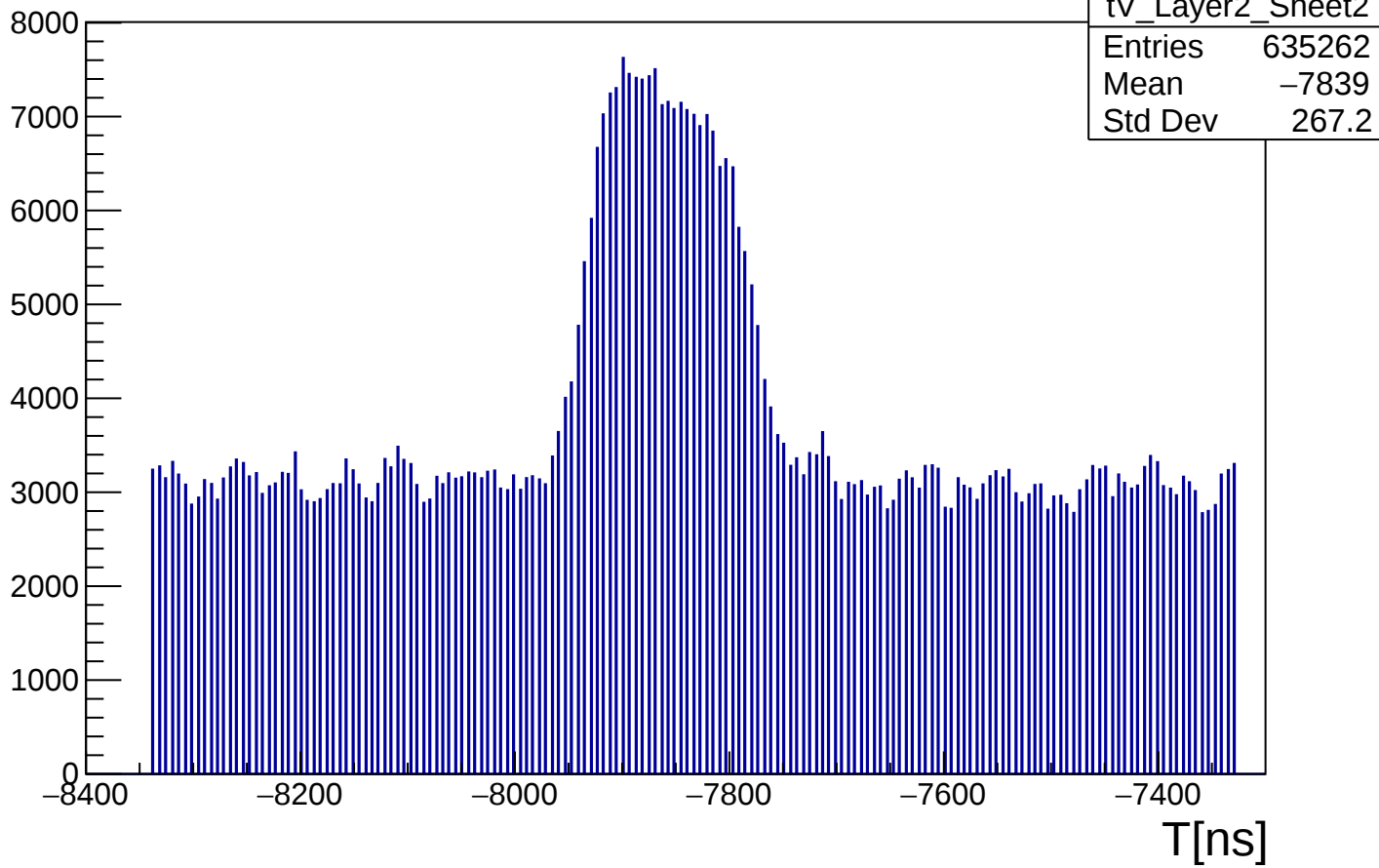
distribution of T, V strip, Layer2, top
