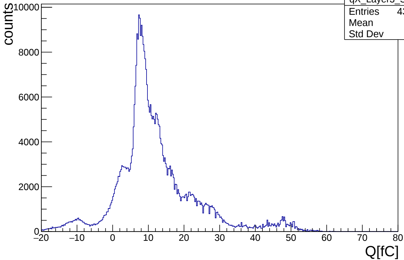
distribution of Q, X strip, Layer3, top
