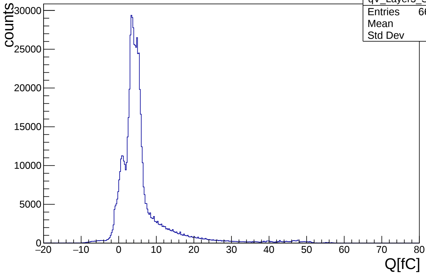
distribution of Q, V strip, Layer3, top
