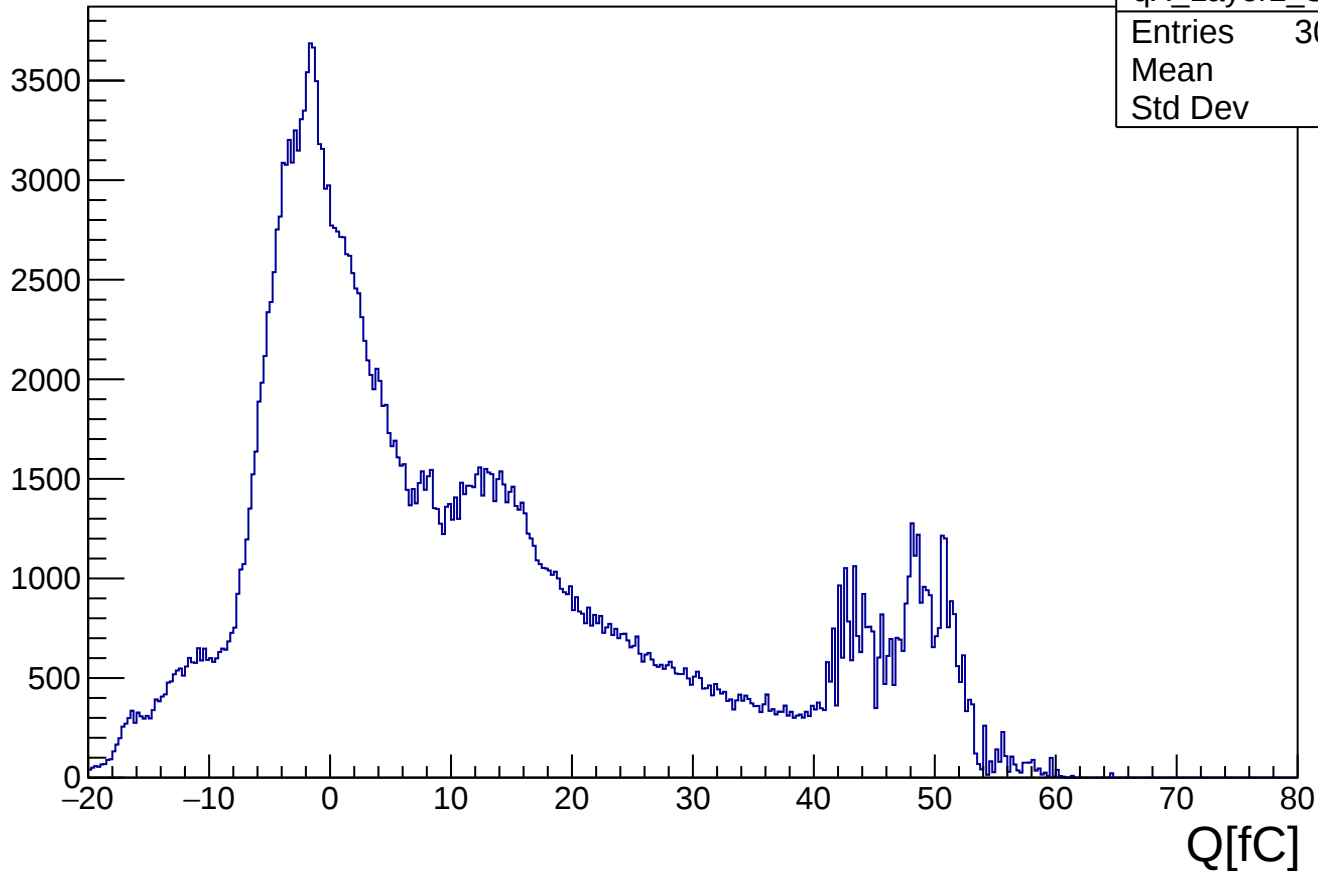
distribution of Q, X strip, Layer2, top
