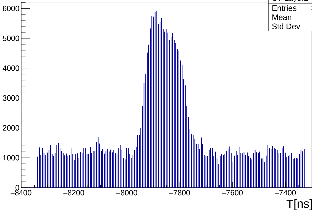
distribution of T, X strip, Layer2, top
