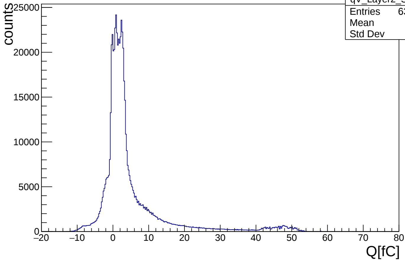
distribution of Q, V strip, Layer2, top
