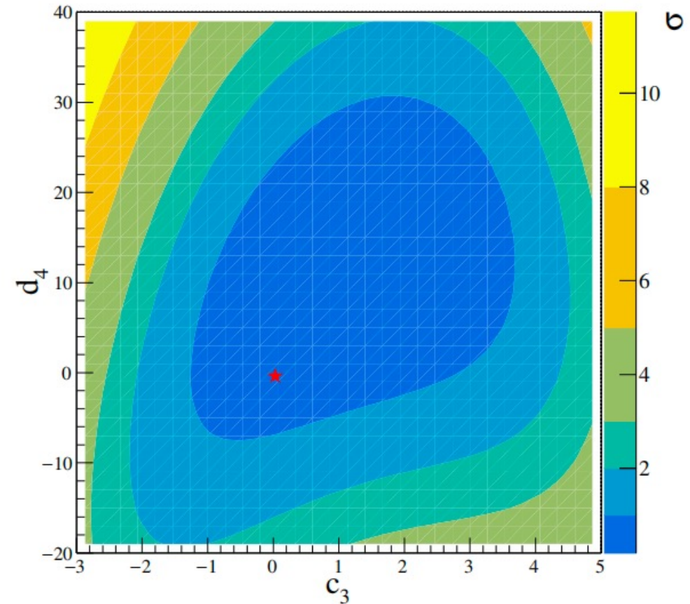
BDT
