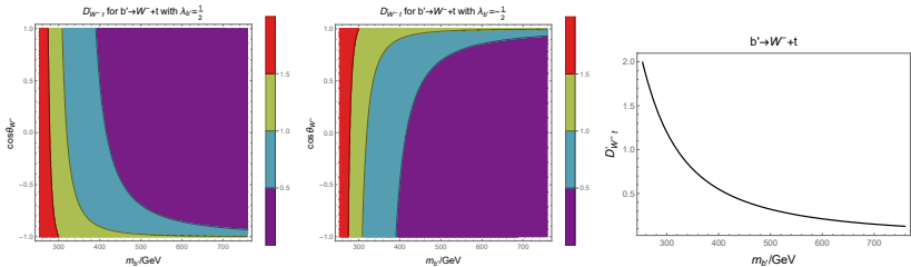
Figure: Left and middle: The LO predictions of D'_{W^-t} = \langle \cos \theta_{e-W^+} \rangle / 0.0658 for the W^-t pair produced by b' decay. Here, \theta_{W^-} represents the angle between the momentum direction of the W^- in the b' rest frame and the direction of b' motion in the laboratory frame. The symbols \lambda_{b'} denote the helicities of b' , defined along the momentum direction of b' in the laboratory frame. Right: The LO predictions of D'_{W^-t} = \langle \cos \theta_{e-W^+} \rangle / 0.0658 for the W^-t produced by b' decay, averaged over \cos \theta_{W^-} .
