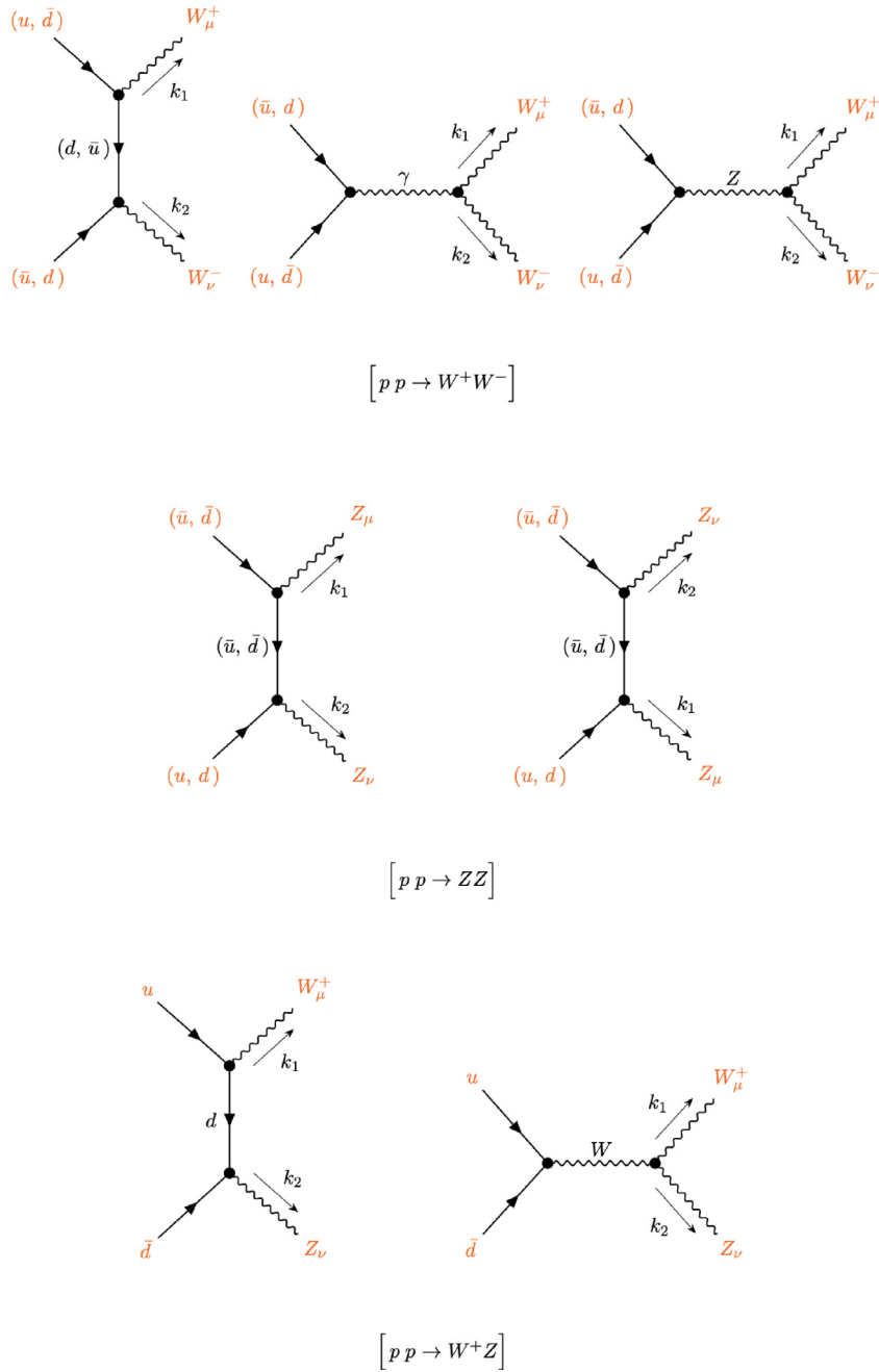
Fig. 5.1. Feynman diagrams for the processes p p \rightarrow W^+ W^- (first row), p p \rightarrow ZZ (second row) and p p \rightarrow W^+ Z (third row) at the parton level for the first quark generation. We neglect Diagrams mediated by the Higgs boson are neglected (in the limit of massless quarks). The arrows on the fermion lines indicate the momentum flow.
