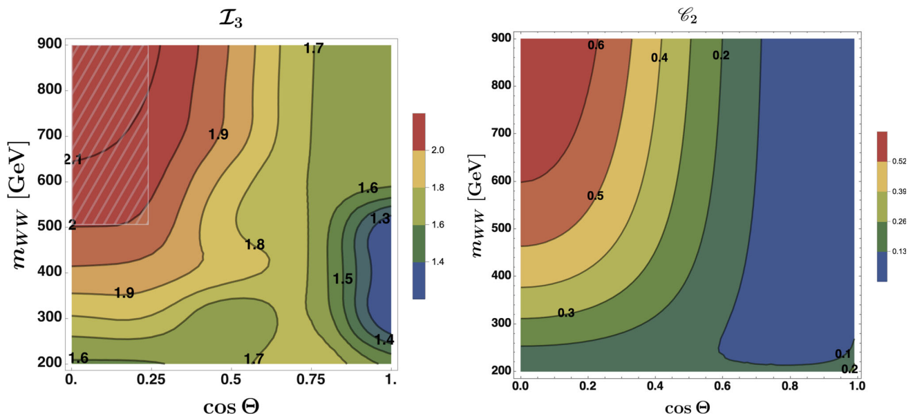
Fig. 11 The observables \mathcal{I}_3 (left plot) and \mathcal{C}_2 (right plot) for the process p p \rightarrow W^+ W^- as functions of the invariant mass and scattering angle. The hatched area in the plot on the left represents the bin used as reference for our estimate of the significance
