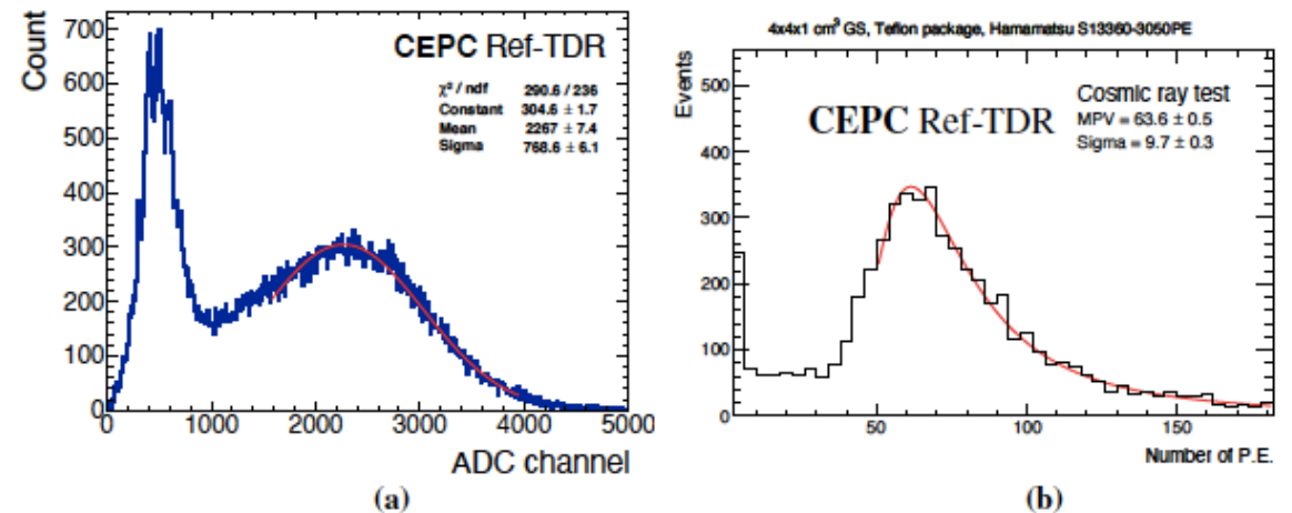
Figure 8.17: Measurement results of the GS cell with SiPM readout, the same GS cell size of 40 \times 40 \times 10 \text{ mm}^3 is used. (a) The measured ADC spectrum of GS cell with a SiPM (HPK S14160-3050HS) using ^{137}\text{Cs} radiation source. (b) Cosmic ray test results measured using HPK S13360-3050PE SiPM, resulting a light output about of 64 p.e./MIP.
