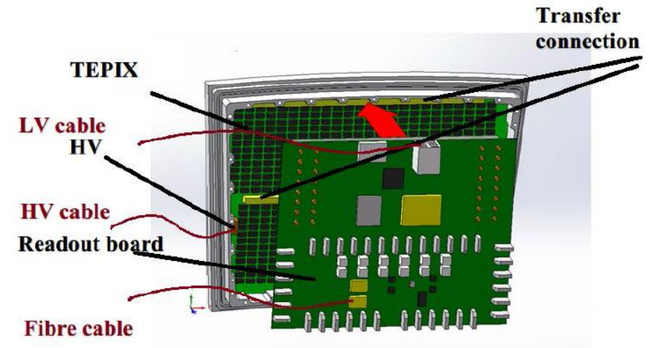
Figure 6.7: Design of the TPC endplate readout modules. Each module is mainly composed of a double-mesh Micromegas detector with a pixelated readout anode, a readout ASIC chip array mounted on the back of the anode board (FEE), and a readout board connected to the FEE board.
